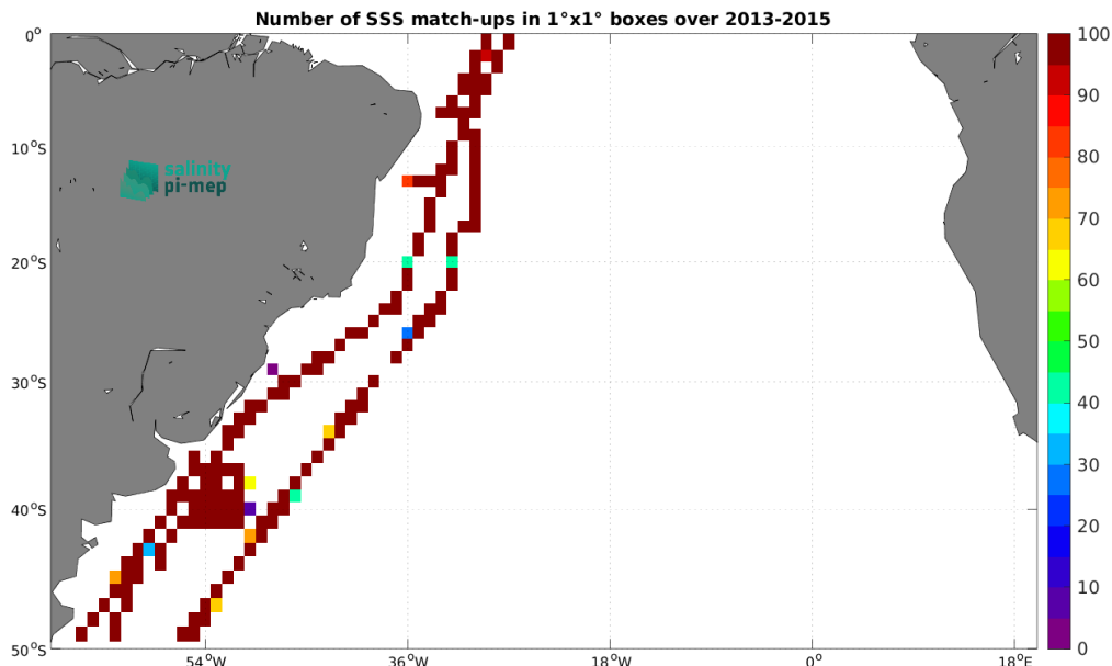
Figure 5: Number of SSS match-ups between TSG (CSIC-UTM) SSS and the Aquarius SSS L3 CAP v5 - 7-Day running (JPL) SSS product for the South Atlantic Ocean Pi-MEP region over 1^\circ \times 1^\circ boxes and for the full satellite product period.
