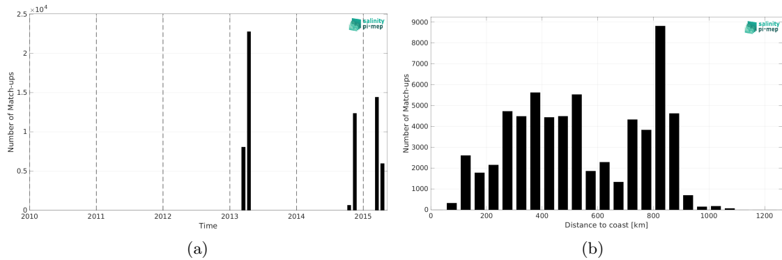
Figure 2: Number of match-ups between TSG (CSIC-UTM) and Aquarius SSS L3 CAP v5 - 7-Day running (JPL) SSS as a function of time (a) and as function of the distance to coast (b) over the South Atlantic Ocean Pi-MEP region and for the full satellite product period.
