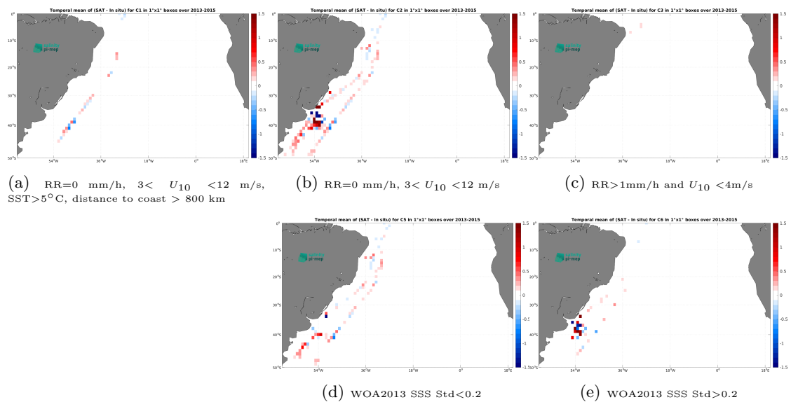
Figure 14: Temporal mean gridded over spatial boxes of size 1^\circ \times 1^\circ of \Delta\text{SSS} (Aquarius SSS L3 CAP v5 - 7-Day running (JPL) - TSG (CSIC-UTM)) for 5 different subdatasets corresponding to:RR=0 mm/h, 3 < U_{10} < 12 m/s, SST >5^\circ\text{C} , distance to coast > 800 km (a), RR=0 mm/h, 3 < U_{10} < 12 m/s (b), RR >1 mm/h and U_{10} < 4 m/s (c), WOA2013 SSS Std <0.2 (d), WOA2013 SSS Std >0.2 (e).
