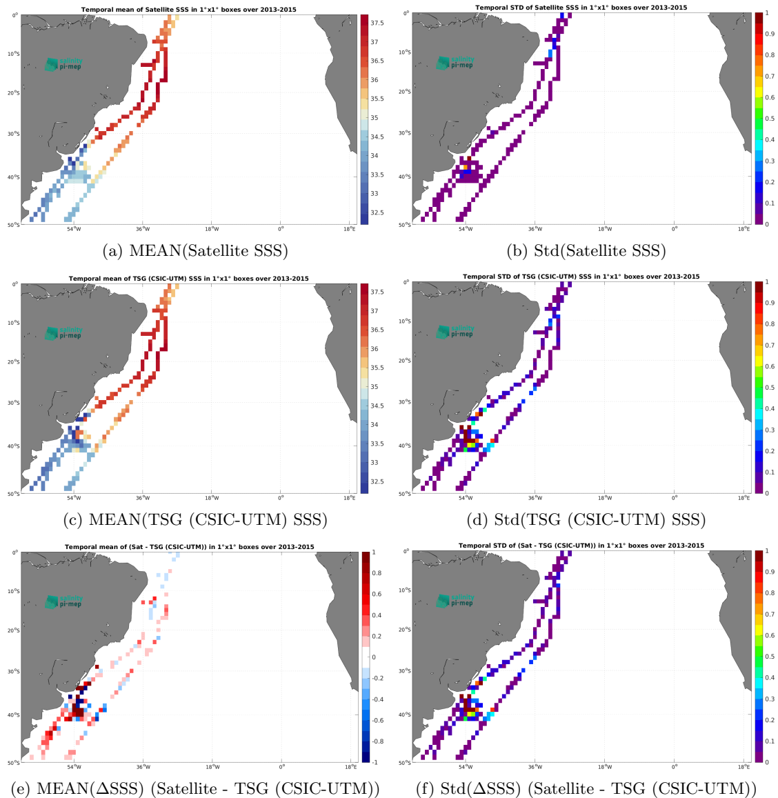
Figure 7: Temporal mean (left) and Std (right) of SSS from Aquarius SSS L3 CAP v5 - 7-Day running (JPL) (top), TSG (CSIC-UTM) (middle), and of \Delta SSS (Satellite - TSG (CSIC-UTM)). Only match-up pairs are used to generate these maps.
