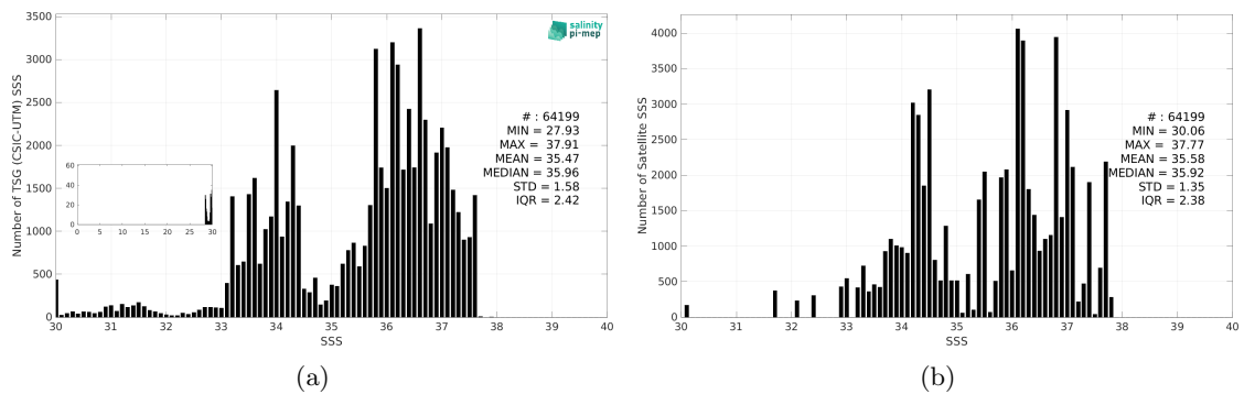
Figure 3: Histograms of SSS from TSG (CSIC-UTM) (a) and Aquarius SSS L3 CAP v5 - 7-Day running (JPL) (b) considering all match-up pairs per bins of 0.1 over the South Atlantic Ocean Pi-MEP region and for the full satellite product period.
