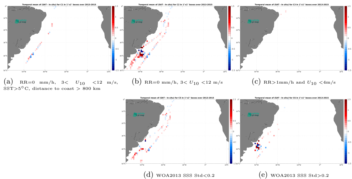
Figure 14: Temporal mean gridded over spatial boxes of size 1^\circ \times 1^\circ of \Delta\text{SSS} (Aquarius SSS L3 CAP v5 - 7-Day running (JPL) - TSG (CSIC-UTM)) for 5 different subdatasets corresponding to:RR=0 mm/h, 3 < U_{10} < 12 m/s, SST >5^\circ\text{C} , distance to coast > 800 km (a), RR=0 mm/h, 3 < U_{10} < 12 m/s (b), RR >1 mm/h and U_{10} < 4 m/s (c), WOA2013 SSS Std <0.2 (d), WOA2013 SSS Std >0.2 (e).
