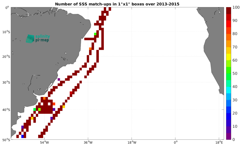
Figure 4: Number of SSS match-ups between TSG (CSIC-UTM) SSS and the Aquarius SSS L3 CAP v5 - 7-Day running (JPL) SSS product for the South Atlantic Ocean Pi-MEP region over 1^\circ \times 1^\circ boxes and for the full satellite product period.
