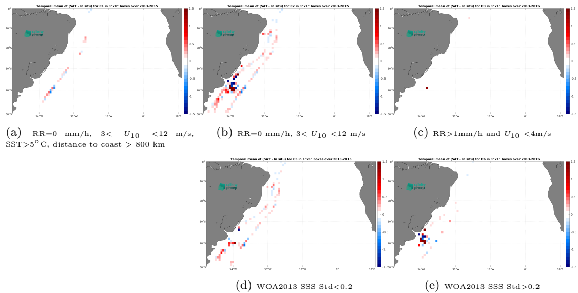
Figure 12: Temporal mean gridded over spatial boxes of size 1^\circ \times 1^\circ of \Delta\text{SSS} (Aquarius SSS L3 CAP v5 - 7-Day running (JPL) - TSG (CSIC-UTM)) for 5 different subdatasets corresponding to:RR=0 mm/h, 3 < U_{10} < 12 m/s, SST >5^\circ\text{C} , distance to coast > 800 km (a), RR=0 mm/h, 3 < U_{10} < 12 m/s (b), RR >1 mm/h and U_{10} < 4 m/s (c), WOA2013 SSS Std <0.2 (d), WOA2013 SSS Std >0.2 (e).
