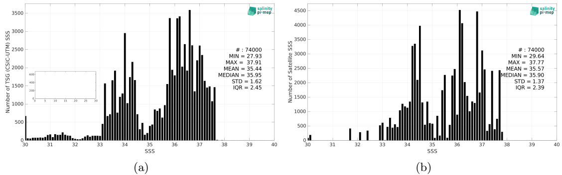
Figure 2: Histograms of SSS from TSG (CSIC-UTM) (a) and Aquarius SSS L3 CAP v5 - 7-Day running (JPL) (b) considering all match-up pairs per bins of 0.1 over the South Atlantic Ocean Pi-MEP region and for the full satellite product period.
