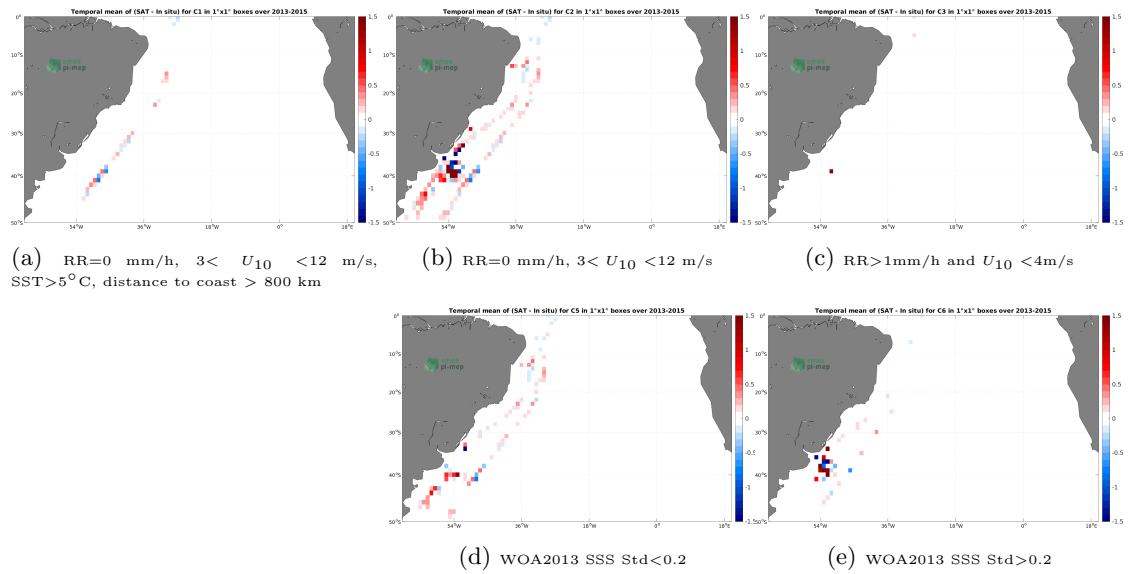
Figure 12: Temporal mean gridded over spatial boxes of size 1^\circ \times 1^\circ of \Delta SSS (Aquarius SSS L3 CAP v5 - 7-Day running (JPL) - TSG (CSIC-UTM)) for 5 different subdatasets corresponding to:RR=0 mm/h, 3 < U_{10} < 12 m/s, SST >5^\circ\text{C} , distance to coast > 800 km (a), RR=0 mm/h, 3 < U_{10} < 12 m/s (b), RR >1 mm/h and U_{10} < 4 m/s (c), WOA2013 SSS Std <0.2 (d), WOA2013 SSS Std >0.2 (e).
