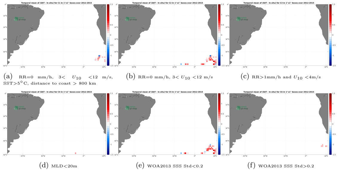
Figure 12: Temporal mean gridded over spatial boxes of size 1^{\circ}\times 1^{\circ} of \Delta\text{SSS} (Aquarius SSS L3 CAP v5 - 7-Day running (JPL) - Marine mammals) for 6 different subdatasets corresponding to:RR=0 mm/h, 3 < U_{10} < 12 m/s, SST >5^{\circ}\text{C} , distance to coast > 800 km (a), RR=0 mm/h, 3 < U_{10} < 12 m/s (b), RR >1\text{mm/h} and U_{10} < 4\text{m/s} (c),MLD <20\text{m} (d),WOA2013 SSS Std <0.2 (e),WOA2013 SSS Std >0.2 (f).
