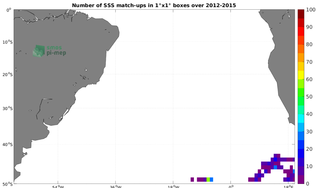
Figure 4: Number of SSS match-ups between Marine mammals SSS and the Aquarius SSS L3 CAP v5 - 7-Day running (JPL) SSS product for the South Atlantic Ocean Pi-MEP region over 1^\circ \times 1^\circ boxes and for the full satellite product period.
