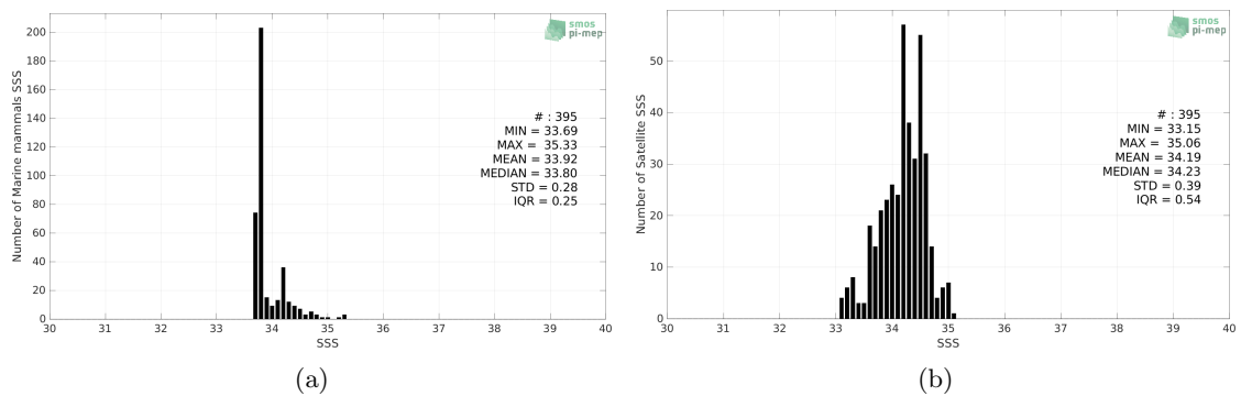
Figure 2: Histograms of SSS from Marine mammals (a) and Aquarius SSS L3 CAP v5 - 7-Day running (JPL) (b) considering all match-up pairs per bins of 0.1 over the South Atlantic Ocean Pi-MEP region and for the full satellite product period.
