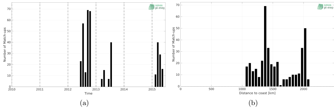
Figure 1: Number of match-ups between Marine mammals and Aquarius SSS L3 CAP v5 - 7-Day running (JPL) SSS as a function of time (a) and as function of the distance to coast (b) over the South Atlantic Ocean Pi-MEP region and for the full satellite product period.
