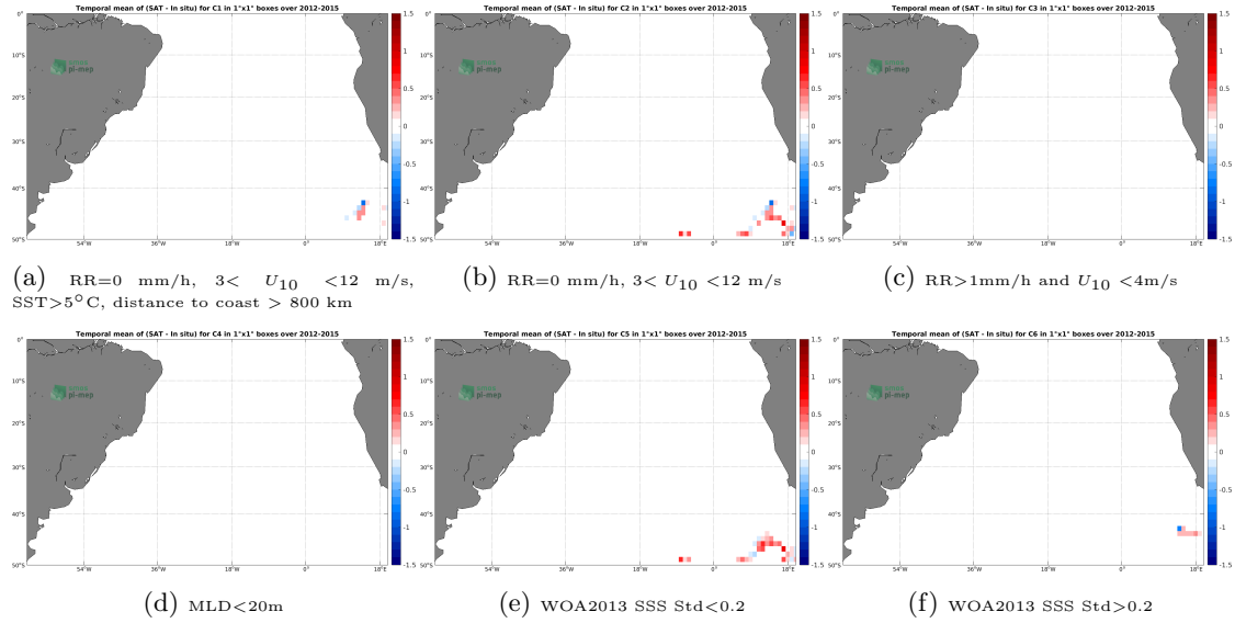
Figure 12: Temporal mean gridded over spatial boxes of size 1^{\circ}\times 1^{\circ} of \Delta\text{SSS} (Aquarius SSS L3 CAP v5 - 7-Day running (JPL) - Sea mammals) for 6 different subdatasets corresponding to: RR=0 mm/h, 3 < U_{10} < 12 m/s, SST > 5^{\circ}\text{C} , distance to coast > 800 km (a), RR=0 mm/h, 3 < U_{10} < 12 m/s (b), RR > 1 mm/h and U_{10} < 4 m/s (c), MLD < 20\text{m} (d), WOA2013 SSS Std < 0.2 (e), WOA2013 SSS Std > 0.2 (f).
