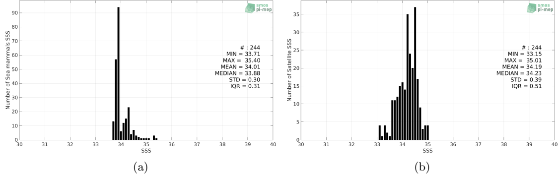
Figure 2: Histograms of SSS from Sea mammals (a) and Aquarius SSS L3 CAP v5 - 7-Day running (JPL) (b) considering all match-up pairs per bins of 0.1 over the South Atlantic Ocean Pi-MEP region and for the full satellite product period.
