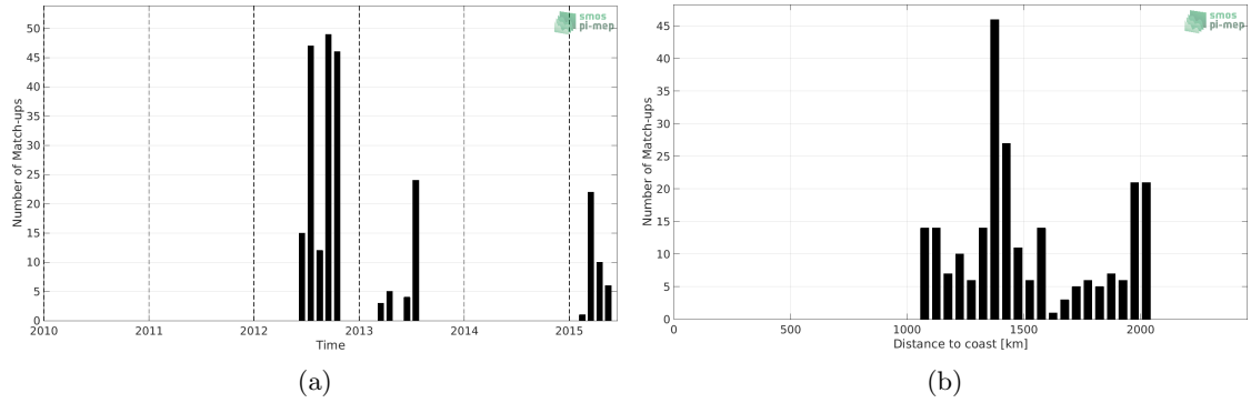
Figure 1: Number of match-ups between Sea mammals and Aquarius SSS L3 CAP v5 - 7-Day running (JPL) SSS as a function of time (a) and as function of the distance to coast (b) over the South Atlantic Ocean Pi-MEP region and for the full satellite product period.
