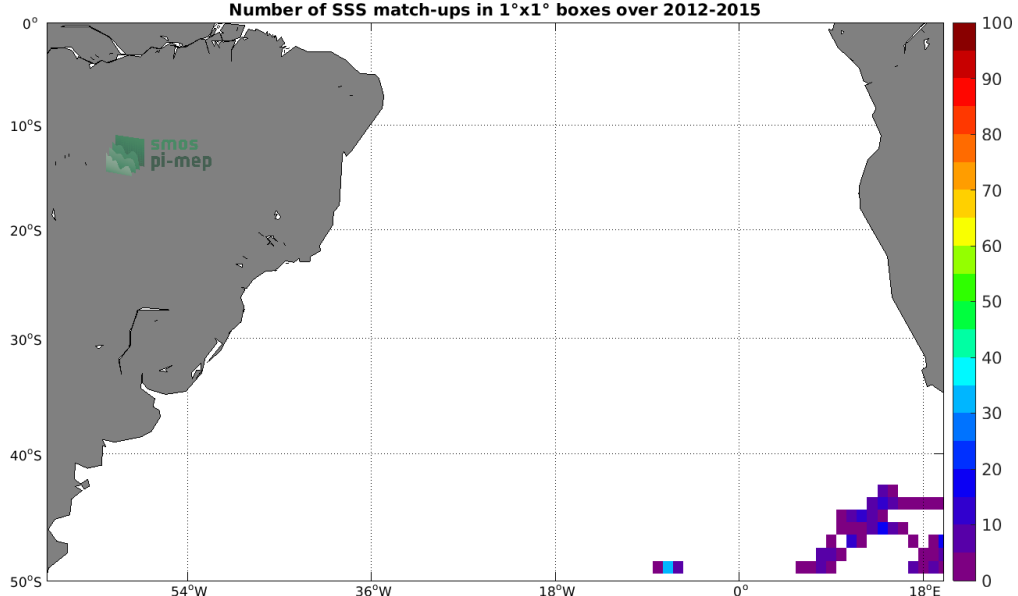
Figure 4: Number of SSS match-ups between Sea mammals SSS and the Aquarius SSS L3 CAP v5 - 7-Day running (JPL) SSS product for the South Atlantic Ocean Pi-MEP region over 1^\circ \times 1^\circ boxes and for the full satellite product period.
