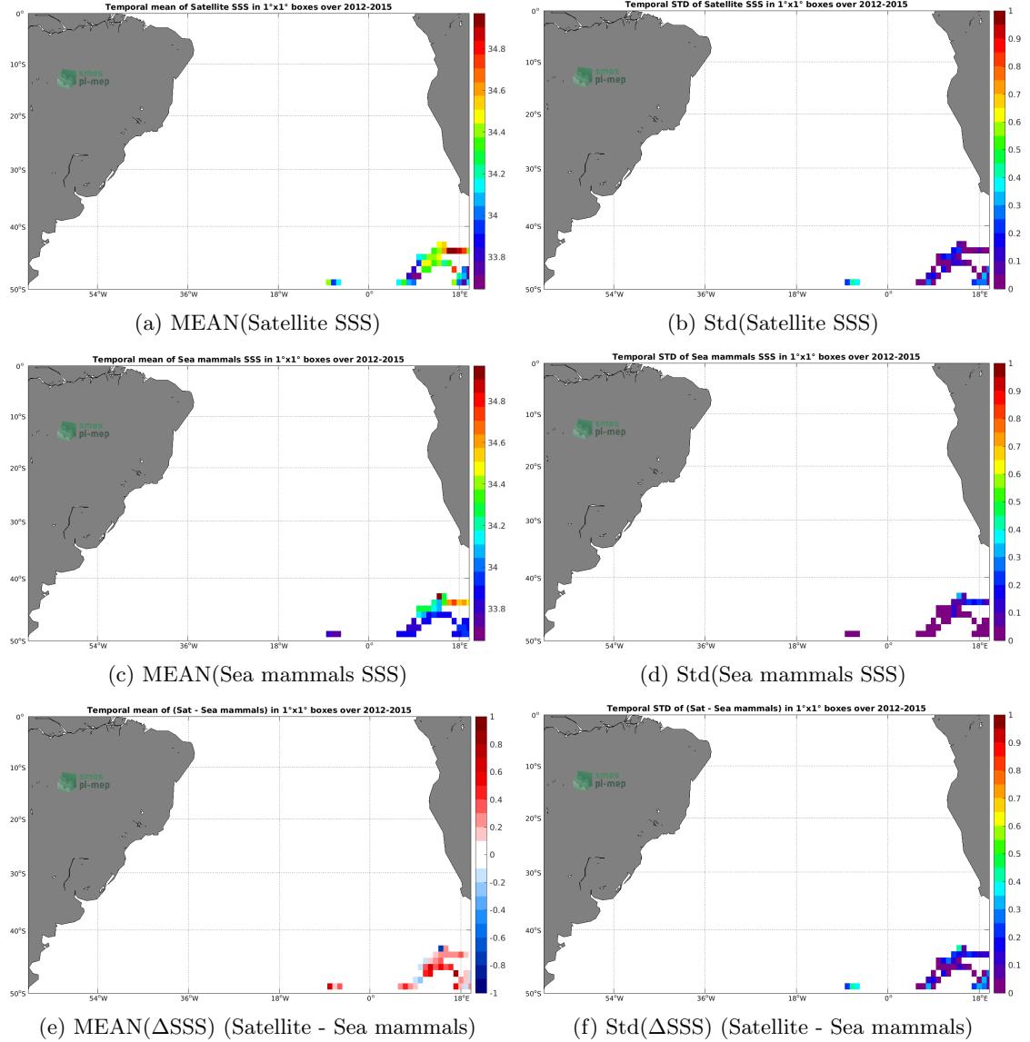
Figure 6: Temporal mean (left) and Std (right) of SSS from Aquarius SSS L3 CAP v5 - 7-Day running (JPL) (top), Sea mammals (middle), and of \Delta SSS (Satellite - Sea mammals). Only match-up pairs are used to generate these maps.
