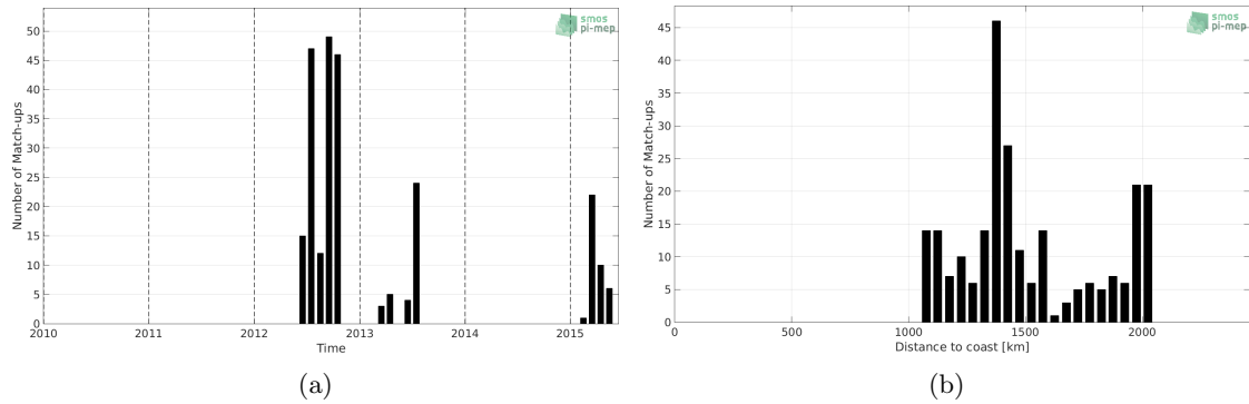
Figure 1: Number of match-ups between Sea mammals and Aquarius-L3-JPL-V5-7DAY-RUNNING SSS as a function of time (a) and as function of the distance to coast (b) over the South Atlantic Ocean Pi-MEP region and for the full satellite product period.
