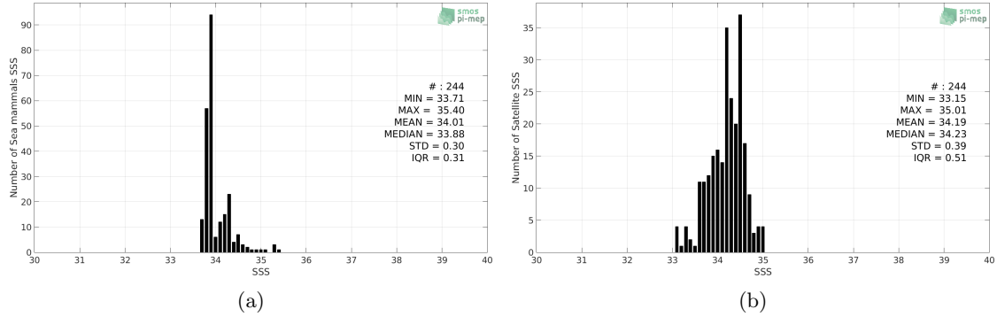
Figure 2: Histograms of SSS from Sea mammals (a) and Aquarius-L3-JPL-V5-7DAY-RUNNING (b) considering all match-up pairs per bins of 0.1 over the South Atlantic Ocean Pi-MEP region and for the full satellite product period.
