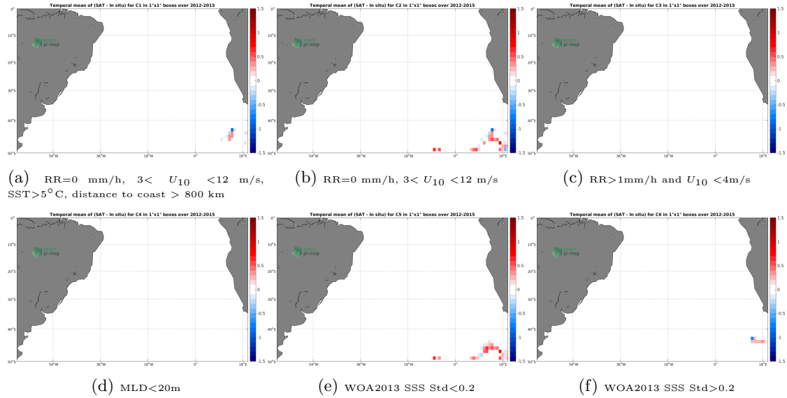
Figure 12: Temporal mean gridded over spatial boxes of size 1^{\circ}\times 1^{\circ} of \Delta\text{SSS} (Aquarius-L3-JPL-V5-7DAY-RUNNING - Sea mammals) for 6 different subdatasets corresponding to: RR=0 mm/h, 3 < U_{10} < 12 m/s, SST > 5^{\circ}\text{C} , distance to coast > 800 km (a), RR=0 mm/h, 3 < U_{10} < 12 m/s (b), RR > 1 mm/h and U_{10} < 4 m/s (c), MLD < 20 m (d), WOA2013 SSS Std < 0.2 (e), WOA2013 SSS Std > 0.2 (f).
