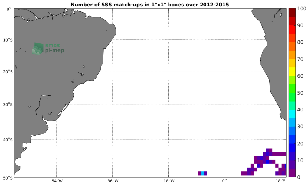
Figure 4: Number of SSS match-ups between Sea mammals SSS and the Aquarius-L3-JPL-V5-7DAY-RUNNING SSS product for the South Atlantic Ocean Pi-MEP region over 1^\circ \times 1^\circ boxes and for the full satellite product period.
