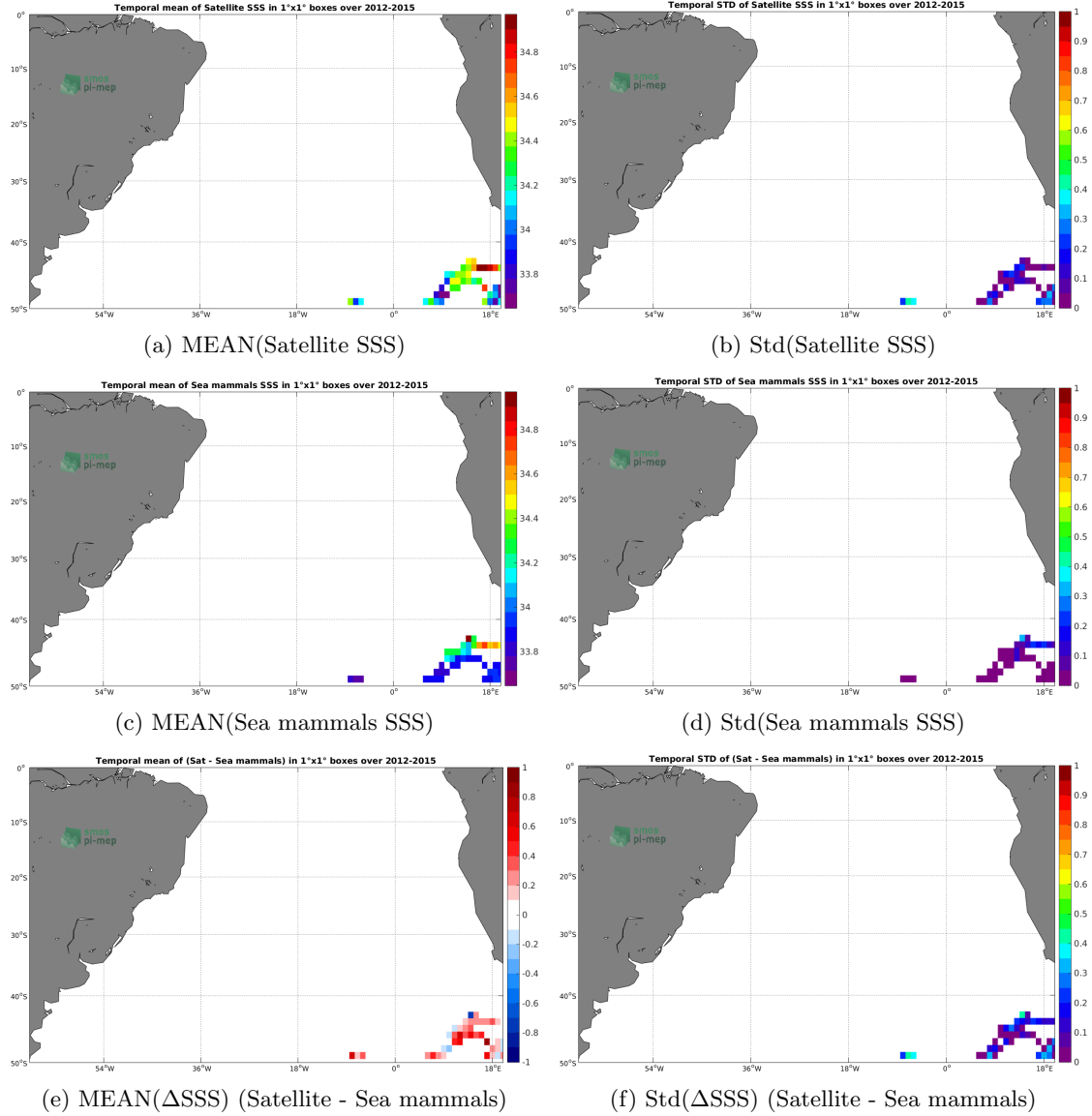
Figure 6: Temporal mean (left) and Std (right) of SSS from Aquarius-L3-JPL-V5-7DAY-RUNNING (top), Sea mammals (middle), and of \Delta SSS (Satellite - Sea mammals). Only match-up pairs are used to generate these maps.
