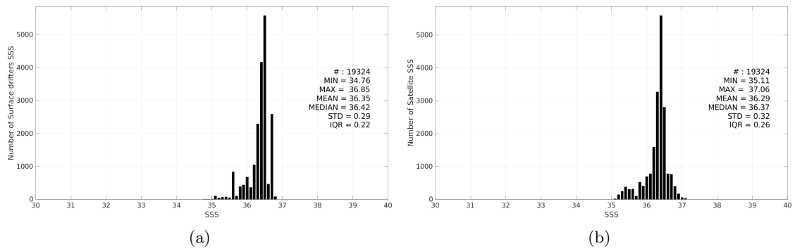
Figure 3: Histograms of SSS from Surface drifters (a) and Aquarius SSS L3 CAP v5 - 7-Day running (JPL) (b) considering all match-up pairs per bins of 0.1 over the South Atlantic Ocean Pi-MEP region and for the full satellite product period.
