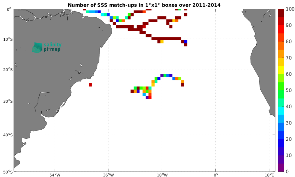
Figure 4: Number of SSS match-ups between Surface drifters SSS and the Aquarius SSS L3 CAP v5 - 7-Day running (JPL) SSS product for the South Atlantic Ocean Pi-MEP region over 1^\circ \times 1^\circ boxes and for the full satellite product period.
