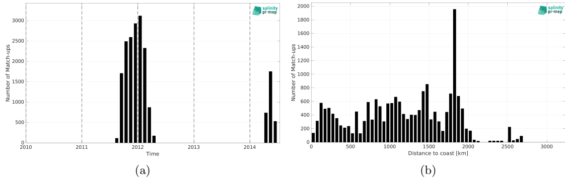
Figure 2: Number of match-ups between Surface drifters and Aquarius SSS L3 CAP v5 - 7-Day running (JPL) SSS as a function of time (a) and as function of the distance to coast (b) over the South Atlantic Ocean Pi-MEP region and for the full satellite product period.
