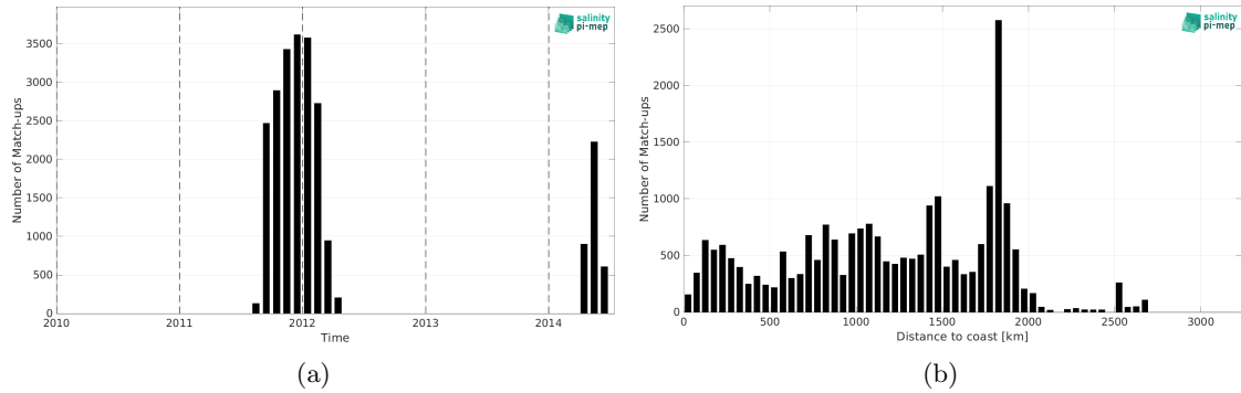
Figure 1: Number of match-ups between Surface drifters and Aquarius SSS L3 CAP v5 - 7-Day running (JPL) SSS as a function of time (a) and as function of the distance to coast (b) over the South Atlantic Ocean Pi-MEP region and for the full satellite product period.
