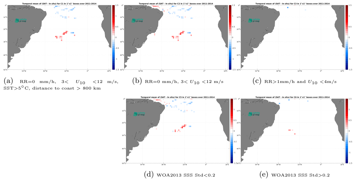
Figure 11: Temporal mean gridded over spatial boxes of size 1^\circ \times 1^\circ of \Delta\text{SSS} (Aquarius SSS L3 CAP v5 - 7-Day running (JPL) - Surface drifters) for 5 different subdatasets corresponding to:RR=0 mm/h, 3 < U_{10} < 12 m/s, SST >5^\circ\text{C} , distance to coast > 800 km (a), RR=0 mm/h, 3 < U_{10} < 12 m/s (b), RR >1 mm/h and U_{10} < 4 m/s (c), WOA2013 SSS Std <0.2 (d), WOA2013 SSS Std >0.2 (e).
