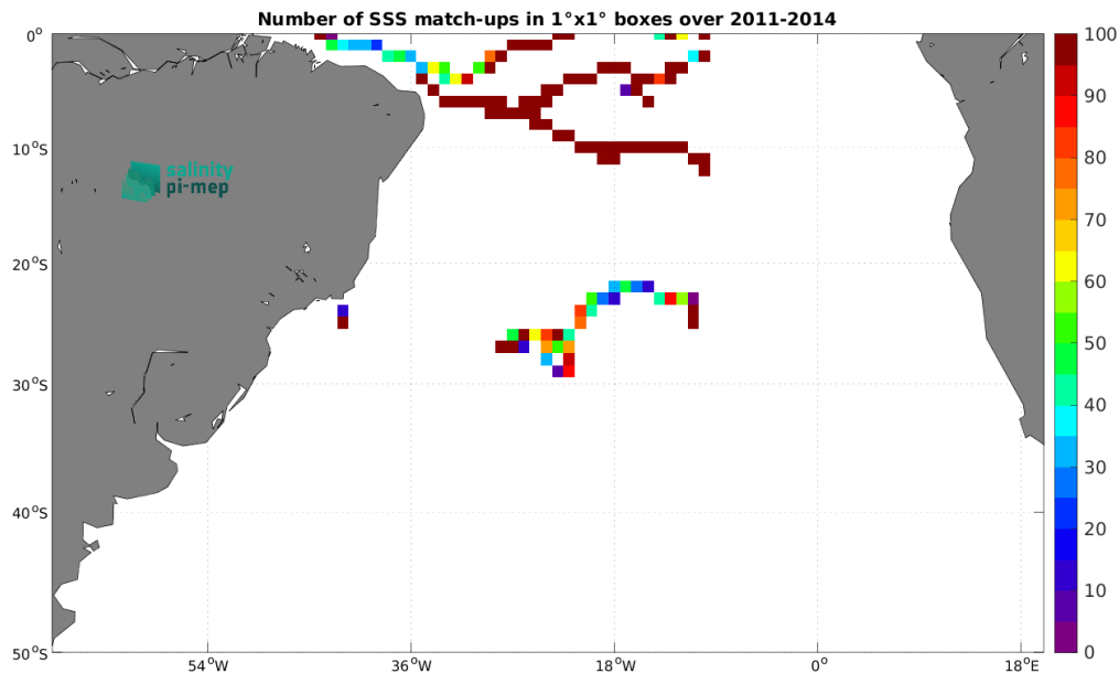
Figure 3: Number of SSS match-ups between Surface drifters SSS and the Aquarius SSS L3 CAP v5 - 7-Day running (JPL) SSS product for the South Atlantic Ocean Pi-MEP region over 1^\circ \times 1^\circ boxes and for the full satellite product period.
