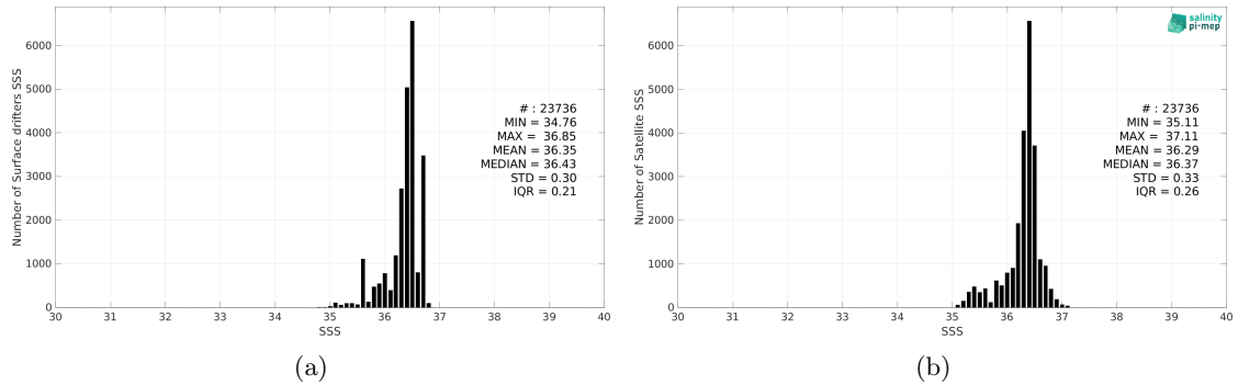
Figure 2: Histograms of SSS from Surface drifters (a) and Aquarius SSS L3 CAP v5 - 7-Day running (JPL) (b) considering all match-up pairs per bins of 0.1 over the South Atlantic Ocean Pi-MEP region and for the full satellite product period.
