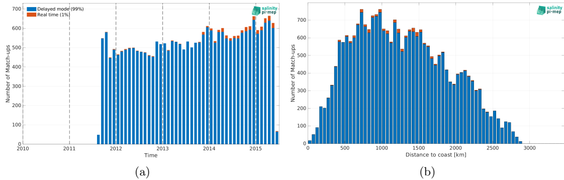
Figure 2: Number of match-ups between Argo and Aquarius SSS L3 CAP v5 - 7-Day running (JPL) SSS as a function of time (a) and as function of the distance to coast (b) over the South Atlantic Ocean Pi-MEP region and for the full satellite product period.
