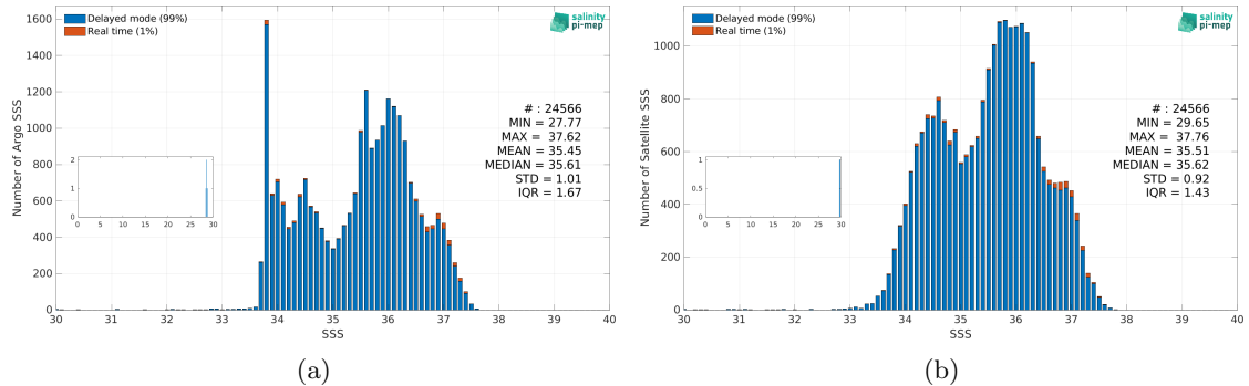
Figure 3: Histograms of SSS from Argo (a) and Aquarius SSS L3 CAP v5 - 7-Day running (JPL) (b) considering all match-up pairs per bins of 0.1 over the South Atlantic Ocean Pi-MEP region and for the full satellite product period.
