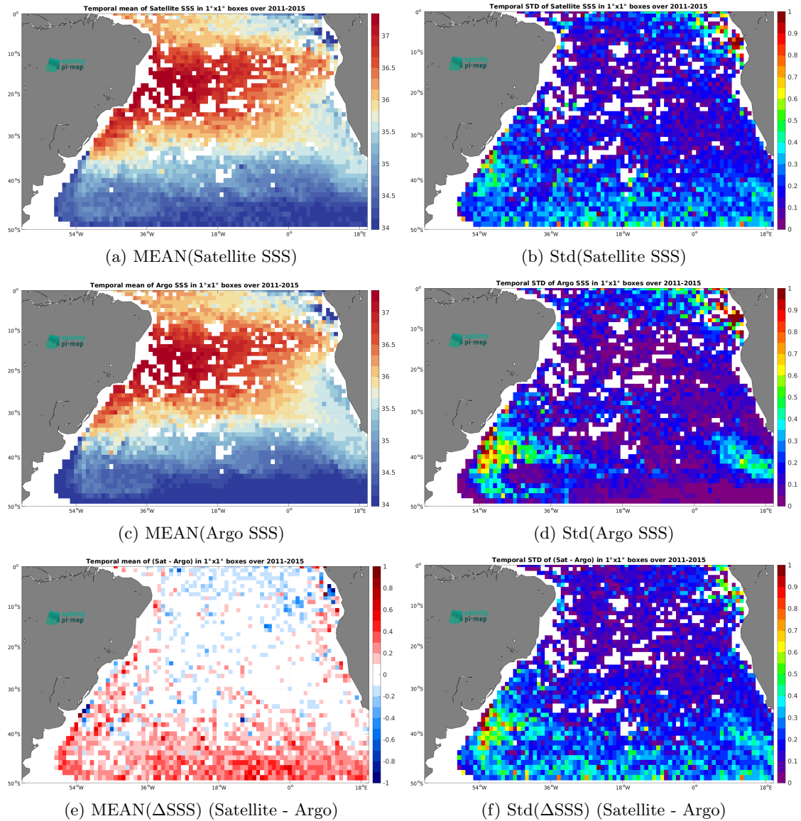
Figure 7: Temporal mean (left) and Std (right) of SSS from Aquarius SSS L3 CAP v5 - 7-Day running (JPL) (top), Argo (middle), and of \Delta SSS (Satellite - Argo). Only match-up pairs are used to generate these maps.
