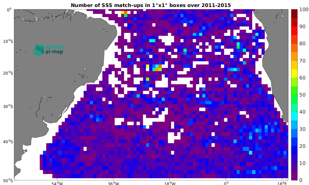
Figure 5: Number of SSS match-ups between Argo SSS and the Aquarius SSS L3 CAP v5 - 7-Day running (JPL) SSS product for the South Atlantic Ocean Pi-MEP region over 1^\circ \times 1^\circ boxes and for the full satellite product period.
