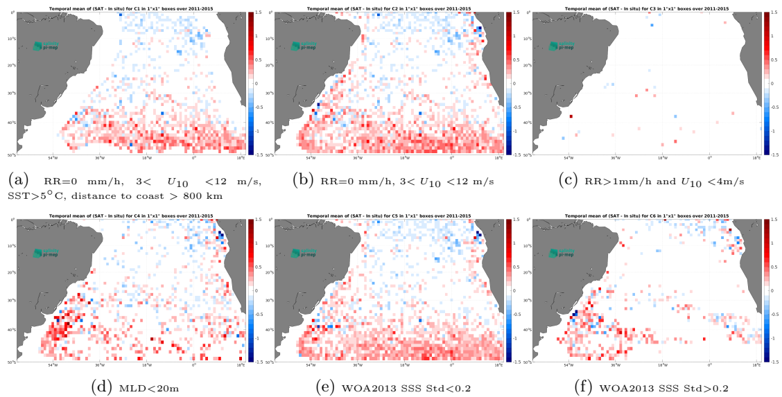
Figure 14: Temporal mean gridded over spatial boxes of size 1^\circ \times 1^\circ of \Delta SSS (Aquarius SSS L3 CAP v5 - 7-Day running (JPL) - Argo) for 6 different subdatasets corresponding to:RR=0 mm/h, 3 < U_{10} < 12 m/s, SST >5^\circ C, distance to coast > 800 km (a), RR=0 mm/h, 3 < U_{10} < 12 m/s (b), RR >1 mm/h and U_{10} < 4 m/s (c),MLD <20 m (d),WOA2013 SSS Std <0.2 (e),WOA2013 SSS Std >0.2 (f).
