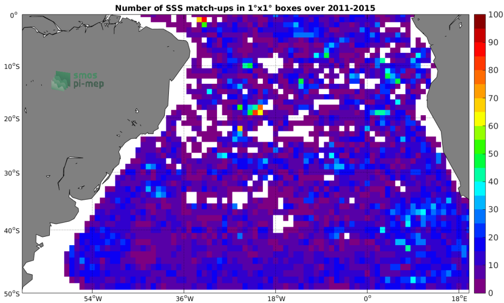
Figure 4: Number of SSS match-ups between Argo SSS and the Aquarius-L3-JPL-V5-7DAY-RUNNING SSS product for the South Atlantic Ocean Pi-MEP region over 1^{\circ} \times 1^{\circ} boxes and for the full satellite product period.
