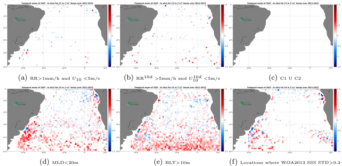
Figure 12: Temporal mean gridded over spatial boxes of size 1^\circ \times 1^\circ of \Delta\text{SSS} (Aquarius-L3-JPL-V5-7DAY-RUNNING - Argo) for 6 different subdatasets corresponding to: \text{RR} > 1\text{mm/h} and U_{10} < 5\text{m/s} (a), \text{RR}^{10d} > 5\text{mm/h} and U_{10}^{10d} < 5\text{m/s} (b), C1 U C2 (c), \text{MLD} < 20\text{m} (d), \text{BLT} > 10\text{m} (e), Locations where WOA2013 SSS STD > 0.2 (f).
