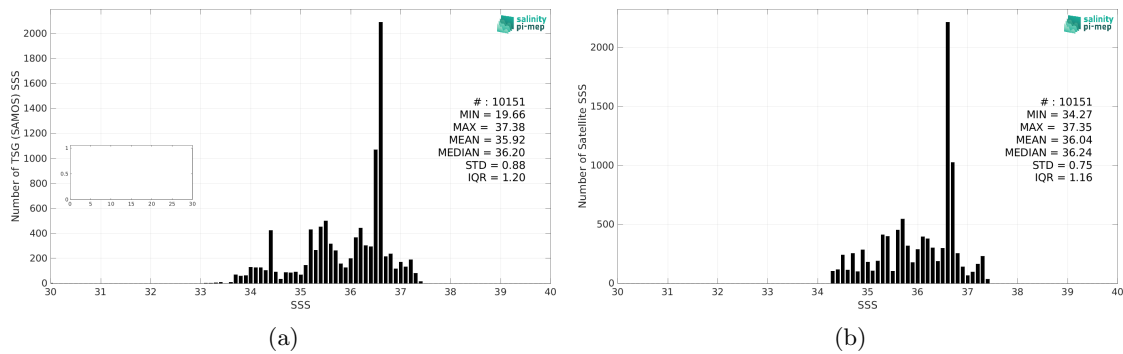
Figure 2: Histograms of SSS from TSG (SAMOS) (a) and Aquarius SSS L3 CAP v5 - Monthly (JPL) (b) considering all match-up pairs per bins of 0.1 over the South Atlantic Ocean Pi-MEP region and for the full satellite product period.
