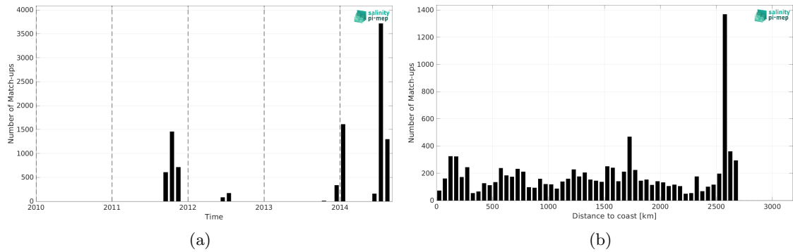
Figure 1: Number of match-ups between TSG (SAMOS) and Aquarius SSS L3 CAP v5 - Monthly (JPL) SSS as a function of time (a) and as function of the distance to coast (b) over the South Atlantic Ocean Pi-MEP region and for the full satellite product period.
