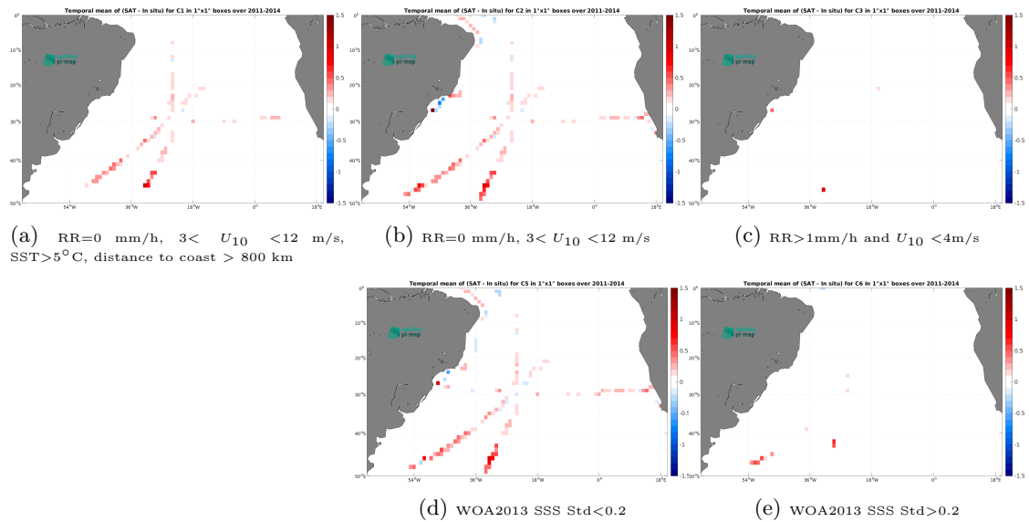
Figure 12: Temporal mean gridded over spatial boxes of size 1^\circ \times 1^\circ of \Delta\text{SSS} (Aquarius SSS L3 CAP v5 - Monthly (JPL) - TSG (SAMOS)) for 5 different subdatasets corresponding to:RR=0 mm/h, 3 < U_{10} < 12 m/s, SST >5^\circ\text{C} , distance to coast > 800 km (a), RR=0 mm/h, 3 < U_{10} < 12 m/s (b), RR >1 mm/h and U_{10} < 4 m/s (c), WOA2013 SSS Std <0.2 (d), WOA2013 SSS Std >0.2 (e).
