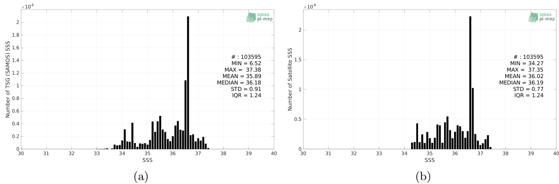
Figure 2: Histograms of SSS from TSG (SAMOS) (a) and Aquarius SSS L3 CAP v5 - Monthly (JPL) (b) considering all match-up pairs per bins of 0.1 over the South Atlantic Ocean Pi-MEP region and for the full satellite product period.
