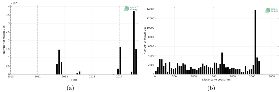
Figure 1: Number of match-ups between TSG (SAMOS) and Aquarius SSS L3 CAP v5 - Monthly (JPL) SSS as a function of time (a) and as function of the distance to coast (b) over the South Atlantic Ocean Pi-MEP region and for the full satellite product period.
