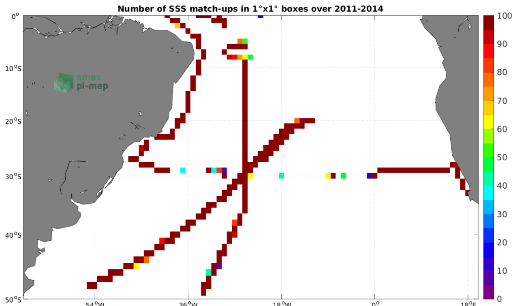
Figure 4: Number of SSS match-ups between TSG (SAMOS) SSS and the Aquarius SSS L3 CAP v5 - Monthly (JPL) SSS product for the South Atlantic Ocean Pi-MEP region over 1^\circ \times 1^\circ boxes and for the full satellite product period.
