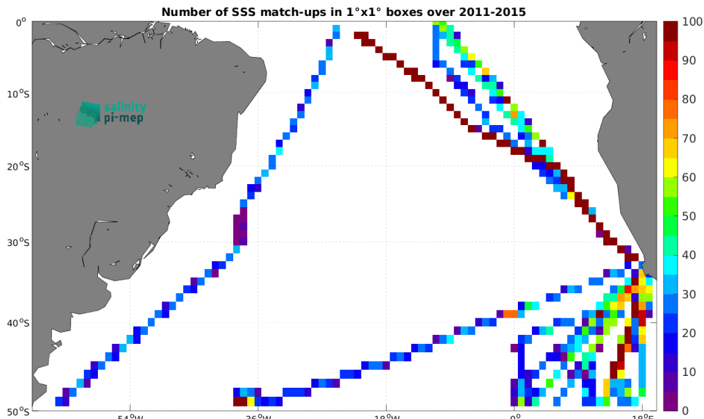
Figure 5: Number of SSS match-ups between TSG (Polarstern) SSS and the Aquarius SSS L3 CAP v5 - Monthly (JPL) SSS product for the South Atlantic Ocean Pi-MEP region over 1^\circ \times 1^\circ boxes and for the full satellite product period.
