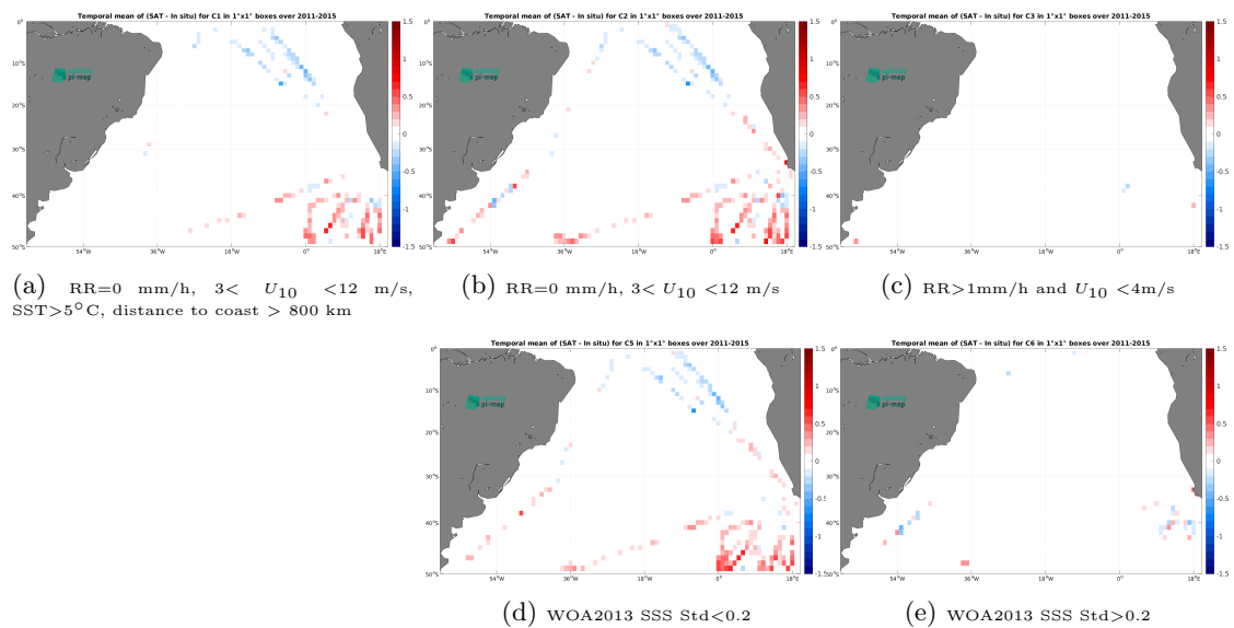
Figure 14: Temporal mean gridded over spatial boxes of size 1^\circ \times 1^\circ of \Delta\text{SSS} (Aquarius SSS L3 CAP v5 - Monthly (JPL) - TSG (Polarstern)) for 5 different subdatasets corresponding to:RR=0 mm/h, 3 < U_{10} < 12 m/s, SST > 5^\circ\text{C} , distance to coast > 800 km (a), RR=0 mm/h, 3 < U_{10} < 12 m/s (b), RR > 1 mm/h and U_{10} < 4 m/s (c), WOA2013 SSS Std < 0.2 (d), WOA2013 SSS Std > 0.2 (e).
