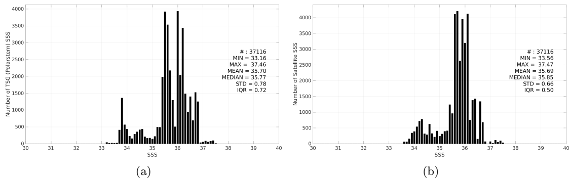
Figure 3: Histograms of SSS from TSG (Polarstern) (a) and Aquarius SSS L3 CAP v5 - Monthly (JPL) (b) considering all match-up pairs per bins of 0.1 over the South Atlantic Ocean Pi-MEP region and for the full satellite product period.
