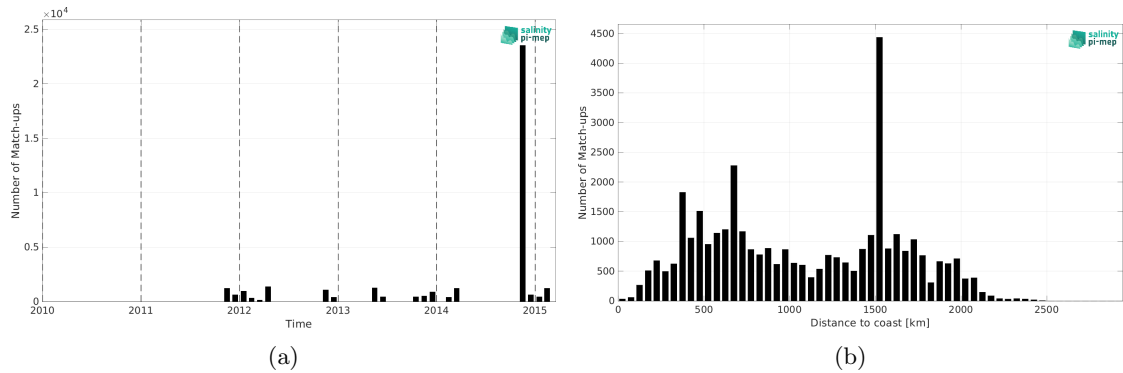
Figure 2: Number of match-ups between TSG (Polarstern) and Aquarius SSS L3 CAP v5 - Monthly (JPL) SSS as a function of time (a) and as function of the distance to coast (b) over the South Atlantic Ocean Pi-MEP region and for the full satellite product period.
