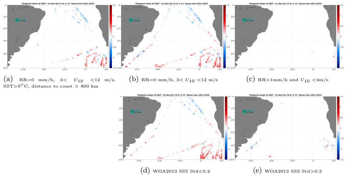
Figure 12: Temporal mean gridded over spatial boxes of size 1^\circ \times 1^\circ of \Delta\text{SSS} (Aquarius SSS L3 CAP v5 - Monthly (JPL) - TSG (Polarstern)) for 5 different subdatasets corresponding to:RR=0 mm/h, 3 < U_{10} < 12 m/s, SST >5^\circ\text{C} , distance to coast > 800 km (a), RR=0 mm/h, 3 < U_{10} < 12 m/s (b), RR >1 mm/h and U_{10} < 4 m/s (c), WOA2013 SSS Std <0.2 (d), WOA2013 SSS Std >0.2 (e).
