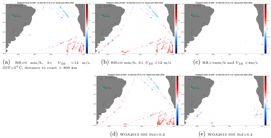
Figure 12: Temporal mean gridded over spatial boxes of size 1^\circ \times 1^\circ of \Delta SSS (Aquarius SSS L3 CAP v5 - Monthly (JPL) - TSG (Polarstern)) for 5 different subdatasets corresponding to:RR=0 mm/h, 3 < U_{10} < 12 m/s, SST >5^\circ\text{C} , distance to coast > 800 km (a), RR=0 mm/h, 3 < U_{10} < 12 m/s (b), RR >1 mm/h and U_{10} < 4 m/s (c), WOA2013 SSS Std <0.2 (d), WOA2013 SSS Std >0.2 (e).
