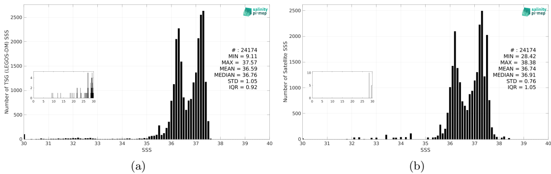
Figure 3: Histograms of SSS from TSG (LEGOS-DM) (a) and Aquarius SSS L3 CAP v5 - Monthly (JPL) (b) considering all match-up pairs per bins of 0.1 over the South Atlantic Ocean Pi-MEP region and for the full satellite product period.
