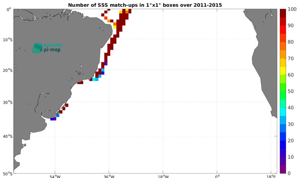
Figure 5: Number of SSS match-ups between TSG (LEGOS-DM) SSS and the Aquarius SSS L3 CAP v5 - Monthly (JPL) SSS product for the South Atlantic Ocean Pi-MEP region over 1^\circ \times 1^\circ boxes and for the full satellite product period.
