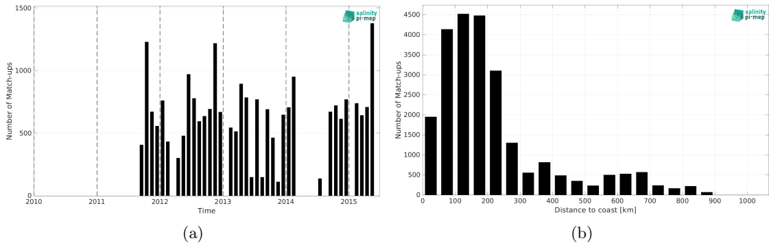
Figure 2: Number of match-ups between TSG (LEGOS-DM) and Aquarius SSS L3 CAP v5 - Monthly (JPL) SSS as a function of time (a) and as function of the distance to coast (b) over the South Atlantic Ocean Pi-MEP region and for the full satellite product period.
