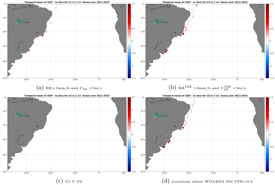
Figure 12: Temporal mean gridded over spatial boxes of size 1^\circ \times 1^\circ of \Delta SSS (Aquarius-L3-JPL-V5-MONTHLY - TSG-LEGOS-DM) for 4 different subdatasets corresponding to: RR > 1mm/h and U_{10} < 5\text{m/s} (a), RR^{10d} > 5\text{mm/h} and U_{10}^{10d} < 5\text{m/s} (b), C1 U C2 (c), Locations where WOA2013 SSS STD > 0.2 (d).
