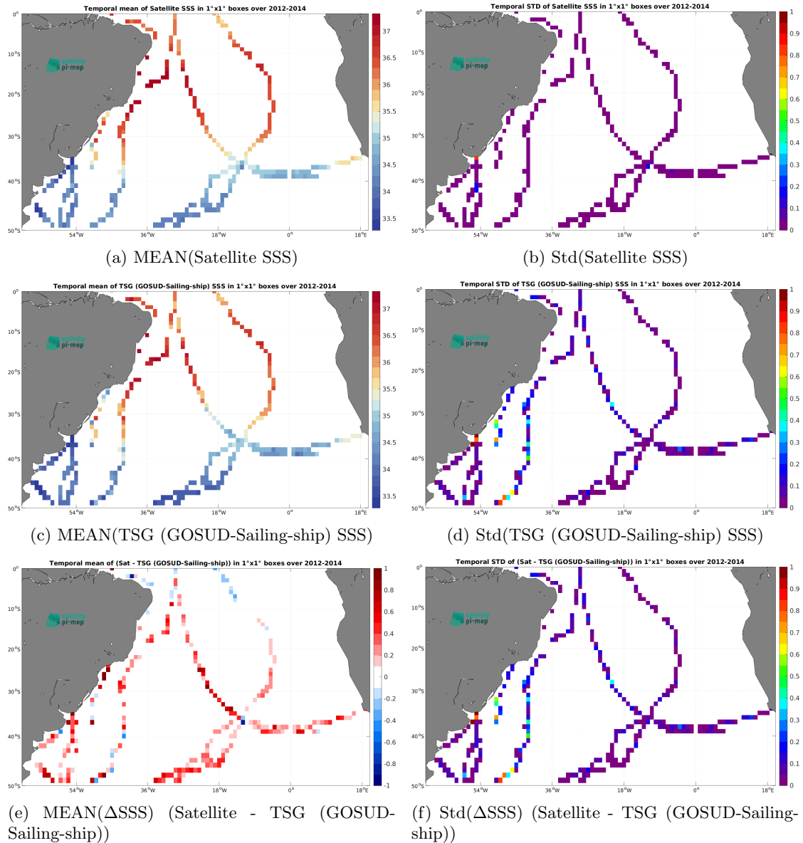
Figure 7: Temporal mean (left) and Std (right) of SSS from Aquarius SSS L3 CAP v5 - Monthly (JPL) (top), TSG (GOSUD-Sailing-ship) (middle), and of \Delta SSS (Satellite - TSG (GOSUD-Sailing-ship)). Only match-up pairs are used to generate these maps.
