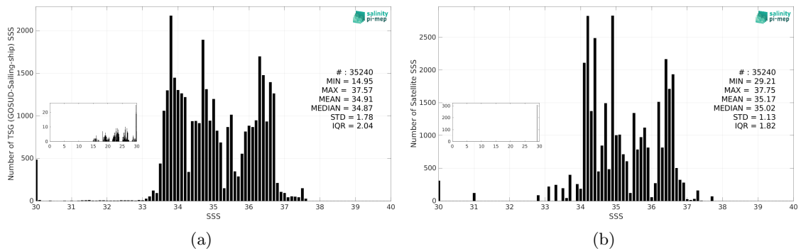
Figure 3: Histograms of SSS from TSG (GOSUD-Sailing-ship) (a) and Aquarius SSS L3 CAP v5 - Monthly (JPL) (b) considering all match-up pairs per bins of 0.1 over the South Atlantic Ocean Pi-MEP region and for the full satellite product period.
