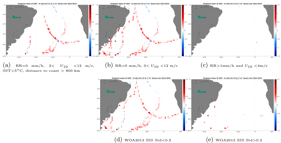
Figure 14: Temporal mean gridded over spatial boxes of size 1^\circ \times 1^\circ of \Delta\text{SSS} (Aquarius SSS L3 CAP v5 - Monthly (JPL) - TSG (GOSUD-Sailing-ship)) for 5 different subdatasets corresponding to:RR=0 mm/h, 3 < U_{10} < 12 m/s, SST >5^\circ\text{C} , distance to coast > 800 km (a), RR=0 mm/h, 3 < U_{10} < 12 m/s (b), RR >1 mm/h and U_{10} < 4 m/s (c), WOA2013 SSS Std <0.2 (d), WOA2013 SSS Std >0.2 (e).
