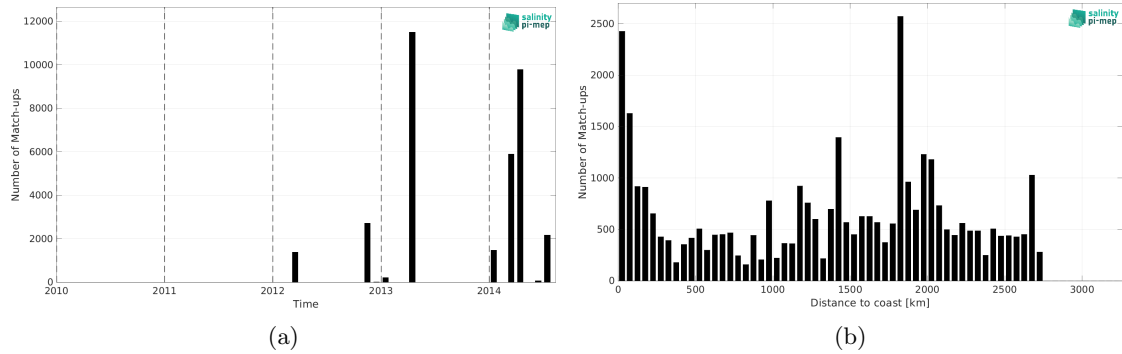
Figure 2: Number of match-ups between TSG (GOSUD-Sailing-ship) and Aquarius SSS L3 CAP v5 - Monthly (JPL) SSS as a function of time (a) and as function of the distance to coast (b) over the South Atlantic Ocean Pi-MEP region and for the full satellite product period.
