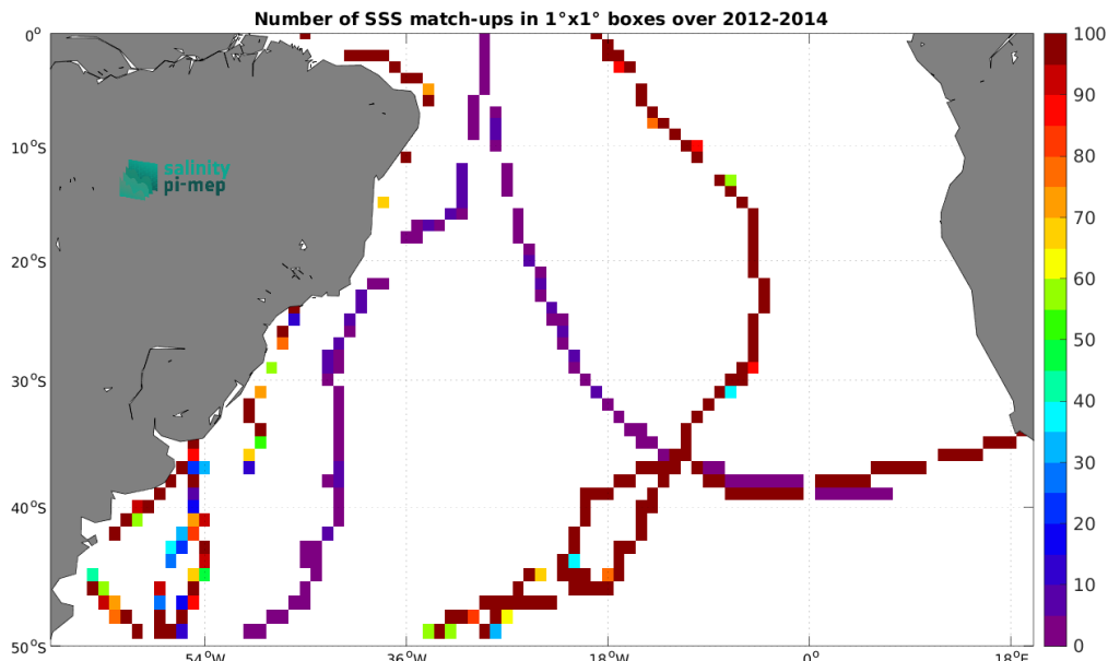
Figure 5: Number of SSS match-ups between TSG (GOSUD-Sailing-ship) SSS and the Aquarius SSS L3 CAP v5 - Monthly (JPL) SSS product for the South Atlantic Ocean Pi-MEP region over 1^\circ \times 1^\circ boxes and for the full satellite product period.
