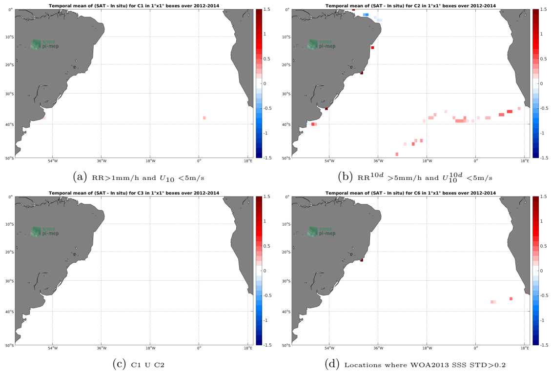
Figure 12: Temporal mean gridded over spatial boxes of size 1^\circ \times 1^\circ of \Delta SSS (Aquarius-L3-JPL-V5-MONTHLY - TSG-GOSUD-Sailing-ship) for 4 different subdatasets corresponding to: RR > 1\text{mm/h} and U_{10} < 5\text{m/s} (a), RR^{10d} > 5\text{mm/h} and U_{10}^{10d} < 5\text{m/s} (b), C1 U C2 (c), Locations where WOA2013 SSS STD > 0.2 (d).
