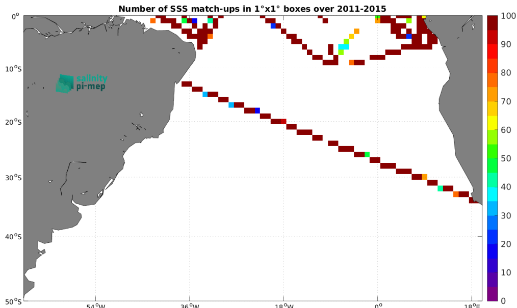
Figure 5: Number of SSS match-ups between TSG (GOSUD-Research-vessel) SSS and the Aquarius SSS L3 CAP v5 - Monthly (JPL) SSS product for the South Atlantic Ocean Pi-MEP region over 1^\circ \times 1^\circ boxes and for the full satellite product period.
