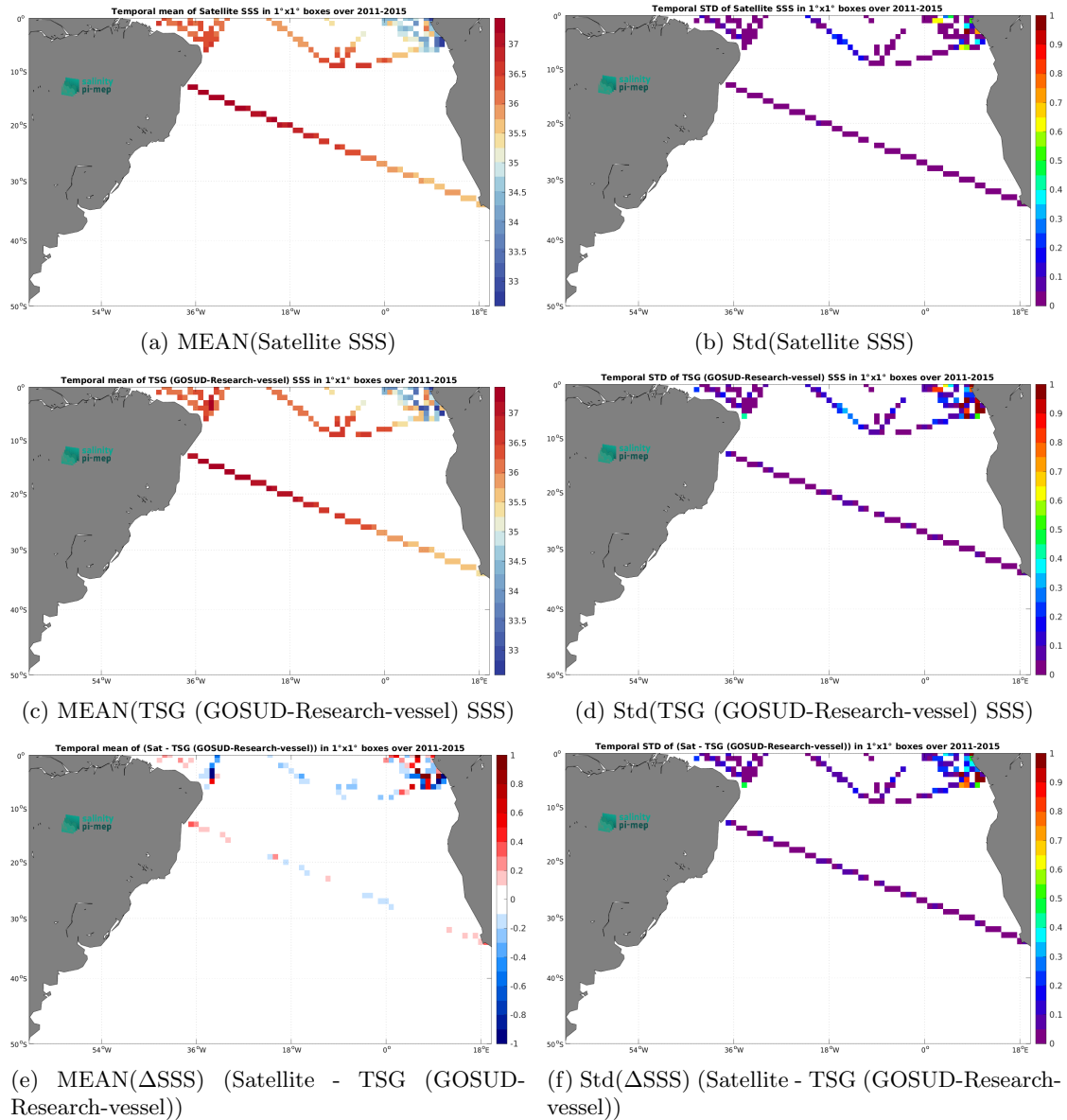
Figure 7: Temporal mean (left) and Std (right) of SSS from Aquarius SSS L3 CAP v5 - Monthly (JPL) (top), TSG (GOSUD-Research-vessel) (middle), and of \Delta SSS (Satellite - TSG (GOSUD-Research-vessel)). Only match-up pairs are used to generate these maps.
