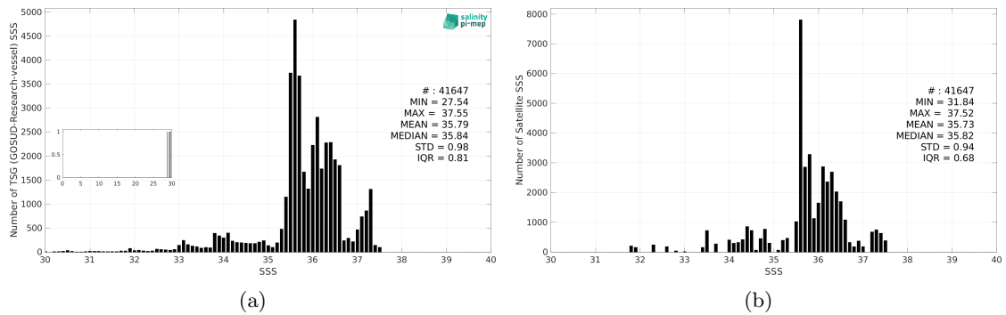
Figure 3: Histograms of SSS from TSG (GOSUD-Research-vessel) (a) and Aquarius SSS L3 CAP v5 - Monthly (JPL) (b) considering all match-up pairs per bins of 0.1 over the South Atlantic Ocean Pi-MEP region and for the full satellite product period.
