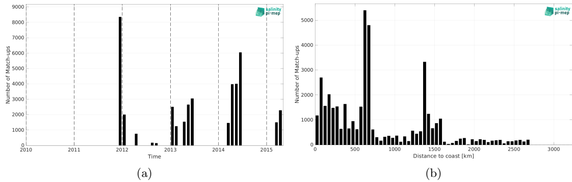
Figure 2: Number of match-ups between TSG (GOSUD-Research-vessel) and Aquarius SSS L3 CAP v5 - Monthly (JPL) SSS as a function of time (a) and as function of the distance to coast (b) over the South Atlantic Ocean Pi-MEP region and for the full satellite product period.
