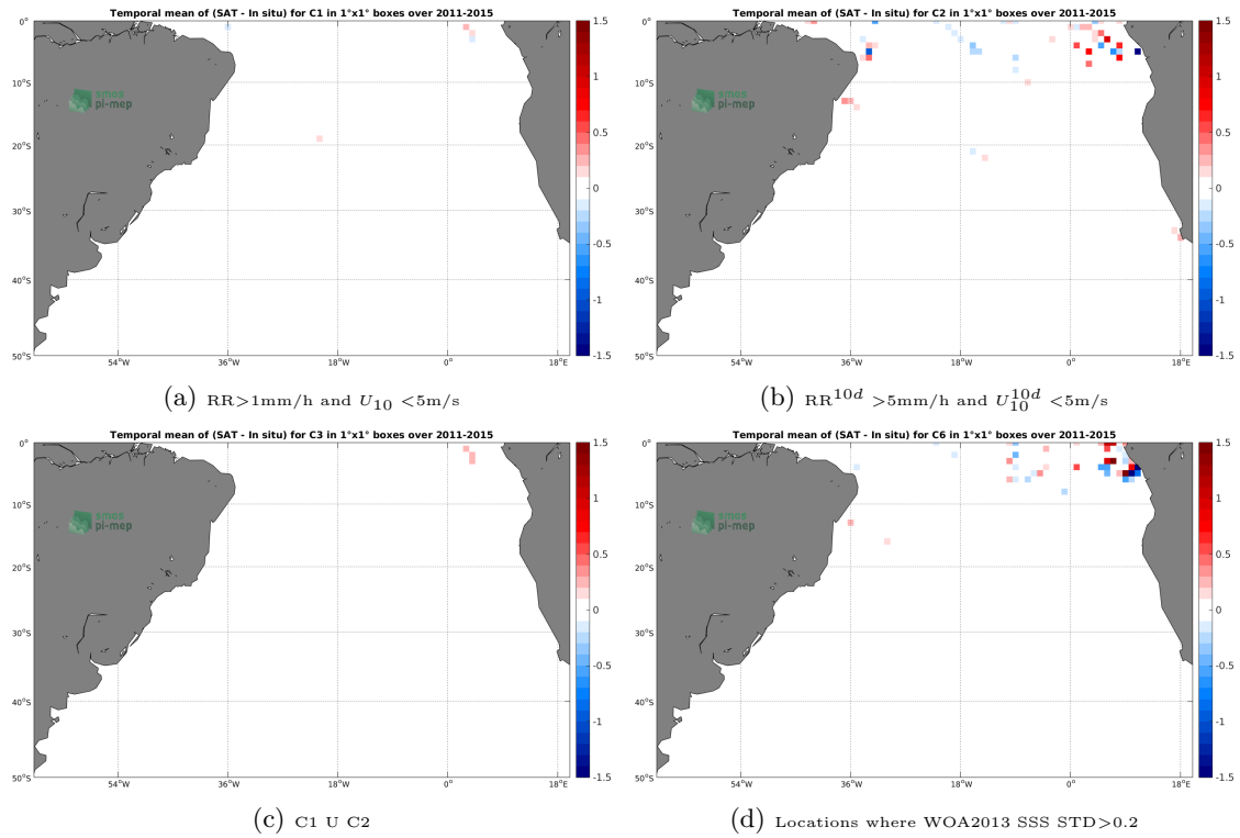
Figure 12: Temporal mean gridded over spatial boxes of size 1^\circ \times 1^\circ of \Delta SSS (Aquarius-L3-JPL-V5-MONTHLY - TSG-GOSUD-Research-vessel) for 4 different subdatasets corresponding to: RR > 1mm/h and U_{10} < 5\text{m/s} (a), RR^{10d} > 5\text{mm/h} and U_{10}^{10d} < 5\text{m/s} (b), C1 U C2 (c), Locations where WOA2013 SSS STD > 0.2 (d).
