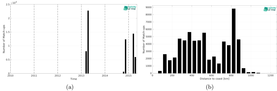
Figure 2: Number of match-ups between TSG (CSIC-UTM) and Aquarius SSS L3 CAP v5 - Monthly (JPL) SSS as a function of time (a) and as function of the distance to coast (b) over the South Atlantic Ocean Pi-MEP region and for the full satellite product period.
