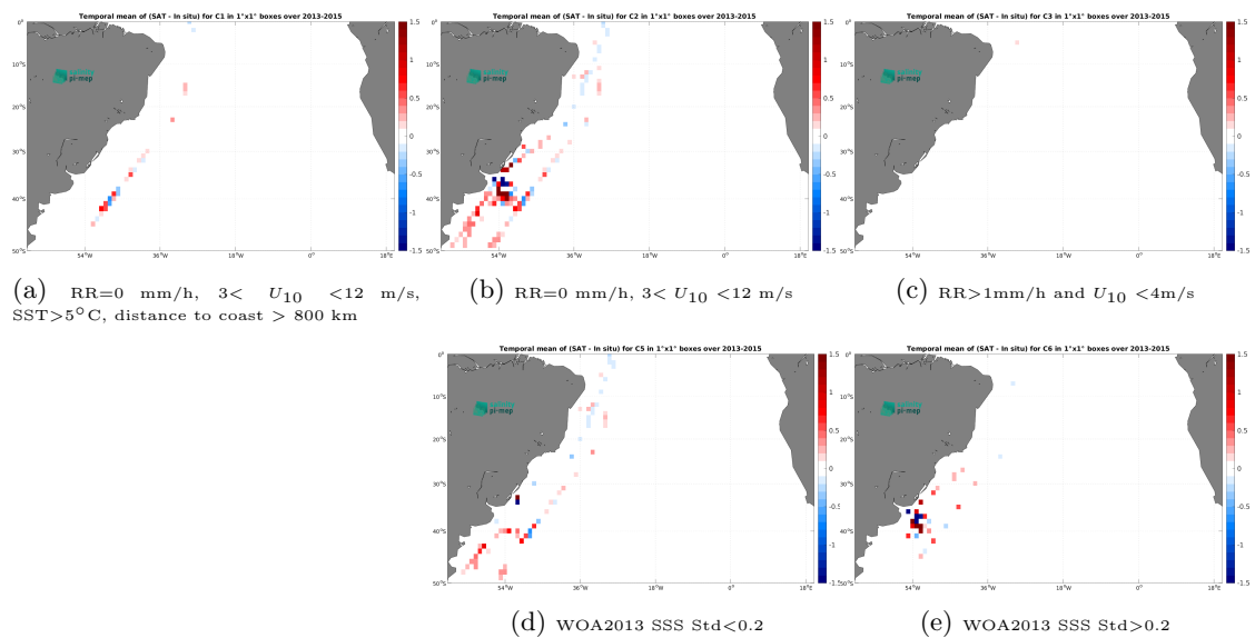
Figure 14: Temporal mean gridded over spatial boxes of size 1^\circ \times 1^\circ of \Delta\text{SSS} (Aquarius SSS L3 CAP v5 - Monthly (JPL) - TSG (CSIC-UTM)) for 5 different subdatasets corresponding to:RR=0 mm/h, 3 < U_{10} < 12 m/s, SST>5°C, distance to coast > 800 km (a), RR=0 mm/h, 3 < U_{10} < 12 m/s (b), RR>1mm/h and U_{10} < 4 m/s (c), WOA2013 SSS Std<0.2 (d), WOA2013 SSS Std>0.2 (e).
