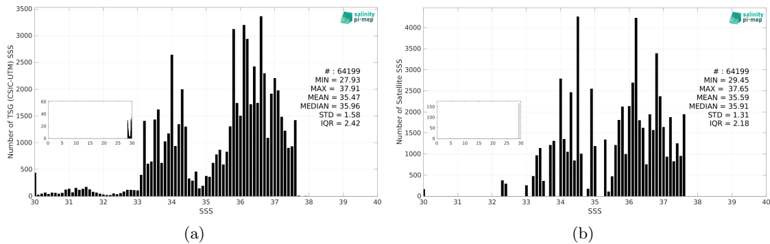
Figure 3: Histograms of SSS from TSG (CSIC-UTM) (a) and Aquarius SSS L3 CAP v5 - Monthly (JPL) (b) considering all match-up pairs per bins of 0.1 over the South Atlantic Ocean Pi-MEP region and for the full satellite product period.
