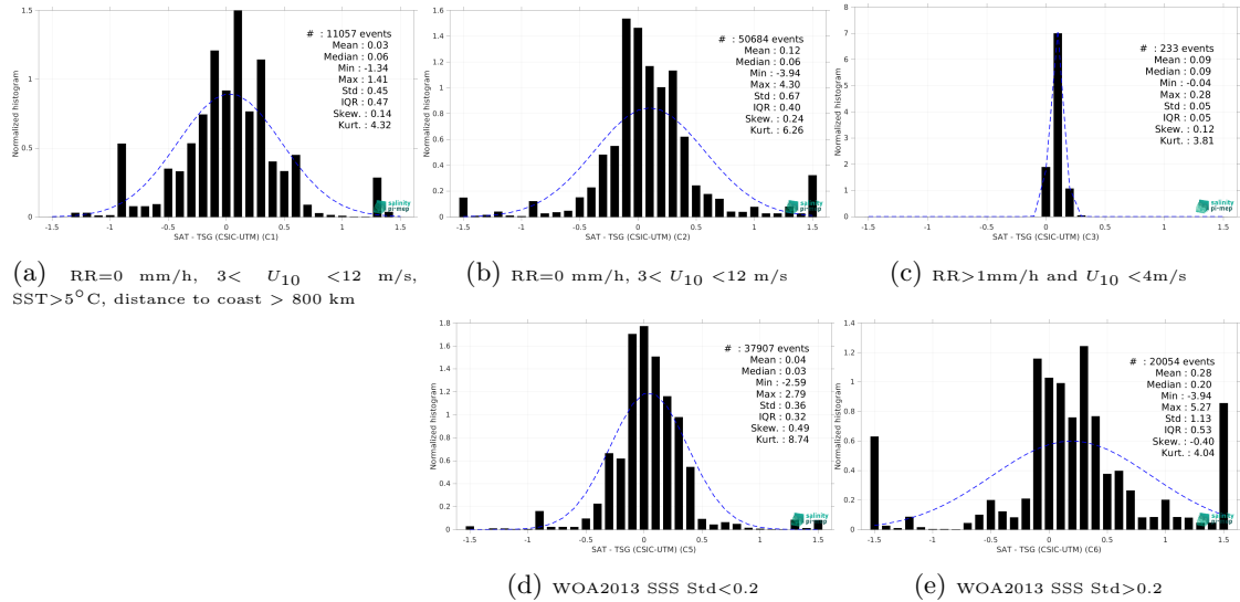
Figure 15: Normalized histogram of \Delta\text{SSS} (Aquarius SSS L3 CAP v5 - Monthly (JPL) - TSG (CSIC-UTM)) for 5 different subdatasets corresponding to: RR=0 mm/h, 3 < U_{10} < 12 m/s, SST>5°C, distance to coast > 800 km (a), RR=0 mm/h, 3 < U_{10} < 12 m/s (b), RR>1mm/h and U_{10} < 4 m/s (c), WOA2013 SSS Std<0.2 (d), WOA2013 SSS Std>0.2 (e).
