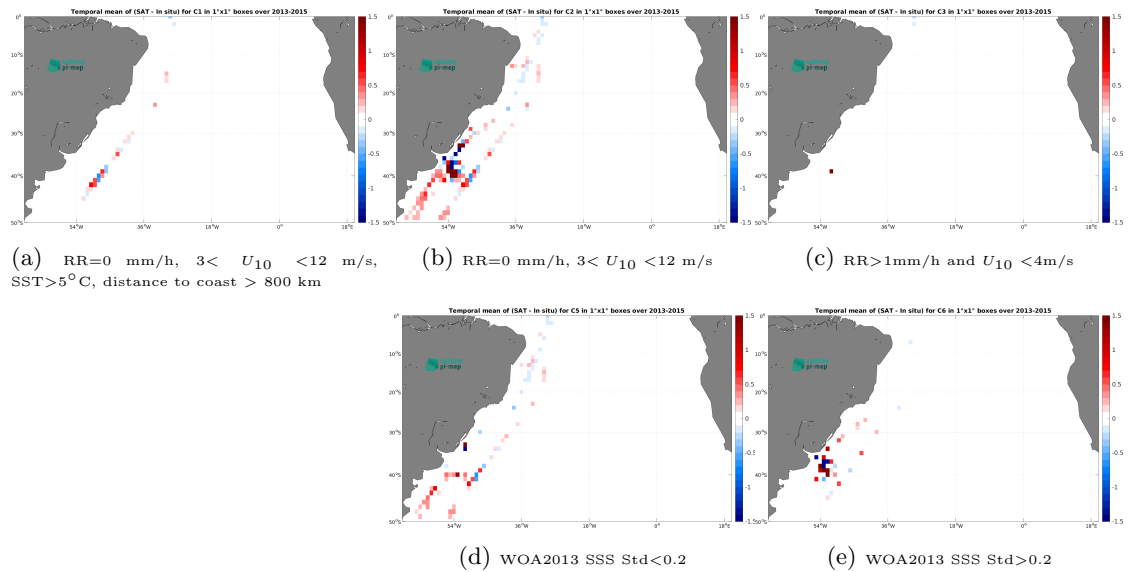
Figure 12: Temporal mean gridded over spatial boxes of size 1^\circ \times 1^\circ of \Delta\text{SSS} (Aquarius SSS L3 CAP v5 - Monthly (JPL) - TSG (CSIC-UTM)) for 5 different subdatasets corresponding to:RR=0 mm/h, 3 < U_{10} < 12 m/s, SST >5^\circ\text{C} , distance to coast > 800 km (a), RR=0 mm/h, 3 < U_{10} < 12 m/s (b), RR >1 mm/h and U_{10} < 4 m/s (c), WOA2013 SSS Std <0.2 (d), WOA2013 SSS Std >0.2 (e).
