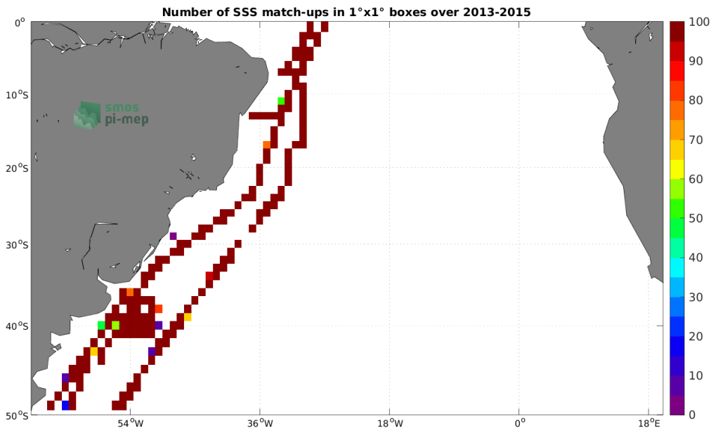
Figure 4: Number of SSS match-ups between TSG (CSIC-UTM) SSS and the Aquarius SSS L3 CAP v5 - Monthly (JPL) SSS product for the South Atlantic Ocean Pi-MEP region over 1^\circ \times 1^\circ boxes and for the full satellite product period.
