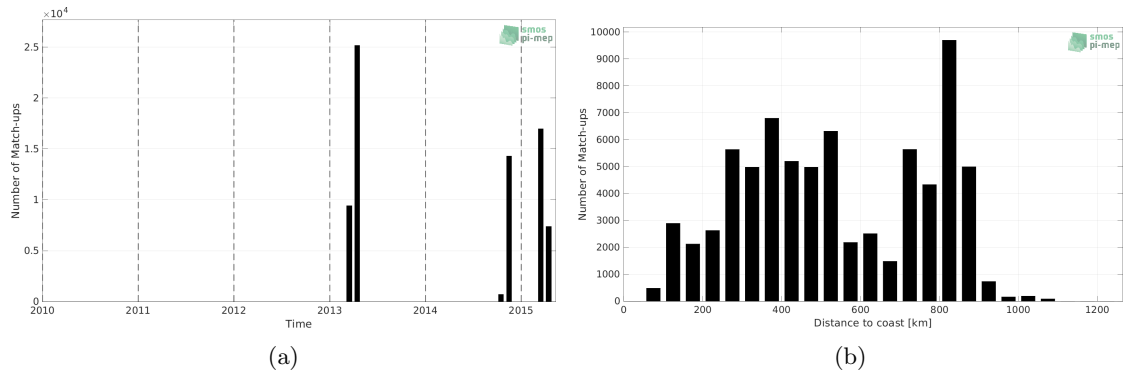
Figure 1: Number of match-ups between TSG (CSIC-UTM) and Aquarius SSS L3 CAP v5 - Monthly (JPL) SSS as a function of time (a) and as function of the distance to coast (b) over the South Atlantic Ocean Pi-MEP region and for the full satellite product period.
