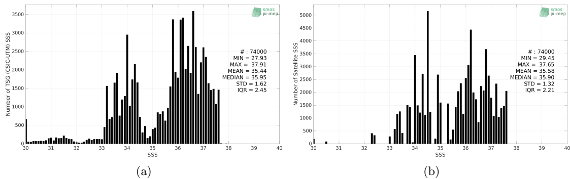
Figure 2: Histograms of SSS from TSG (CSIC-UTM) (a) and Aquarius SSS L3 CAP v5 - Monthly (JPL) (b) considering all match-up pairs per bins of 0.1 over the South Atlantic Ocean Pi-MEP region and for the full satellite product period.
