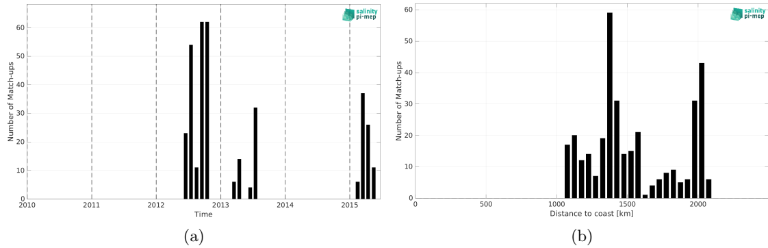
Figure 2: Number of match-ups between Marine mammals and Aquarius SSS L3 CAP v5 - Monthly (JPL) SSS as a function of time (a) and as function of the distance to coast (b) over the South Atlantic Ocean Pi-MEP region and for the full satellite product period.
