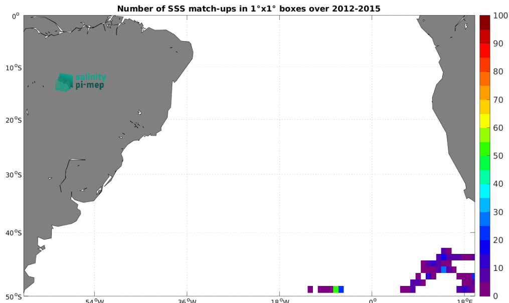
Figure 5: Number of SSS match-ups between Marine mammals SSS and the Aquarius SSS L3 CAP v5 - Monthly (JPL) SSS product for the South Atlantic Ocean Pi-MEP region over 1^\circ \times 1^\circ boxes and for the full satellite product period.
