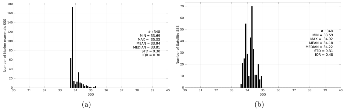
Figure 3: Histograms of SSS from Marine mammals (a) and Aquarius SSS L3 CAP v5 - Monthly (JPL) (b) considering all match-up pairs per bins of 0.1 over the South Atlantic Ocean Pi-MEP region and for the full satellite product period.
