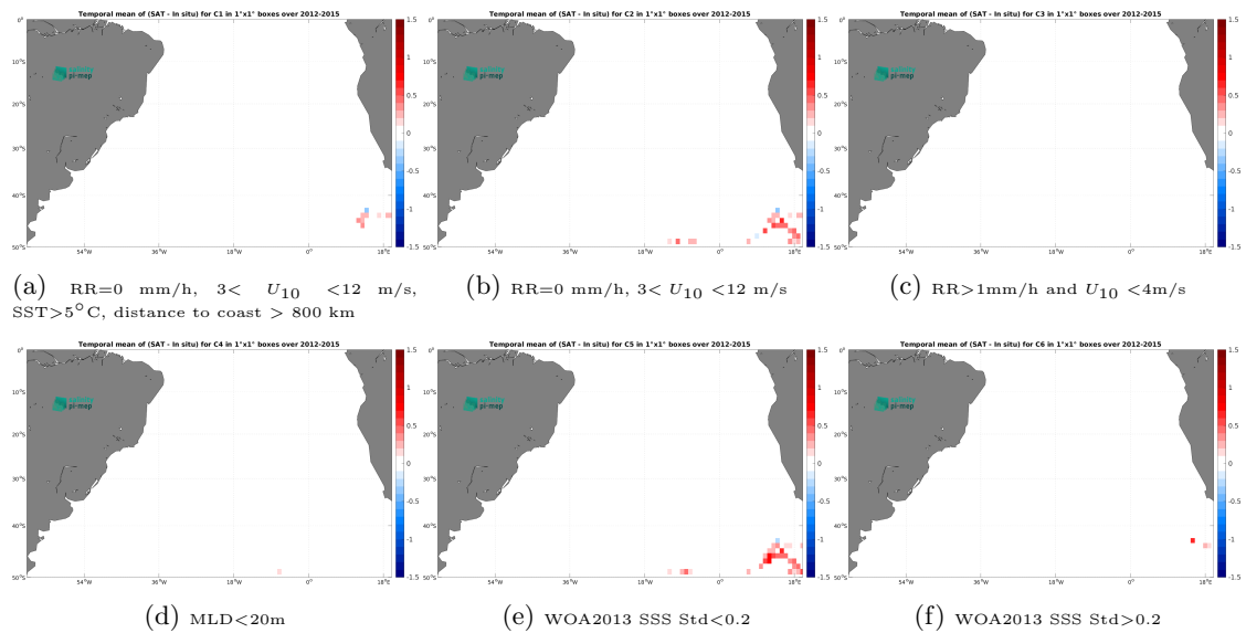
Figure 14: Temporal mean gridded over spatial boxes of size 1^\circ \times 1^\circ of \Delta SSS (Aquarius SSS L3 CAP v5 - Monthly (JPL) - Marine mammals) for 6 different subdatasets corresponding to:RR=0 mm/h, 3 < U_{10} < 12 m/s, SST > 5^\circ\text{C} , distance to coast > 800 km (a), RR=0 mm/h, 3 < U_{10} < 12 m/s (b), RR > 1 mm/h and U_{10} < 4 m/s (c),MLD < 20 m (d),WOA2013 SSS Std < 0.2 (e),WOA2013 SSS Std > 0.2 (f).
