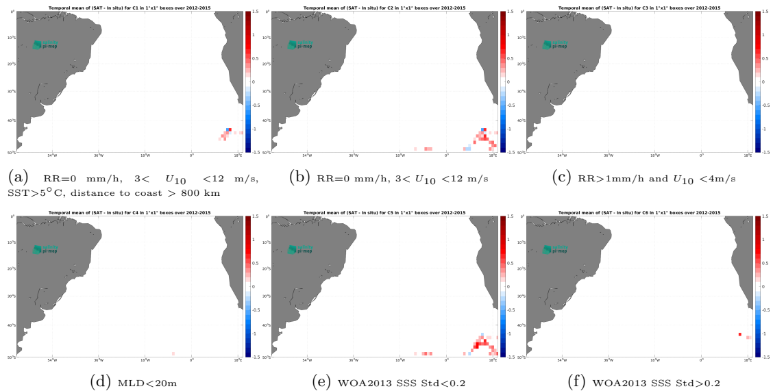
Figure 12: Temporal mean gridded over spatial boxes of size 1^{\circ}\times 1^{\circ} of \Delta\text{SSS} (Aquarius SSS L3 CAP v5 - Monthly (JPL) - Marine mammals) for 6 different subdatasets corresponding to: \text{RR}=0 mm/h, 3 < U_{10} < 12 m/s, \text{SST} > 5^{\circ}\text{C} , distance to coast > 800 km (a), \text{RR}=0 mm/h, 3 < U_{10} < 12 m/s (b), \text{RR} > 1\text{mm/h} and U_{10} < 4\text{m/s} (c), \text{MLD} < 20\text{m} (d), \text{WOA2013 SSS Std} < 0.2 (e), \text{WOA2013 SSS Std} > 0.2 (f).
