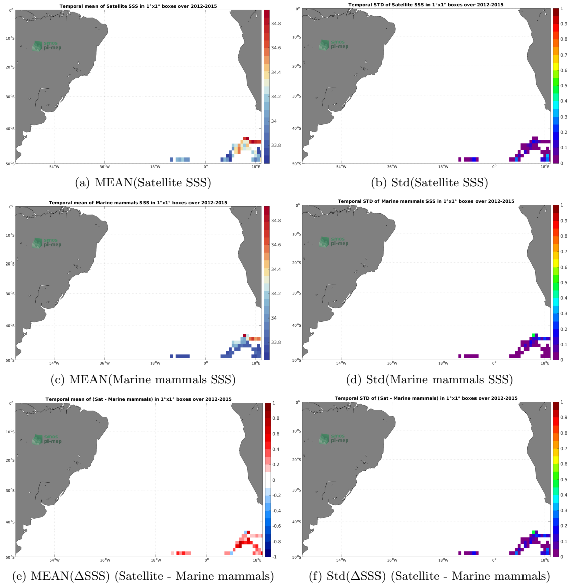
Figure 6: Temporal mean (left) and Std (right) of SSS from Aquarius SSS L3 CAP v5 - Monthly (JPL) (top), Marine mammals (middle), and of \Delta SSS (Satellite - Marine mammals). Only match-up pairs are used to generate these maps.
