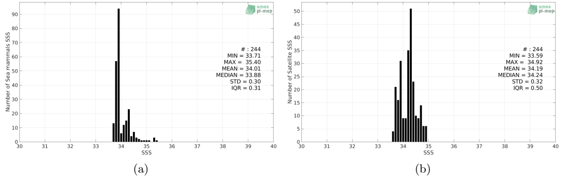
Figure 2: Histograms of SSS from Marine mammals (a) and Aquarius SSS L3 CAP v5 - Monthly (JPL) (b) considering all match-up pairs per bins of 0.1 over the South Atlantic Ocean Pi-MEP region and for the full satellite product period.
