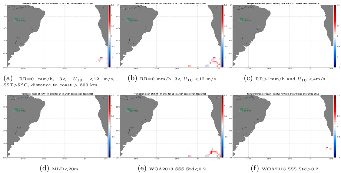
Figure 12: Temporal mean gridded over spatial boxes of size 1^{\circ}\times 1^{\circ} of \Delta\text{SSS} (Aquarius SSS L3 CAP v5 - Monthly (JPL) - Marine mammals) for 6 different subdatasets corresponding to: \text{RR}=0 mm/h, 3 < U_{10} < 12 m/s, \text{SST} > 5^{\circ}\text{C} , distance to coast > 800 km (a), \text{RR}=0 mm/h, 3 < U_{10} < 12 m/s (b), \text{RR} > 1 mm/h and U_{10} < 4 m/s (c), \text{MLD} < 20\text{m} (d), WOA2013 SSS Std < 0.2 (e), WOA2013 SSS Std > 0.2 (f).
