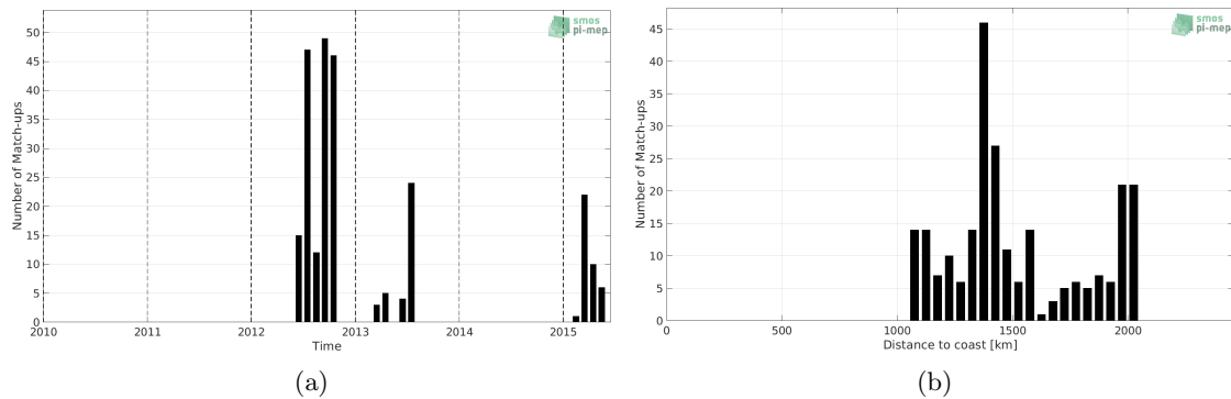
Figure 1: Number of match-ups between Marine mammals and Aquarius SSS L3 CAP v5 - Monthly (JPL) SSS as a function of time (a) and as function of the distance to coast (b) over the South Atlantic Ocean Pi-MEP region and for the full satellite product period.
