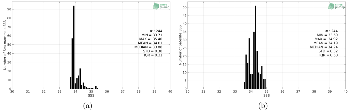
Figure 2: Histograms of SSS from Sea mammals (a) and Aquarius SSS L3 CAP v5 - Monthly (JPL) (b) considering all match-up pairs per bins of 0.1 over the South Atlantic Ocean Pi-MEP region and for the full satellite product period.
