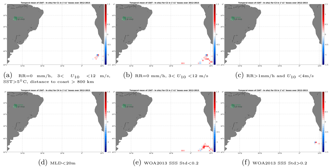
Figure 12: Temporal mean gridded over spatial boxes of size 1^{\circ}\times 1^{\circ} of \Delta\text{SSS} (Aquarius SSS L3 CAP v5 - Monthly (JPL) - Sea mammals) for 6 different subdatasets corresponding to: \text{RR}=0 mm/h, 3 < U_{10} < 12 m/s, \text{SST} > 5^{\circ}\text{C} , distance to coast > 800 km (a), \text{RR}=0 mm/h, 3 < U_{10} < 12 m/s (b), \text{RR} > 1 mm/h and U_{10} < 4 m/s (c), \text{MLD} < 20\text{m} (d), WOA2013 SSS Std < 0.2 (e), WOA2013 SSS Std > 0.2 (f).
