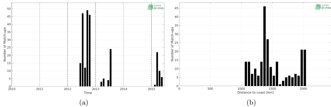
Figure 1: Number of match-ups between Sea mammals and Aquarius SSS L3 CAP v5 - Monthly (JPL) SSS as a function of time (a) and as function of the distance to coast (b) over the South Atlantic Ocean Pi-MEP region and for the full satellite product period.
