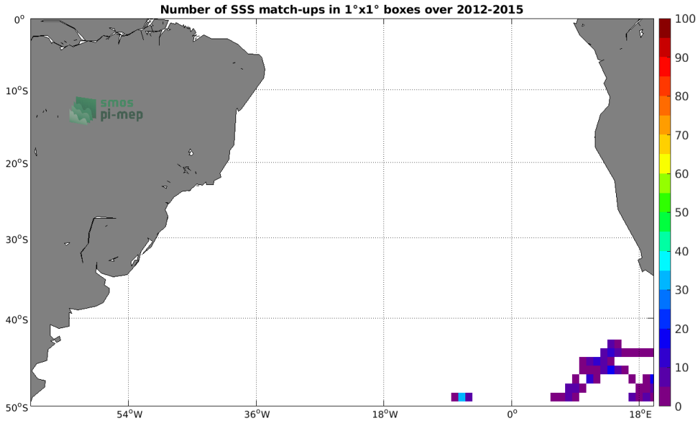
Figure 4: Number of SSS match-ups between Sea mammals SSS and the Aquarius SSS L3 CAP v5 - Monthly (JPL) SSS product for the South Atlantic Ocean Pi-MEP region over 1^{\circ} \times 1^{\circ} boxes and for the full satellite product period.
