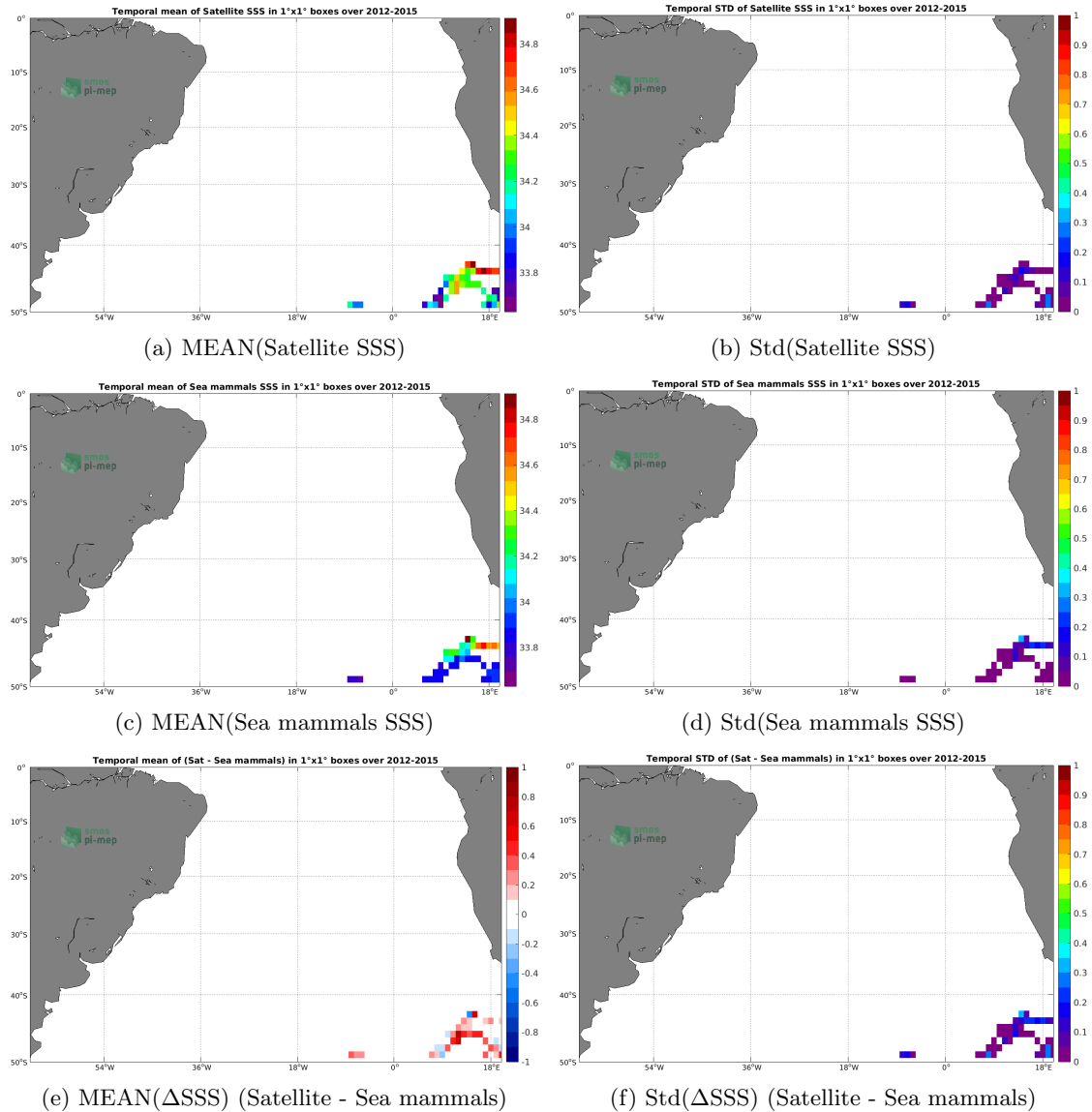
Figure 6: Temporal mean (left) and Std (right) of SSS from Aquarius SSS L3 CAP v5 - Monthly (JPL) (top), Sea mammals (middle), and of \Delta SSS (Satellite - Sea mammals). Only match-up pairs are used to generate these maps.
