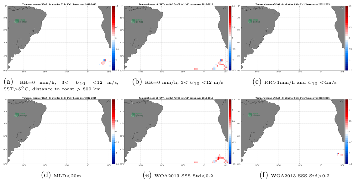
Figure 12: Temporal mean gridded over spatial boxes of size 1^{\circ}\times 1^{\circ} of \Delta\text{SSS} (Aquarius-L3-JPL-V5-MONTHLY - Sea mammals) for 6 different subdatasets corresponding to:RR=0 mm/h, 3 < U_{10} < 12 m/s, SST > 5^{\circ}\text{C} , distance to coast > 800 km (a), RR=0 mm/h, 3 < U_{10} < 12 m/s (b), RR > 1 mm/h and U_{10} < 4 m/s (c),MLD < 20 m (d),WOA2013 SSS Std < 0.2 (e),WOA2013 SSS Std > 0.2 (f).
