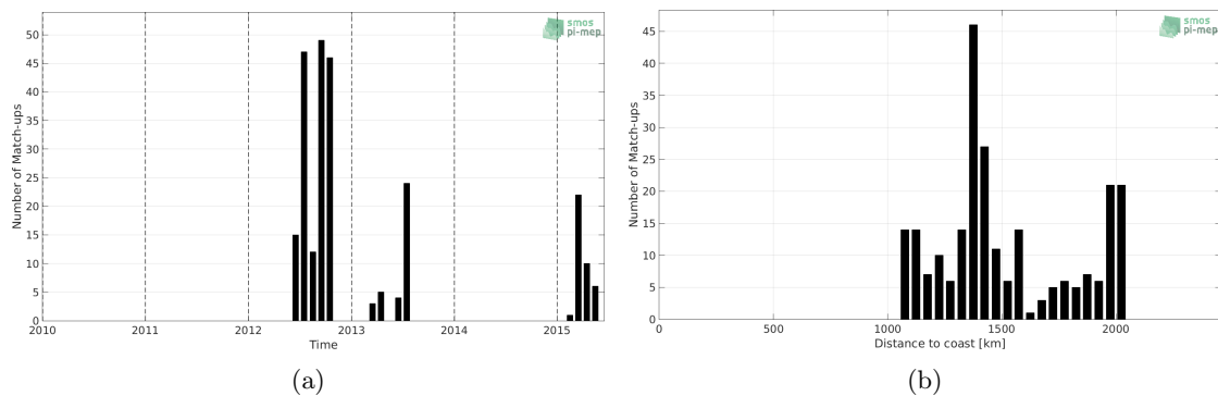
Figure 1: Number of match-ups between Sea mammals and Aquarius-L3-JPL-V5-MONTHLY SSS as a function of time (a) and as function of the distance to coast (b) over the South Atlantic Ocean Pi-MEP region and for the full satellite product period.
