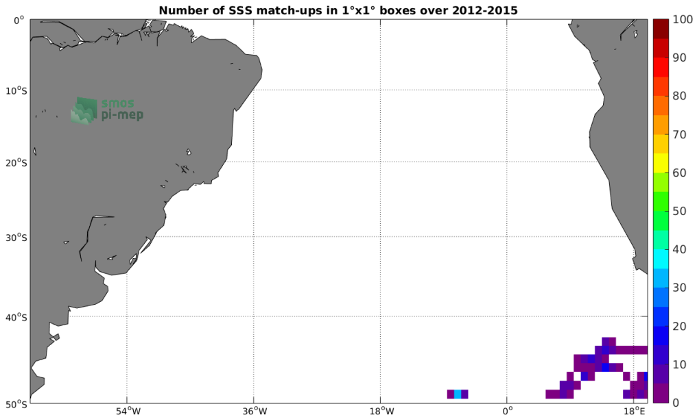
Figure 4: Number of SSS match-ups between Sea mammals SSS and the Aquarius-L3-JPL-V5-MONTHLY SSS product for the South Atlantic Ocean Pi-MEP region over 1^\circ \times 1^\circ boxes and for the full satellite product period.
