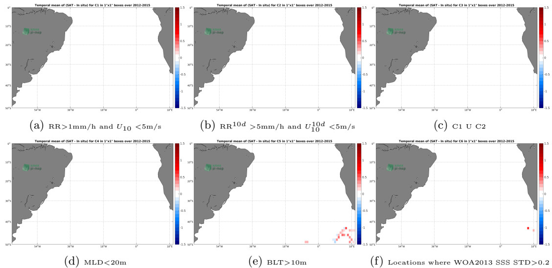
Figure 12: Temporal mean gridded over spatial boxes of size 1^\circ \times 1^\circ of \Delta\text{SSS} (Aquarius-L3-JPL-V5-MONTHLY - Sea mammals) for 6 different subdatasets corresponding to: \text{RR} > 1\text{mm/h} and U_{10} < 5\text{m/s} (a), \text{RR}^{10d} > 5\text{mm/h} and U_{10}^{10d} < 5\text{m/s} (b), C1 U C2 (c), \text{MLD} < 20\text{m} (d), \text{BLT} > 10\text{m} (e), Locations where WOA2013 SSS STD > 0.2 (f).
