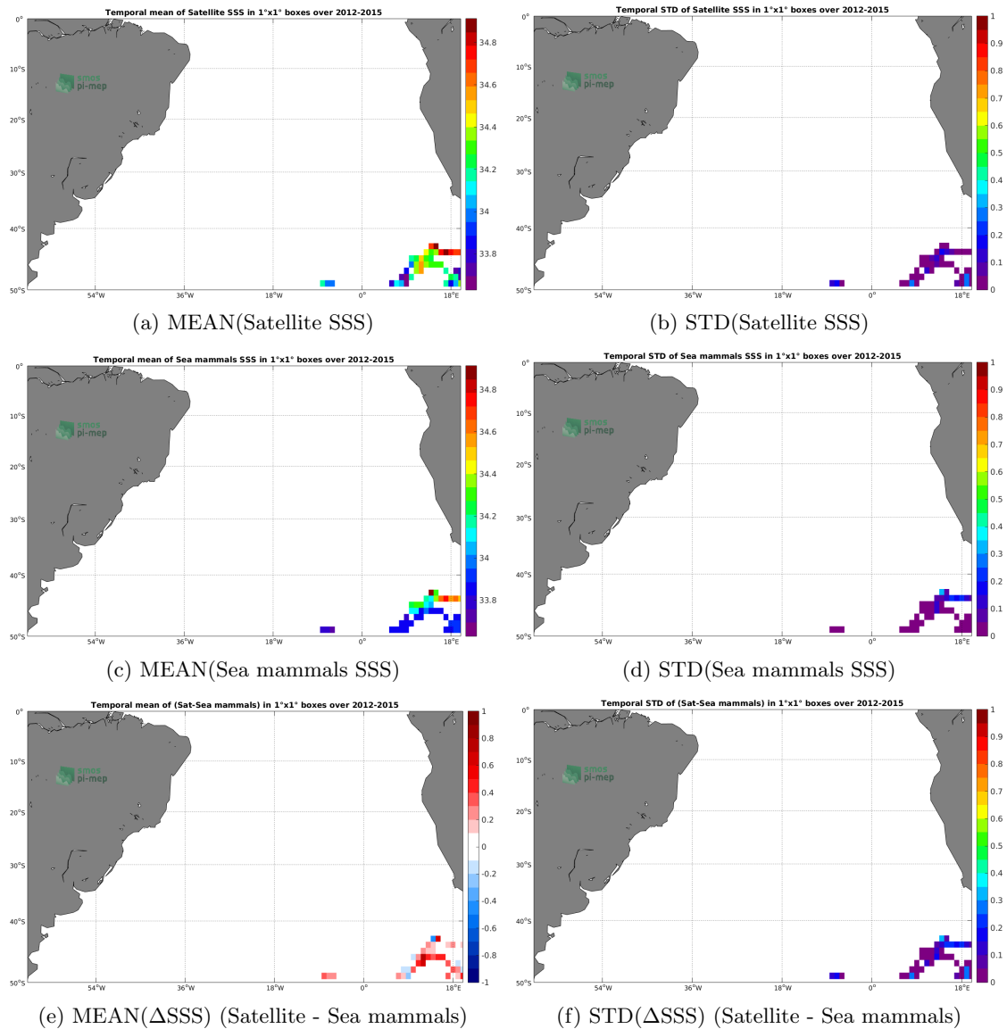
Figure 6: Temporal mean (left) and STD (right) of SSS from Aquarius-L3-JPL-V5-MONTHLY (top), Sea mammals (middle), and of \Delta SSS (Satellite - Sea mammals). Only match-up pairs are used to generate these maps.
