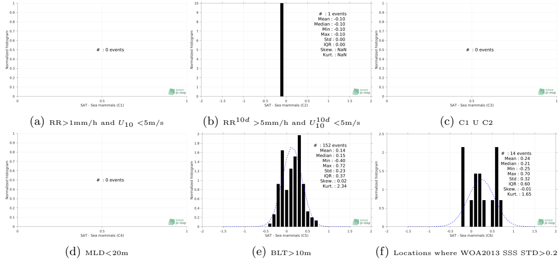
Figure 13: Normalized histogram of \Delta\text{SSS} (Aquarius-L3-JPL-V5-MONTHLY - Sea mammals) for 6 different subdatasets corresponding to: \text{RR} > 1\text{mm/h} and U_{10} < 5\text{m/s} (a), \text{RR}^{10d} > 5\text{mm/h} and U_{10}^{10d} < 5\text{m/s} (b), C1 \cup C2 (c), \text{MLD} < 20\text{m} (d), \text{BLT} > 10\text{m} (e), Locations where WOA2013 SSS \text{STD} > 0.2 (f).
