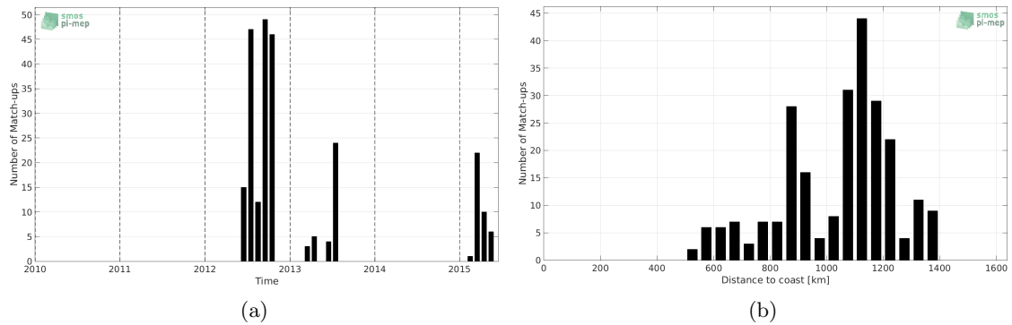
Figure 1: Number of match-ups between Sea mammals and Aquarius-L3-JPL-V5-MONTHLY SSS as a function of time (a) and as function of the distance to coast (b) over the South Atlantic Ocean Pi-MEP region and for the full satellite product period.
