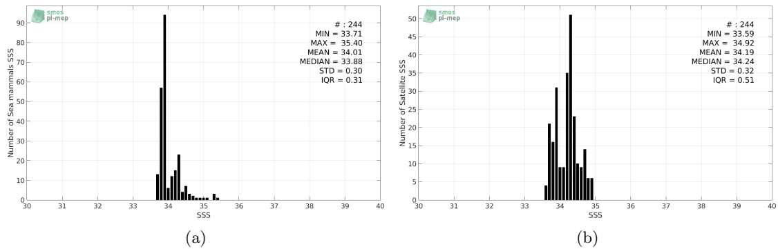
Figure 2: Histograms of SSS from Sea mammals (a) and Aquarius-L3-JPL-V5-MONTHLY (b) considering all match-up pairs per bins of 0.1 over the South Atlantic Ocean Pi-MEP region and for the full satellite product period.
