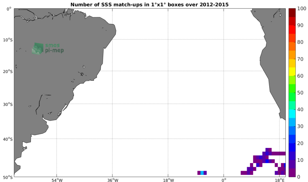
Figure 4: Number of SSS match-ups between Sea mammals SSS and the Aquarius-L3-JPL-V5-MONTHLY SSS product for the South Atlantic Ocean Pi-MEP region over 1^{\circ} \times 1^{\circ} boxes and for the full satellite product period.
