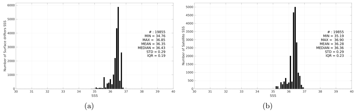
Figure 3: Histograms of SSS from Surface drifters (a) and Aquarius SSS L3 CAP v5 - Monthly (JPL) (b) considering all match-up pairs per bins of 0.1 over the South Atlantic Ocean Pi-MEP region and for the full satellite product period.
