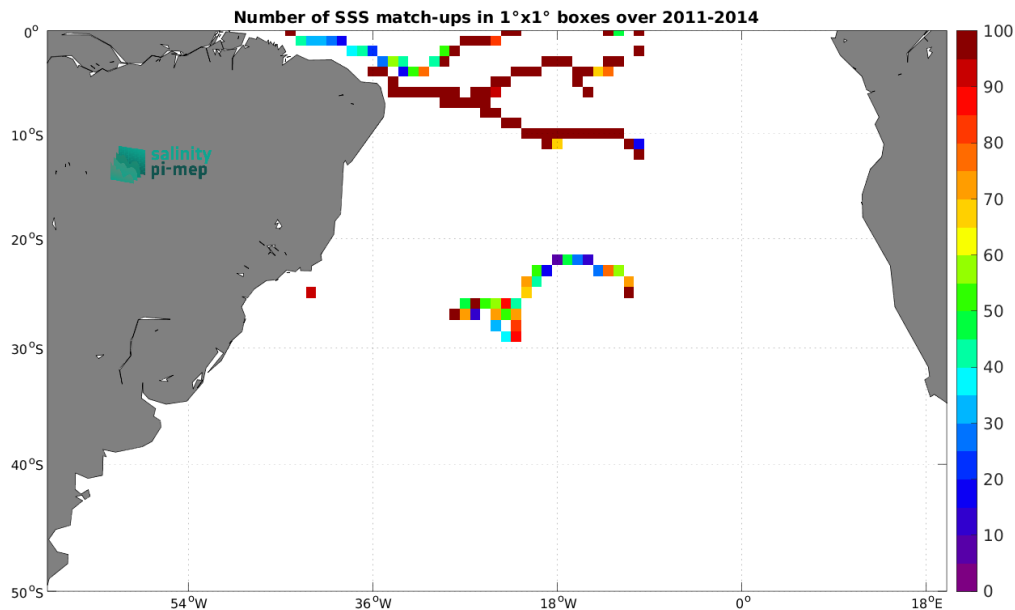
Figure 4: Number of SSS match-ups between Surface drifters SSS and the Aquarius SSS L3 CAP v5 - Monthly (JPL) SSS product for the South Atlantic Ocean Pi-MEP region over 1^\circ \times 1^\circ boxes and for the full satellite product period.
