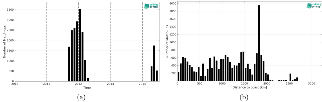
Figure 2: Number of match-ups between Surface drifters and Aquarius SSS L3 CAP v5 - Monthly (JPL) SSS as a function of time (a) and as function of the distance to coast (b) over the South Atlantic Ocean Pi-MEP region and for the full satellite product period.
