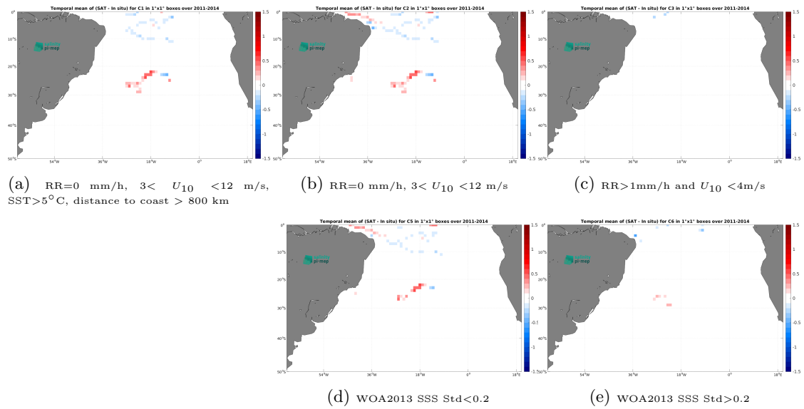
Figure 11: Temporal mean gridded over spatial boxes of size 1^\circ \times 1^\circ of \Delta\text{SSS} (Aquarius SSS L3 CAP v5 - Monthly (JPL) - Surface drifters) for 5 different subdatasets corresponding to:RR=0 mm/h, 3 < U_{10} < 12 m/s, SST >5^\circ\text{C} , distance to coast > 800 km (a), RR=0 mm/h, 3 < U_{10} < 12 m/s (b), RR >1 mm/h and U_{10} < 4 m/s (c), WOA2013 SSS Std <0.2 (d), WOA2013 SSS Std >0.2 (e).
