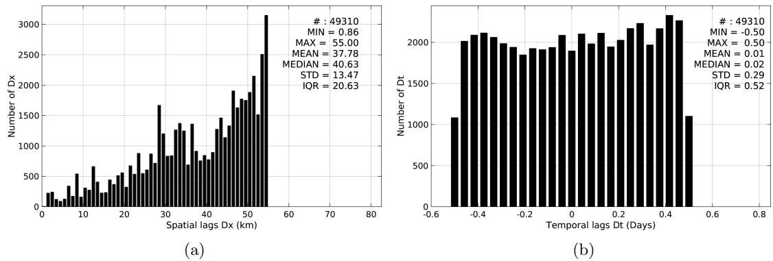
Figure 5: Histograms of the spatial (a) and temporal (b) lags between the time of the TSG-SAMOS measurements and the date of the corresponding Aquarius-L3-JPL-V4-7DAY-RUNNING SSS product.
