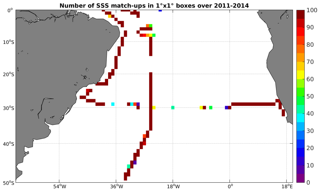
Figure 4: Number of SSS match-ups between TSG-SAMOS SSS and the Aquarius-L3-JPL-V4-7DAY-RUNNING SSS product for the South Atlantic Ocean Pi-MEP region over 1^{\circ} \times 1^{\circ} boxes and for the full satellite product period.
