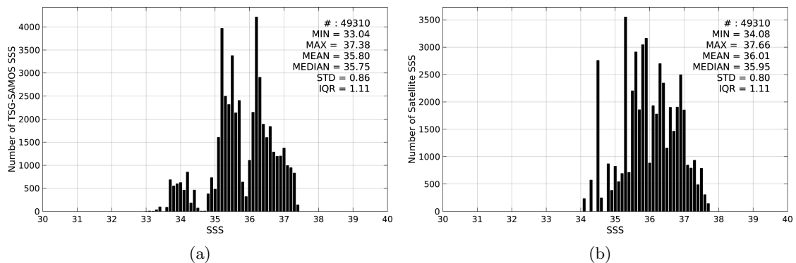
Figure 2: Histograms of SSS from TSG-SAMOS (a) and Aquarius-L3-JPL-V4-7DAY-RUNNING (b) considering all match-up pairs per bins of 0.1 over the South Atlantic Ocean Pi-MEP region and for the full satellite product period.
