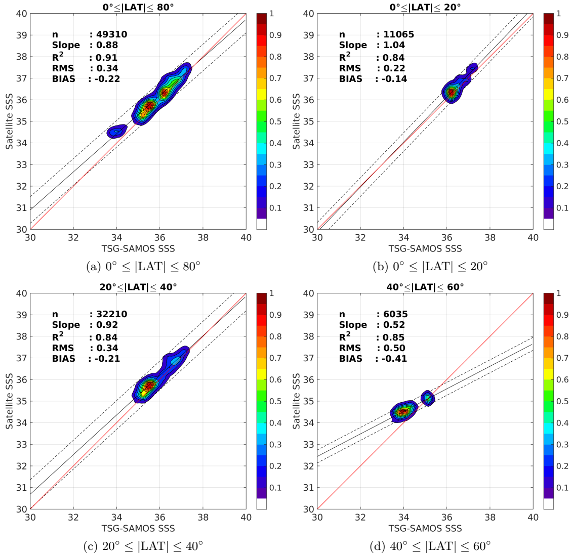
Figure 9: Contour maps of the concentration of Aquarius-L3-JPL-V4-7DAY-RUNNING SSS (y-axis) versus TSG-SAMOS SSS (x-axis) at match-up pairs for different latitude bands. For each plot, the red line shows x=y . The black thin and dashed lines indicate a linear fit through the data cloud and the \pm 95\% confidence levels, respectively. The number match-up pairs n , the slope and R^2 coefficient of the linear fit, the root mean square (RMS) and the mean bias between satellite and in situ data are indicated for each latitude band in each plots.
