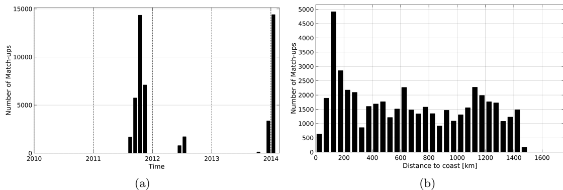
Figure 1: Number of match-ups between TSG-SAMOS and Aquarius-L3-JPL-V4-7DAY-RUNNING SSS as a function of time (a) and as function of the distance to coast (b) over the South Atlantic Ocean Pi-MEP region and for the full satellite product period.
