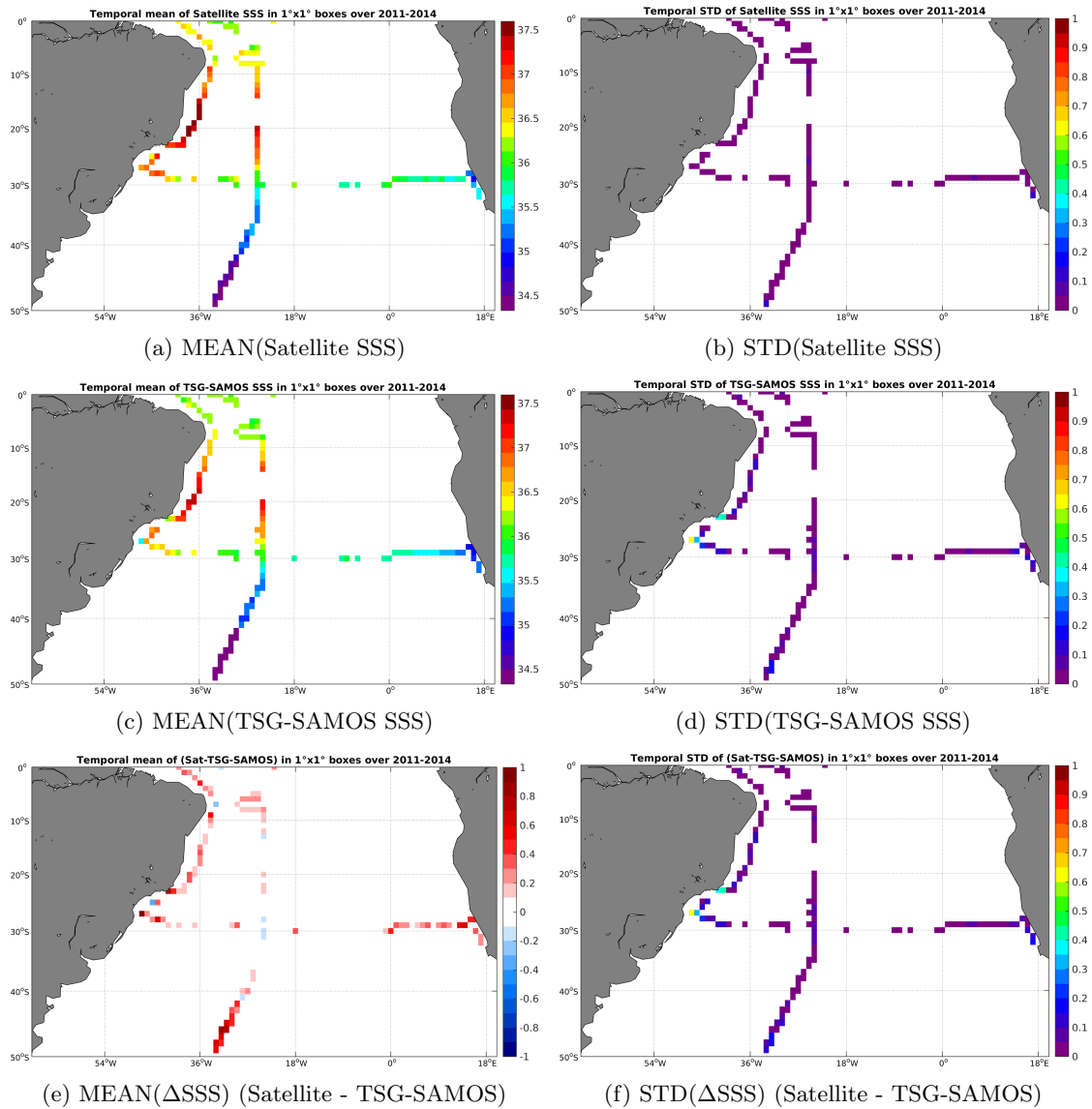
Figure 6: Temporal mean (left) and STD (right) of SSS from Aquarius-L3-JPL-V4-7DAY-RUNNING (top), TSG-SAMOS (middle), and of \Delta SSS (Satellite - TSG-SAMOS). Only match-up pairs are used to generate these maps.
