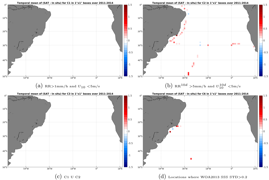
Figure 12: Temporal mean gridded over spatial boxes of size 1^\circ \times 1^\circ of \Delta SSS (Aquarius-L3-JPL-V4-7DAY-RUNNING - TSG-SAMOS) for 4 different subdatasets corresponding to:RR > 1 mm/h and U_{10} < 5 m/s (a), RR^{10d} > 5 mm/h and U_{10}^{10d} < 5 m/s (b), C1 U C2 (c),Locations where WOA2013 SSS STD > 0.2 (d).
