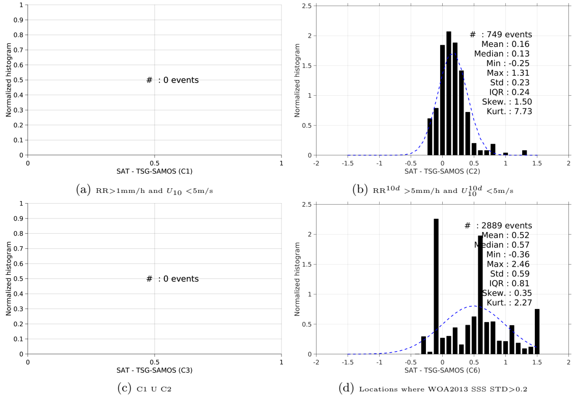
Figure 13: Normalized histogram of \Delta\text{SSS} (Aquarius-L3-JPL-V4-7DAY-RUNNING - TSG-SAMOS) for 6 different subdatasets corresponding to: RR > 1\text{mm/h} and U_{10} < 5\text{m/s} (a), RR^{10d} > 5\text{mm/h} and U_{10}^{10d} < 5\text{m/s} (b), C1 \cup C2 (c), Locations where WOA2013 SSS STD > 0.2 (d).
