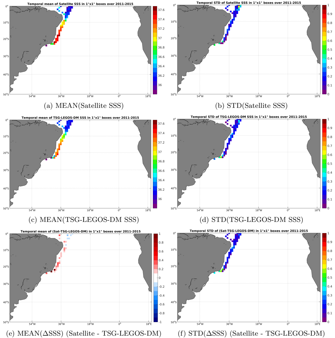
Figure 6: Temporal mean (left) and STD (right) of SSS from Aquarius-L3-JPL-V4-7DAY-RUNNING (top), TSG-LEGOS-DM (middle), and of \Delta SSS (Satellite - TSG-LEGOS-DM). Only match-up pairs are used to generate these maps.
