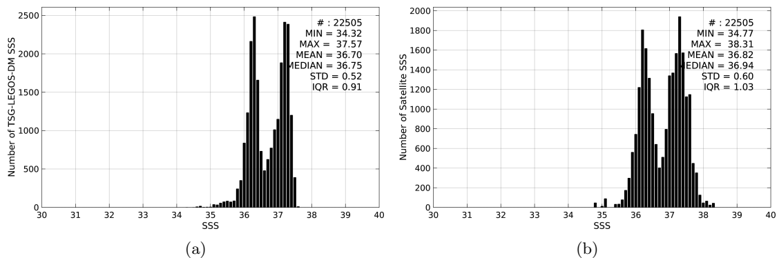
Figure 2: Histograms of SSS from TSG-LEGOS-DM (a) and Aquarius-L3-JPL-V4-7DAY-RUNNING (b) considering all match-up pairs per bins of 0.1 over the South Atlantic Ocean Pi-MEP region and for the full satellite product period.
