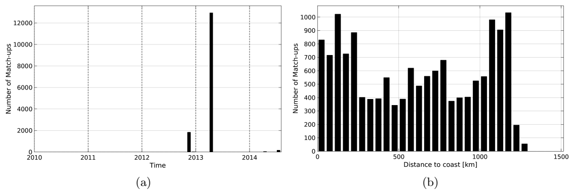
Figure 1: Number of match-ups between TSG-GOSUD-Sailing-ship and Aquarius-L3-JPL-V4-7DAY-RUNNING SSS as a function of time (a) and as function of the distance to coast (b) over the South Atlantic Ocean Pi-MEP region and for the full satellite product period.
