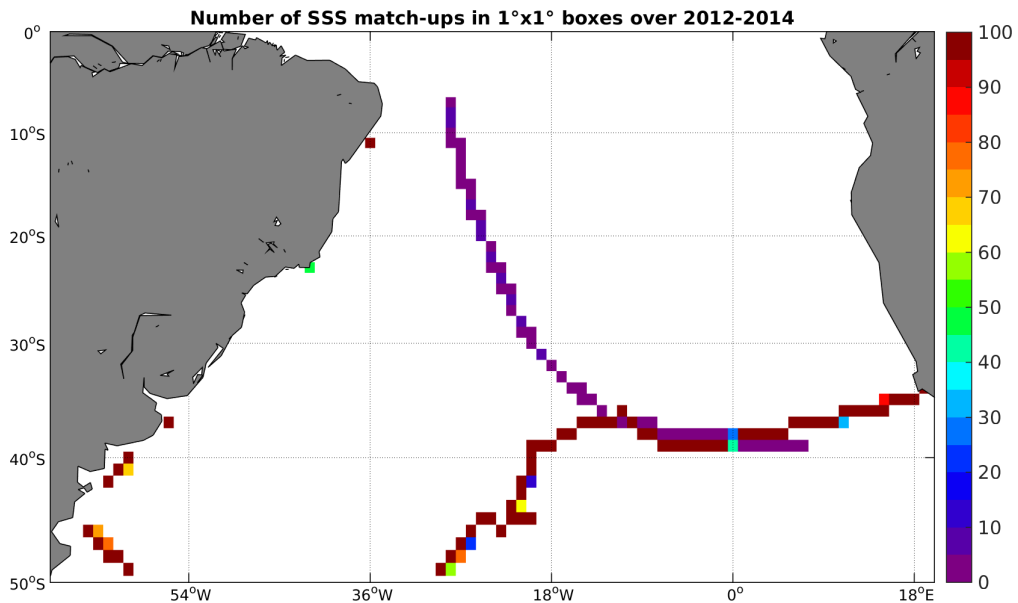
Figure 4: Number of SSS match-ups between TSG-GOSUD-Sailing-ship SSS and the Aquarius-L3-JPL-V4-7DAY-RUNNING SSS product for the South Atlantic Ocean Pi-MEP region over 1^{\circ} \times 1^{\circ} boxes and for the full satellite product period.
