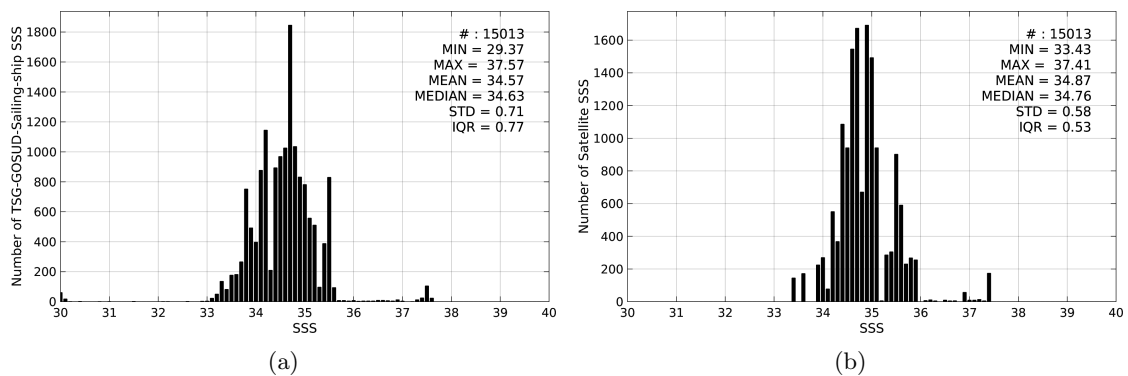
Figure 2: Histograms of SSS from TSG-GOSUD-Sailing-ship (a) and Aquarius-L3-JPL-V4-7DAY-RUNNING (b) considering all match-up pairs per bins of 0.1 over the South Atlantic Ocean Pi-MEP region and for the full satellite product period.
