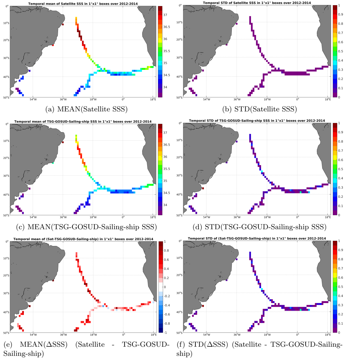
Figure 6: Temporal mean (left) and STD (right) of SSS from Aquarius-L3-JPL-V4-7DAY-RUNNING (top), TSG-GOSUD-Sailing-ship (middle), and of \Delta SSS (Satellite - TSG-GOSUD-Sailing-ship). Only match-up pairs are used to generate these maps.
