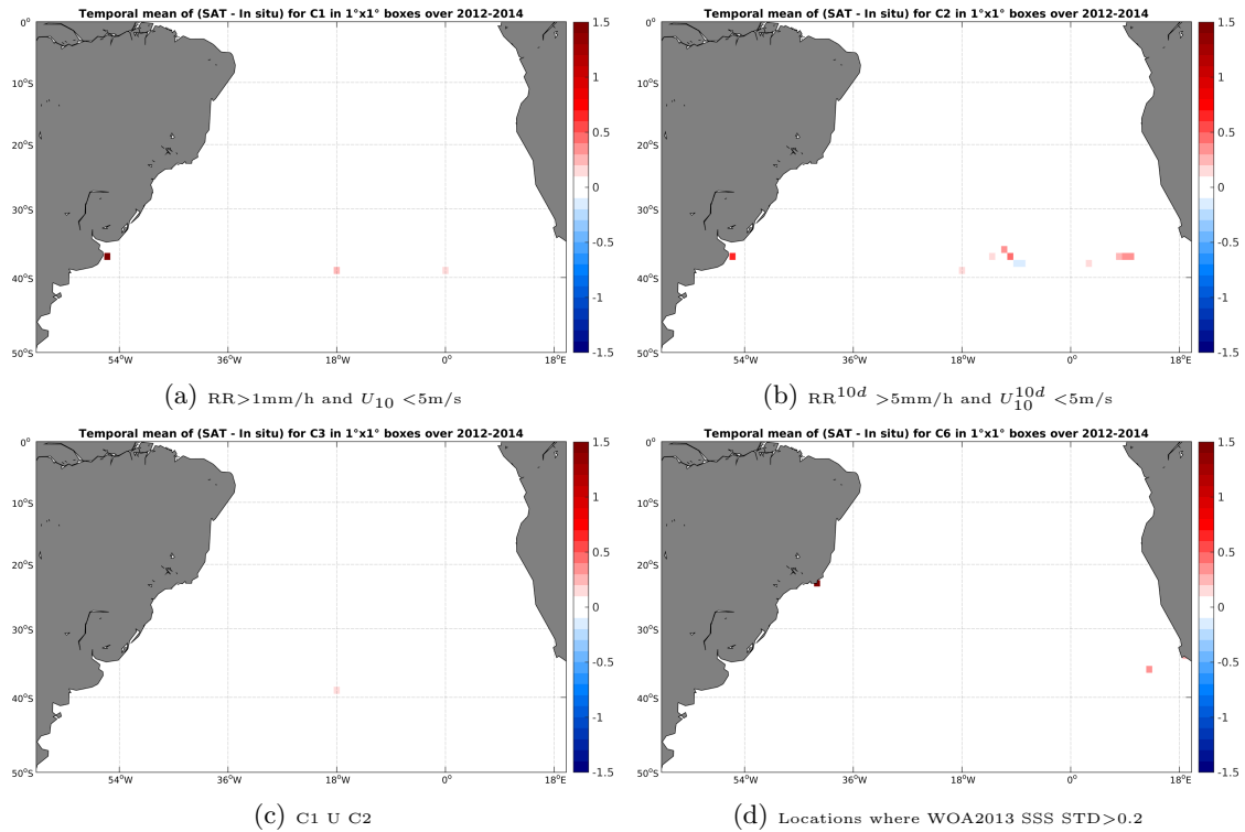
Figure 12: Temporal mean gridded over spatial boxes of size 1°x1° of \Delta SSS (Aquarius-L3-JPL-V4-7DAY-RUNNING - TSG-GOSUD-Sailing-ship) for 4 different subdatasets corresponding to: RR > 1mm/h and U_{10} < 5\text{m/s} (a), RR^{10d} > 5\text{mm/h} and U_{10}^{10d} < 5\text{m/s} (b), C1 U C2 (c), Locations where WOA2013 SSS STD > 0.2 (d).
