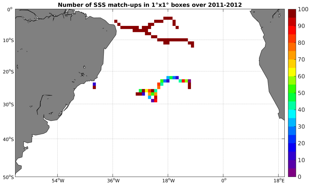
Figure 3: Number of SSS match-ups between Surface drifters SSS and the Aquarius-L3-JPL-V4-7DAY-RUNNING SSS product for the South Atlantic Ocean Pi-MEP region over 1^{\circ} \times 1^{\circ} boxes and for the full satellite product period.
