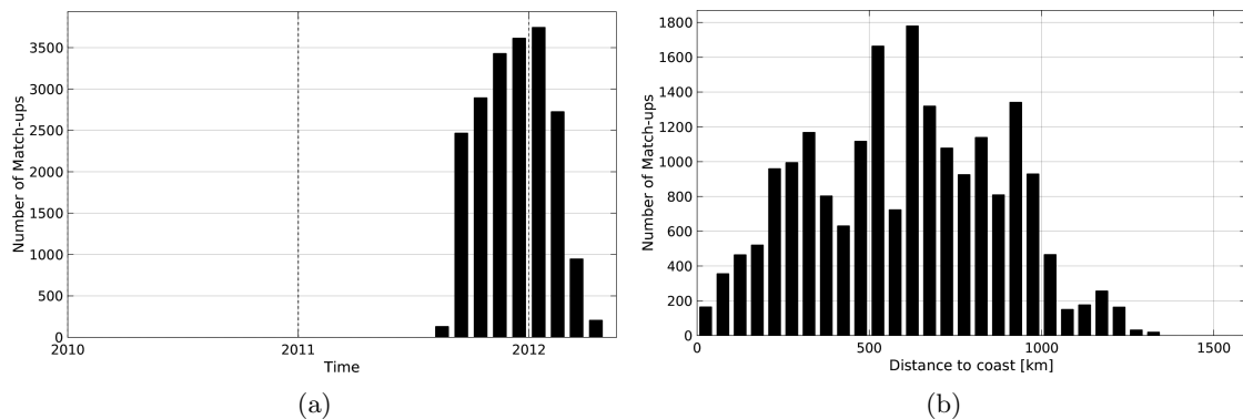
Figure 1: Number of match-ups between Surface drifters and Aquarius-L3-JPL-V4-7DAY-RUNNING SSS as a function of time (a) and as function of the distance to coast (b) over the South Atlantic Ocean Pi-MEP region and for the full satellite product period.
