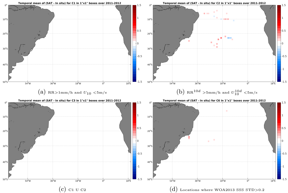
Figure 11: Temporal mean gridded over spatial boxes of size 1^\circ \times 1^\circ of \Delta SSS (Aquarius-L3-JPL-V4-7DAY-RUNNING - Surface drifters) for 4 different subdatasets corresponding to: RR > 1\text{mm/h} and U_{10} < 5\text{m/s} (a), RR^{10d} > 5\text{mm/h} and U_{10}^{10d} < 5\text{m/s} (b), C1 U C2 (c), Locations where WOA2013 SSS STD > 0.2 (d).
