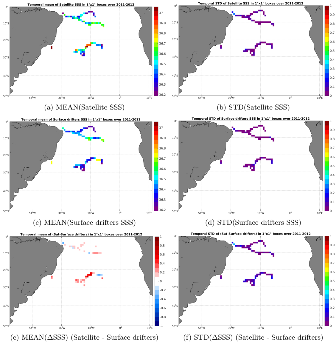
Figure 5: Temporal mean (left) and STD (right) of SSS from Aquarius-L3-JPL-V4-7DAY-RUNNING (top), Surface drifters (middle), and of \Delta SSS (Satellite - Surface drifters). Only match-up pairs are used to generate these maps.
