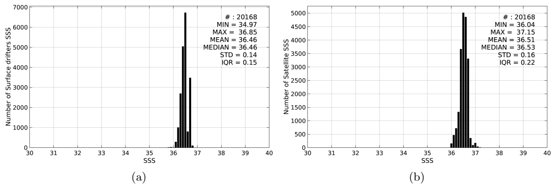
Figure 2: Histograms of SSS from Surface drifters (a) and Aquarius-L3-JPL-V4-7DAY-RUNNING (b) considering all match-up pairs per bins of 0.1 over the South Atlantic Ocean Pi-MEP region and for the full satellite product period.
