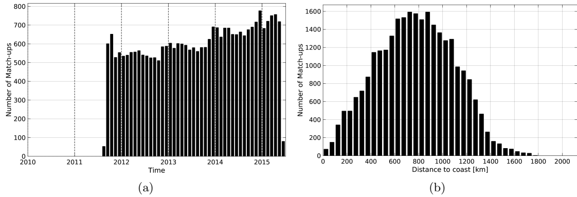
Figure 1: Number of match-ups between Argo and Aquarius-L3-JPL-V4-7DAY-RUNNING SSS as a function of time (a) and as function of the distance to coast (b) over the South Atlantic Ocean Pi-MEP region and for the full satellite product period.
