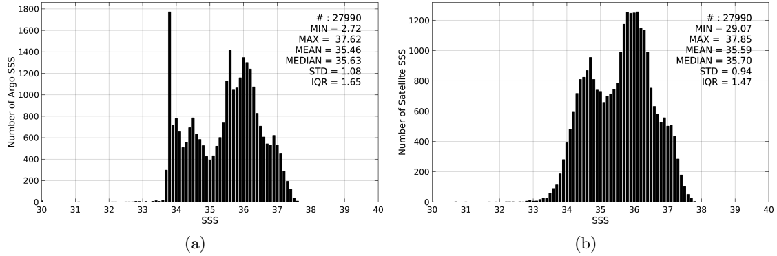
Figure 2: Histograms of SSS from Argo (a) and Aquarius-L3-JPL-V4-7DAY-RUNNING (b) considering all match-up pairs per bins of 0.1 over the South Atlantic Ocean Pi-MEP region and for the full satellite product period.
