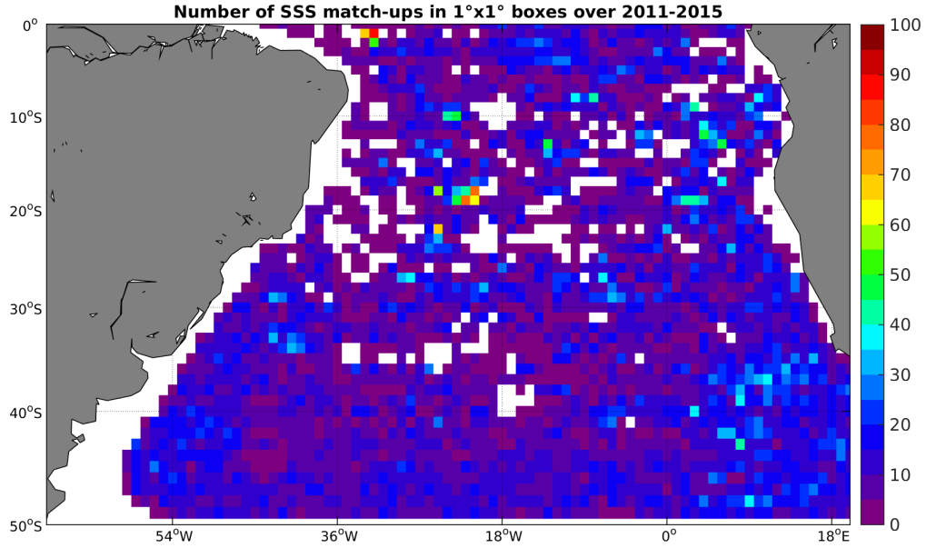
Figure 4: Number of SSS match-ups between Argo SSS and the Aquarius-L3-JPL-V4-7DAY-RUNNING SSS product for the South Atlantic Ocean Pi-MEP region over 1^\circ \times 1^\circ boxes and for the full satellite product period.
