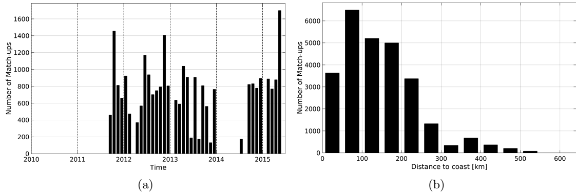
Figure 1: Number of match-ups between TSG-LEGOS-DM and Aquarius-L3-JPL-V4-MONTHLY SSS as a function of time (a) and as function of the distance to coast (b) over the South Atlantic Ocean Pi-MEP region and for the full satellite product period.
