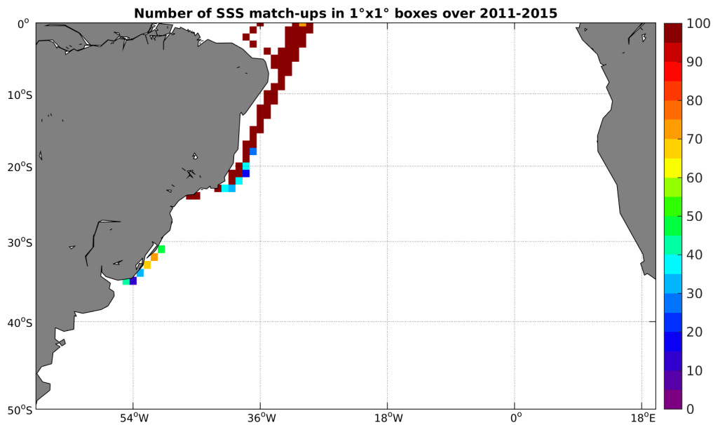
Figure 4: Number of SSS match-ups between TSG-LEGOS-DM SSS and the Aquarius-L3-JPL-V4-MONTHLY SSS product for the South Atlantic Ocean Pi-MEP region over 1^\circ \times 1^\circ boxes and for the full satellite product period.
