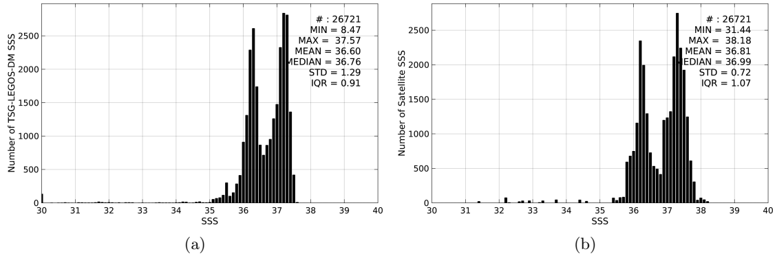
Figure 2: Histograms of SSS from TSG-LEGOS-DM (a) and Aquarius-L3-JPL-V4-MONTHLY (b) considering all match-up pairs per bins of 0.1 over the South Atlantic Ocean Pi-MEP region and for the full satellite product period.
