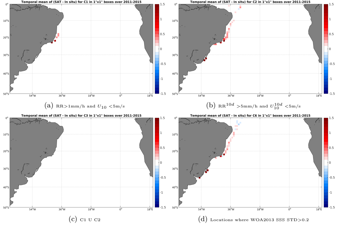
Figure 12: Temporal mean gridded over spatial boxes of size 1^\circ \times 1^\circ of \Delta SSS (Aquarius-L3-JPL-V4-MONTHLY - TSG-LEGOS-DM) for 4 different subdatasets corresponding to: RR > 1\text{mm/h} and U_{10} < 5\text{m/s} (a), RR^{10d} > 5\text{mm/h} and U_{10}^{10d} < 5\text{m/s} (b), C1 U C2 (c), Locations where WOA2013 SSS STD > 0.2 (d).
