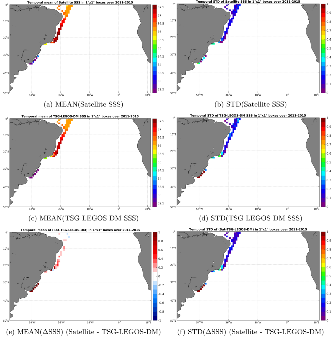
Figure 6: Temporal mean (left) and STD (right) of SSS from Aquarius-L3-JPL-V4-MONTHLY (top), TSG-LEGOS-DM (middle), and of \Delta SSS (Satellite - TSG-LEGOS-DM). Only match-up pairs are used to generate these maps.
