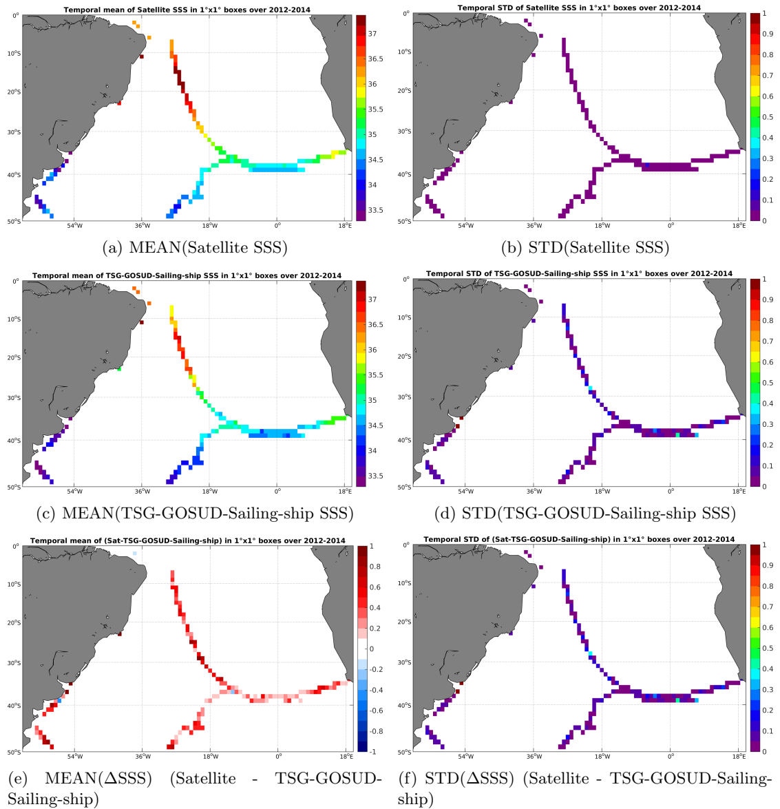
Figure 6: Temporal mean (left) and STD (right) of SSS from Aquarius-L3-JPL-V4-MONTHLY (top), TSG-GOSUD-Sailing-ship (middle), and of \Delta SSS (Satellite - TSG-GOSUD-Sailing-ship). Only match-up pairs are used to generate these maps.
