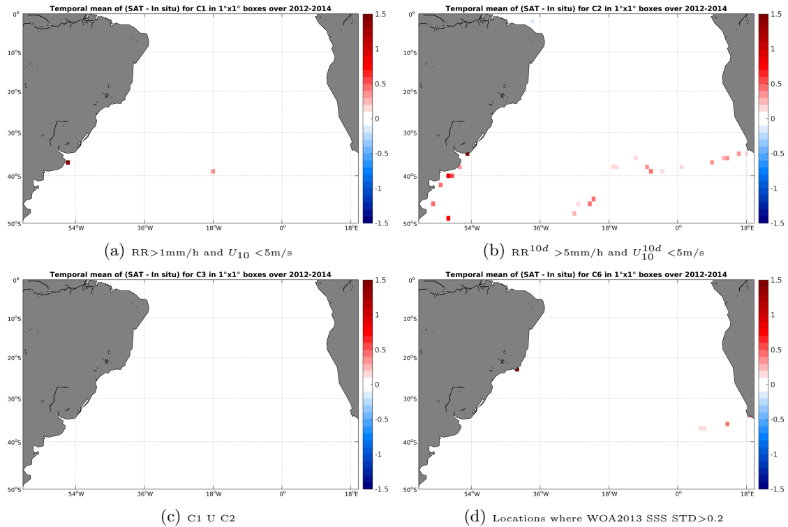
Figure 12: Temporal mean gridded over spatial boxes of size 1^\circ \times 1^\circ of \Delta SSS (Aquarius-L3-JPL-V4-MONTHLY - TSG-GOSUD-Sailing-ship) for 4 different subdatasets corresponding to: RR > 1mm/h and U_{10} < 5\text{m/s} (a), RR^{10d} > 5\text{mm/h} and U_{10}^{10d} < 5\text{m/s} (b), C1 U C2 (c), Locations where WOA2013 SSS STD > 0.2 (d).
