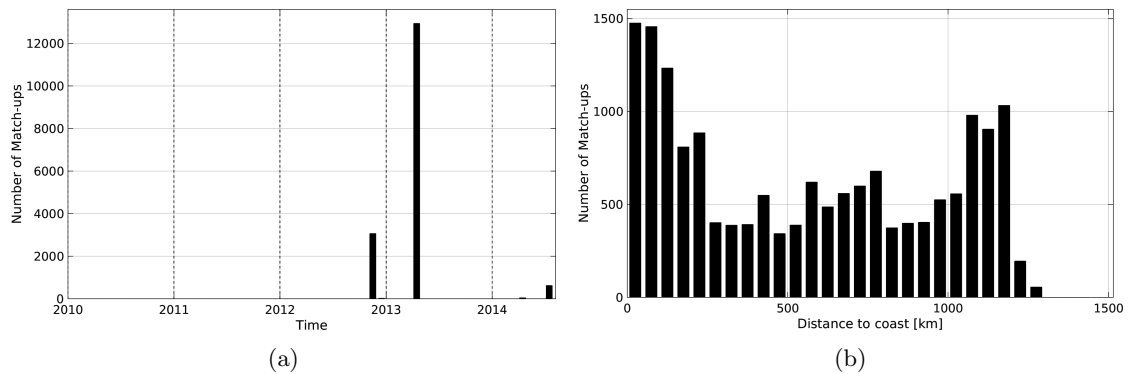
Figure 1: Number of match-ups between TSG-GOSUD-Sailing-ship and Aquarius-L3-JPL-V4-MONTHLY SSS as a function of time (a) and as function of the distance to coast (b) over the South Atlantic Ocean Pi-MEP region and for the full satellite product period.
