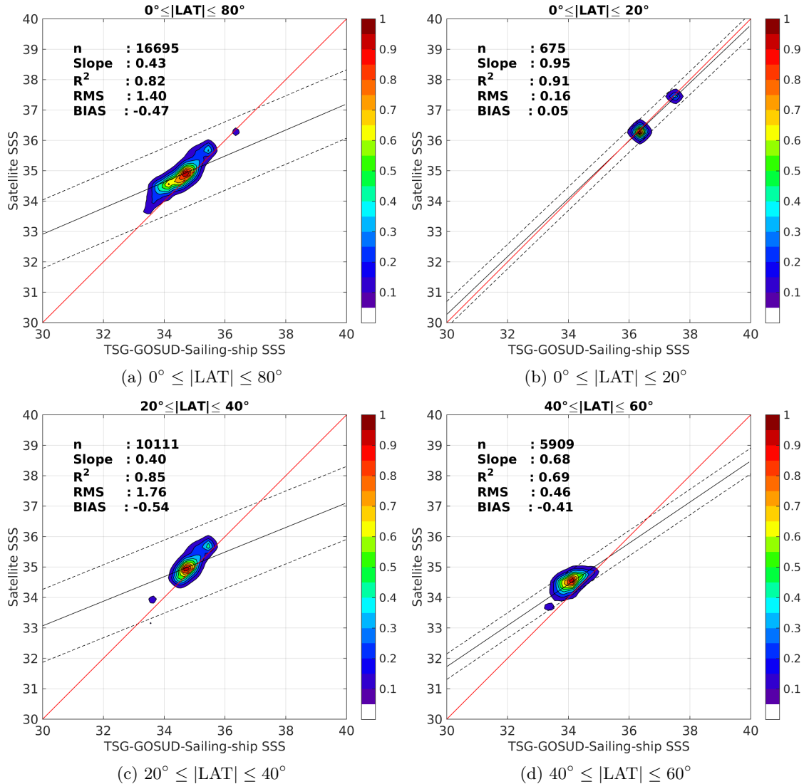
Figure 9: Contour maps of the concentration of Aquarius-L3-JPL-V4-MONTHLY SSS (y-axis) versus TSG-GOSUD-Sailing-ship SSS (x-axis) at match-up pairs for different latitude bands. For each plot, the red line shows x=y . The black thin and dashed lines indicate a linear fit through the data cloud and the \pm 95\% confidence levels, respectively. The number match-up pairs n , the slope and R^2 coefficient of the linear fit, the root mean square (RMS) and the mean bias between satellite and in situ data are indicated for each latitude band in each plots.
