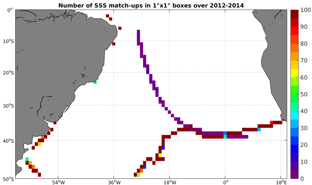
Figure 4: Number of SSS match-ups between TSG-GOSUD-Sailing-ship SSS and the Aquarius-L3-JPL-V4-MONTHLY SSS product for the South Atlantic Ocean Pi-MEP region over 1^\circ \times 1^\circ boxes and for the full satellite product period.
