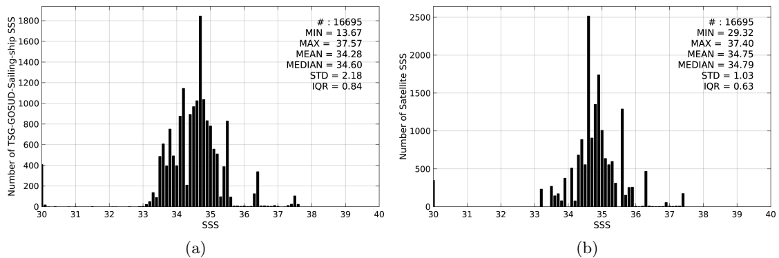
Figure 2: Histograms of SSS from TSG-GOSUD-Sailing-ship (a) and Aquarius-L3-JPL-V4-MONTHLY (b) considering all match-up pairs per bins of 0.1 over the South Atlantic Ocean Pi-MEP region and for the full satellite product period.
