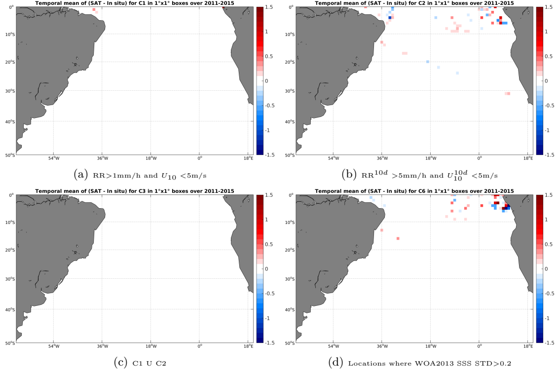
Figure 12: Temporal mean gridded over spatial boxes of size 1^\circ \times 1^\circ of \Delta SSS (Aquarius-L3-JPL-V4-MONTHLY - TSG-GOSUD-Research-vessel) for 4 different subdatasets corresponding to: RR > 1mm/h and U_{10} < 5 m/s (a), RR^{10d} > 5 mm/h and U_{10}^{10d} < 5 m/s (b), C1 U C2 (c), Locations where WOA2013 SSS STD > 0.2 (d).
