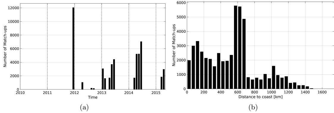
Figure 1: Number of match-ups between TSG-GOSUD-Research-vessel and Aquarius-L3-JPL-V4-MONTHLY SSS as a function of time (a) and as function of the distance to coast (b) over the South Atlantic Ocean Pi-MEP region and for the full satellite product period.
