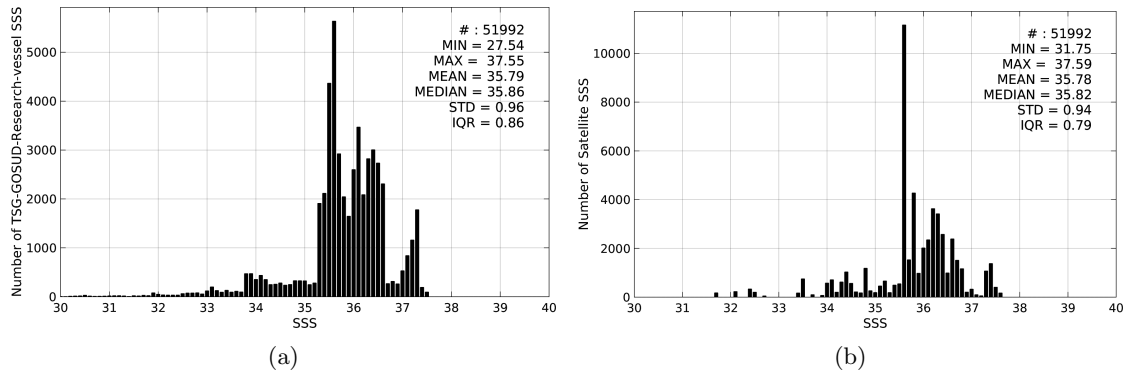
Figure 2: Histograms of SSS from TSG-GOSUD-Research-vessel (a) and Aquarius-L3-JPL-V4-MONTHLY (b) considering all match-up pairs per bins of 0.1 over the South Atlantic Ocean Pi-MEP region and for the full satellite product period.
