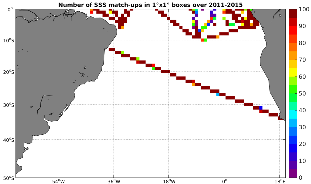
Figure 4: Number of SSS match-ups between TSG-GOSUD-Research-vessel SSS and the Aquarius-L3-JPL-V4-MONTHLY SSS product for the South Atlantic Ocean Pi-MEP region over 1^\circ \times 1^\circ boxes and for the full satellite product period.
