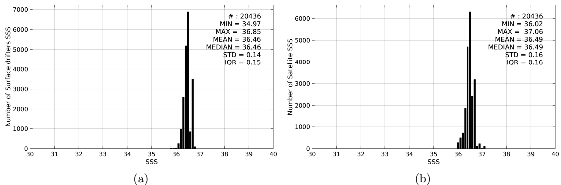
Figure 2: Histograms of SSS from Surface drifters (a) and Aquarius-L3-JPL-V4-MONTHLY (b) considering all match-up pairs per bins of 0.1 over the South Atlantic Ocean Pi-MEP region and for the full satellite product period.
