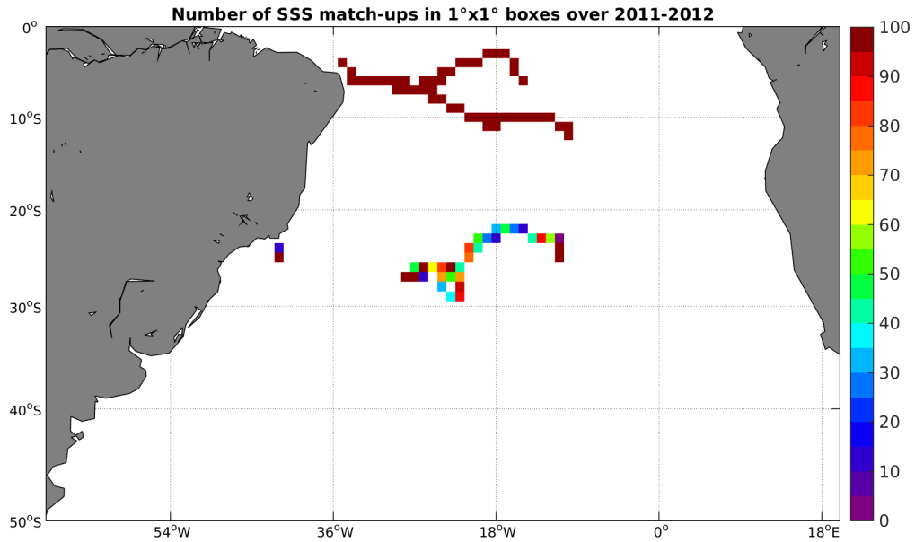
Figure 3: Number of SSS match-ups between Surface drifters SSS and the Aquarius-L3-JPL-V4-MONTHLY SSS product for the South Atlantic Ocean Pi-MEP region over 1°x1° boxes and for the full satellite product period.
