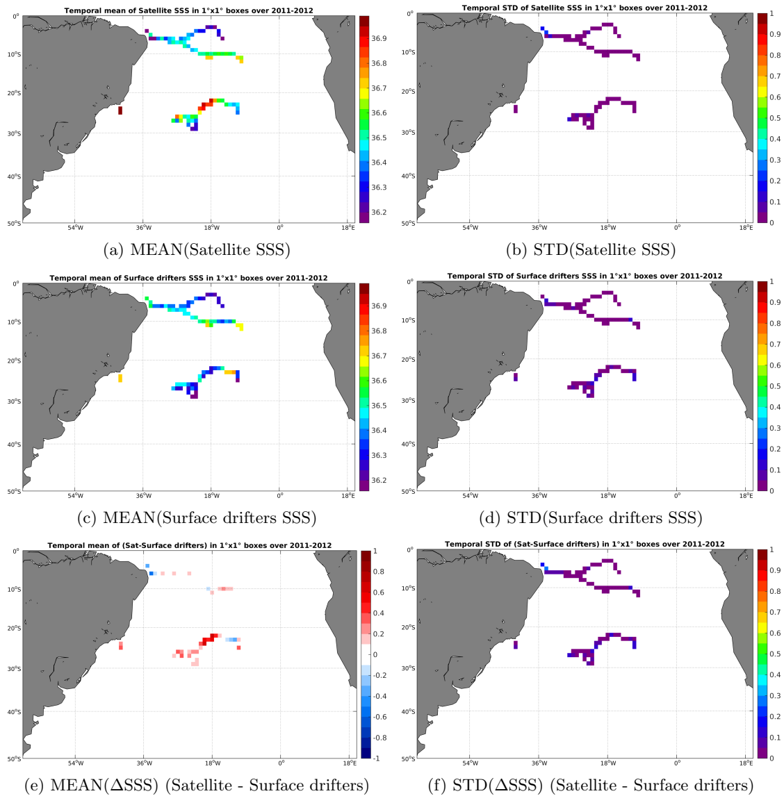
Figure 5: Temporal mean (left) and STD (right) of SSS from Aquarius-L3-JPL-V4-MONTHLY (top), Surface drifters (middle), and of \Delta SSS (Satellite - Surface drifters). Only match-up pairs are used to generate these maps.
