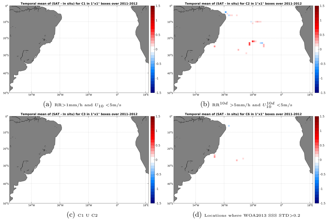
Figure 11: Temporal mean gridded over spatial boxes of size 1^\circ \times 1^\circ of \Delta SSS (Aquarius-L3-JPL-V4-MONTHLY - Surface drifters) for 4 different subdatasets corresponding to:RR>1mm/h and U_{10} < 5m/s (a), RR^{10d} > 5mm/h and U_{10}^{10d} < 5m/s (b), C1 U C2 (c),Locations where WOA2013 SSS STD>0.2 (d).
