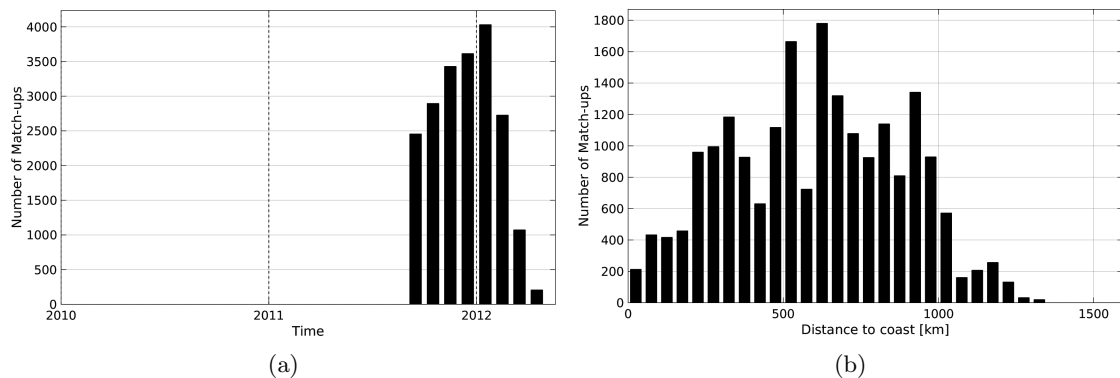
Figure 1: Number of match-ups between Surface drifters and Aquarius-L3-JPL-V4-MONTHLY SSS as a function of time (a) and as function of the distance to coast (b) over the South Atlantic Ocean Pi-MEP region and for the full satellite product period.
