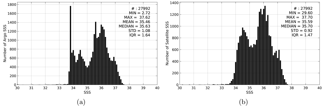
Figure 2: Histograms of SSS from Argo (a) and Aquarius-L3-JPL-V4-MONTHLY (b) considering all match-up pairs per bins of 0.1 over the South Atlantic Ocean Pi-MEP region and for the full satellite product period.
