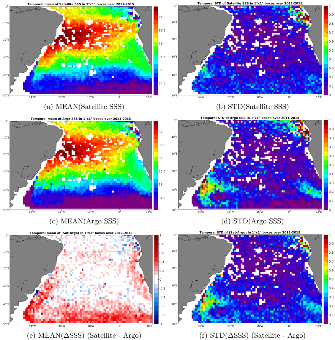
Figure 6: Temporal mean (left) and STD (right) of SSS from Aquarius-L3-JPL-V4-MONTHLY (top), Argo (middle), and of \Delta SSS (Satellite - Argo). Only match-up pairs are used to generate these maps.
