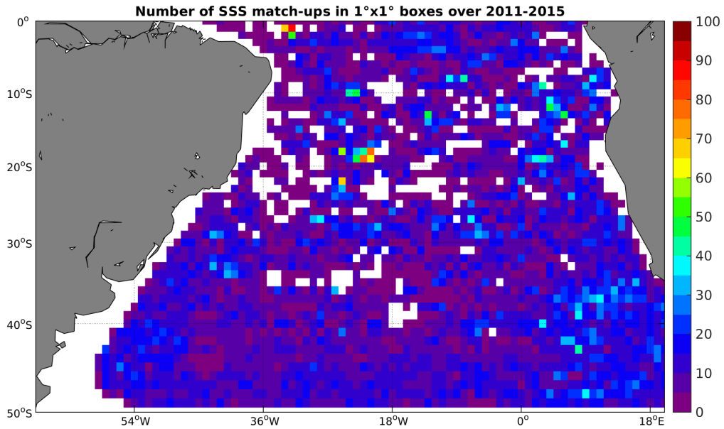
Figure 4: Number of SSS match-ups between Argo SSS and the Aquarius-L3-JPL-V4-MONTHLY SSS product for the South Atlantic Ocean Pi-MEP region over 1^\circ \times 1^\circ boxes and for the full satellite product period.
