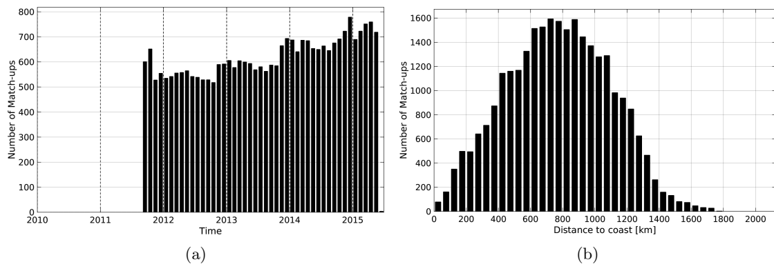
Figure 1: Number of match-ups between Argo and Aquarius-L3-JPL-V4-MONTHLY SSS as a function of time (a) and as function of the distance to coast (b) over the South Atlantic Ocean Pi-MEP region and for the full satellite product period.
