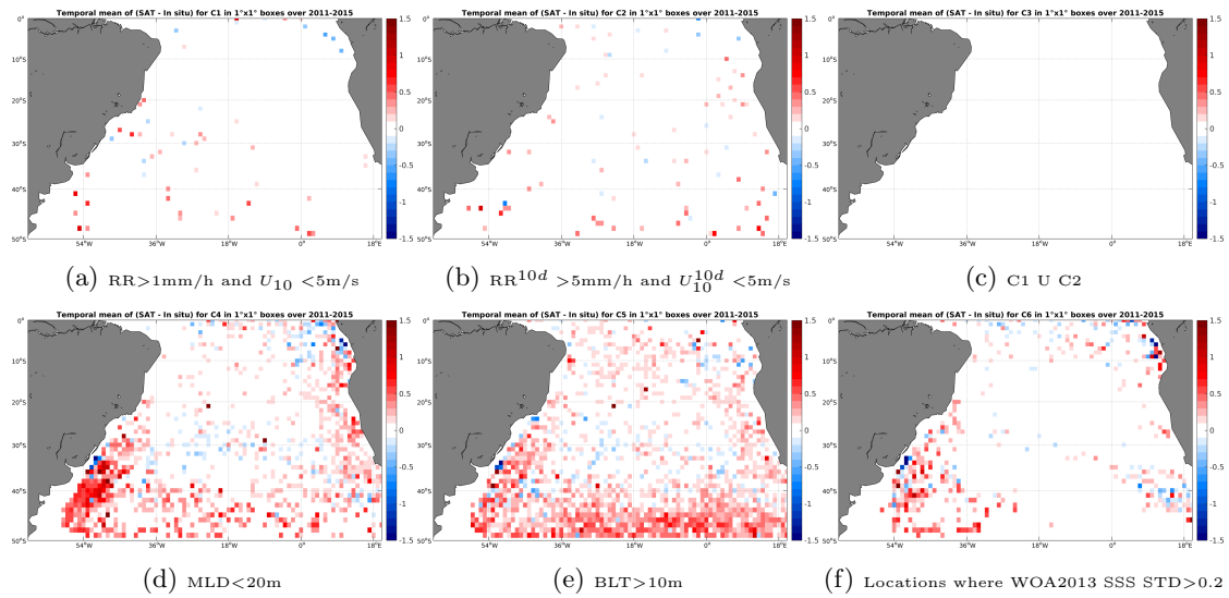
Figure 12: Temporal mean gridded over spatial boxes of size 1^\circ \times 1^\circ of \Delta SSS (Aquarius-L3-JPL-V4-MONTHLY - Argo) for 6 different subdatasets corresponding to: RR > 1\text{mm/h} and U_{10} < 5\text{m/s} (a), RR^{10d} > 5\text{mm/h} and U_{10}^{10d} < 5\text{m/s} (b), C1 U C2 (c), MLD < 20\text{m} (d), BLT > 10\text{m} (e), Locations where WOA2013 SSS STD > 0.2 (f).
