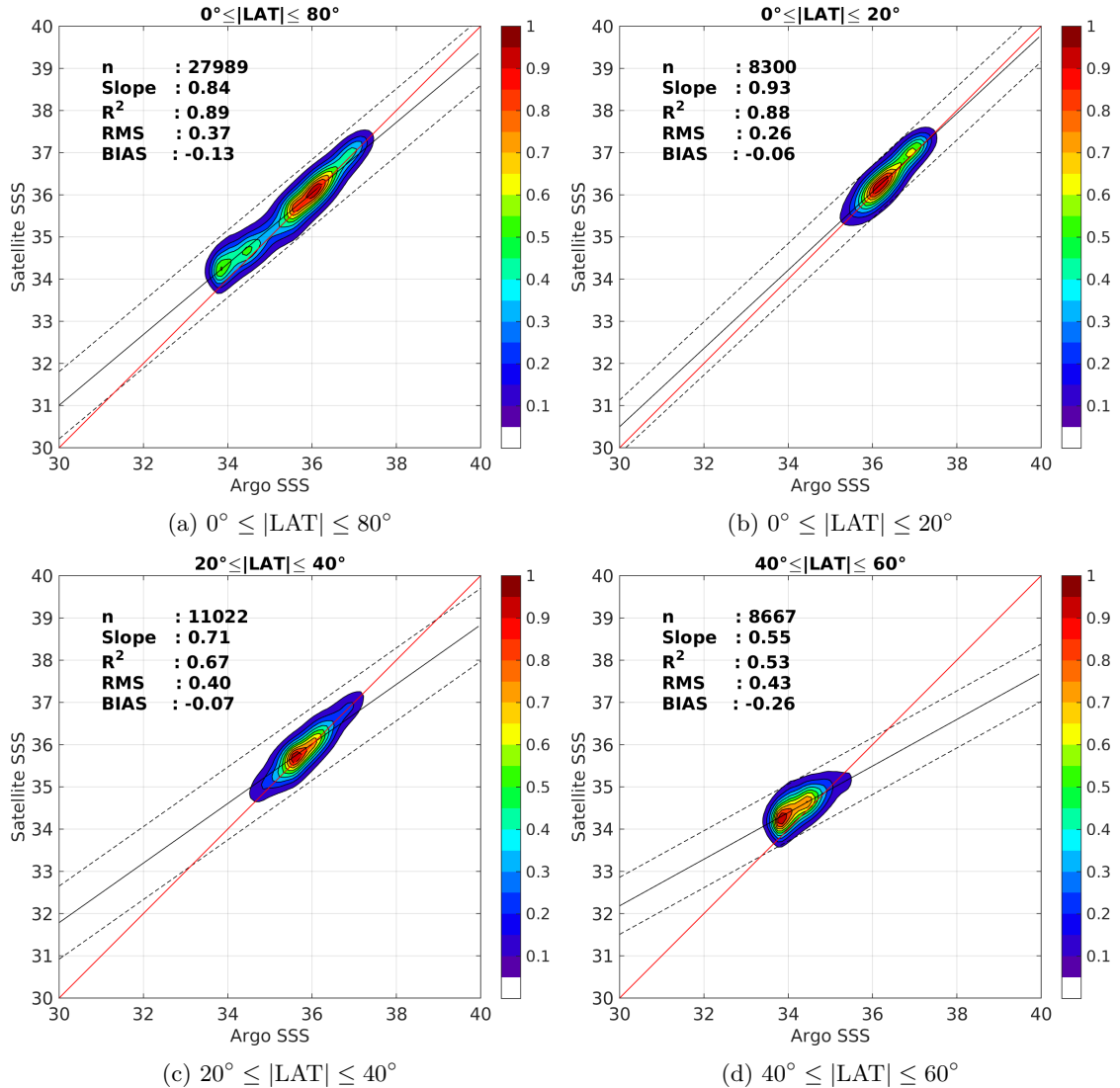
Figure 9: Contour maps of the concentration of Aquarius-L3-JPL-V4-MONTHLY SSS (y-axis) versus Argo SSS (x-axis) at match-up pairs for different latitude bands. For each plot, the red line shows x=y . The black thin and dashed lines indicate a linear fit through the data cloud and the \pm 95\% confidence levels, respectively. The number match-up pairs n , the slope and R^2 coefficient of the linear fit, the root mean square (RMS) and the mean bias between satellite and in situ data are indicated for each latitude band in each plots.
