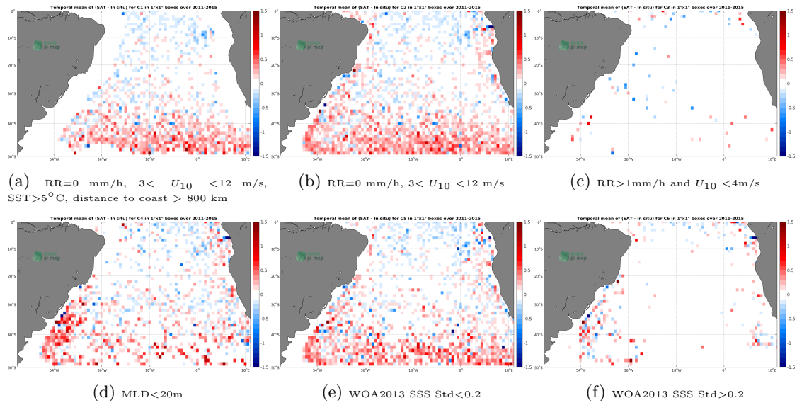
Figure 12: Temporal mean gridded over spatial boxes of size 1^\circ \times 1^\circ of \Delta SSS (Aquarius SSS L2-AVERAGED CAP v5 (JPL) - Argo) for 6 different subdatasets corresponding to:RR=0 mm/h, 3 < U_{10} < 12 m/s, SST >5^\circ\text{C} , distance to coast > 800 km (a), RR=0 mm/h, 3 < U_{10} < 12 m/s (b), RR >1 mm/h and U_{10} < 4 m/s (c),MLD <20 m (d),WOA2013 SSS Std <0.2 (e),WOA2013 SSS Std >0.2 (f).
