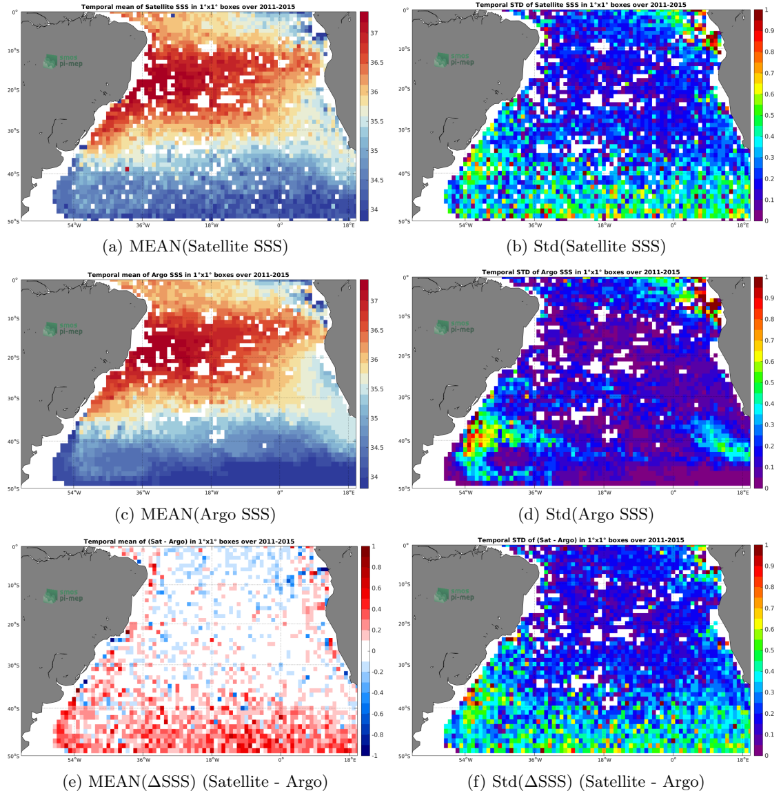
Figure 6: Temporal mean (left) and Std (right) of SSS from Aquarius SSS L2-AVERAGED CAP v5 (JPL) (top), Argo (middle), and of \Delta SSS (Satellite - Argo). Only match-up pairs are used to generate these maps.
