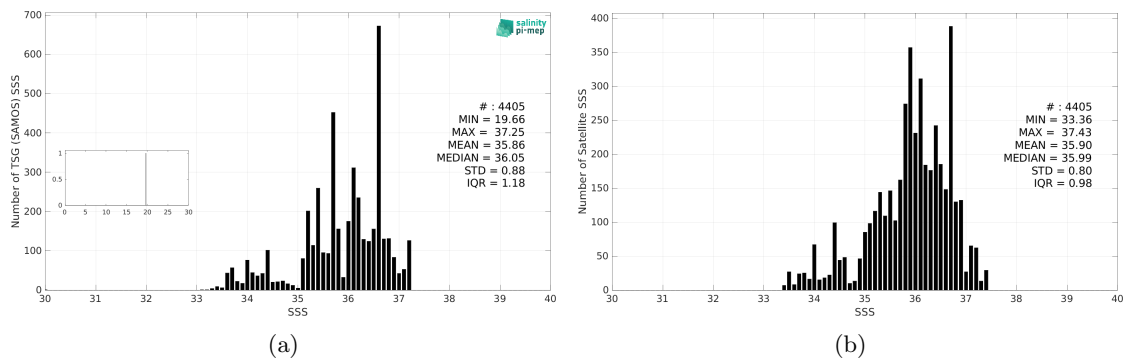
Figure 3: Histograms of SSS from TSG (SAMOS) (a) and Aquarius SSS L2 OR v5 (NASA-GSFC) (b) considering all match-up pairs per bins of 0.1 over the South Atlantic Ocean Pi-MEP region and for the full satellite product period.
