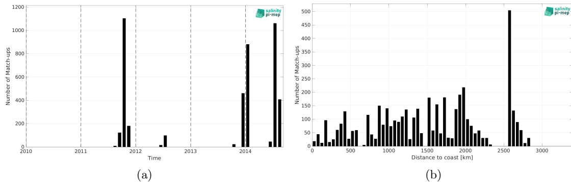
Figure 2: Number of match-ups between TSG (SAMOS) and Aquarius SSS L2 OR v5 (NASA-GSFC) SSS as a function of time (a) and as function of the distance to coast (b) over the South Atlantic Ocean Pi-MEP region and for the full satellite product period.
