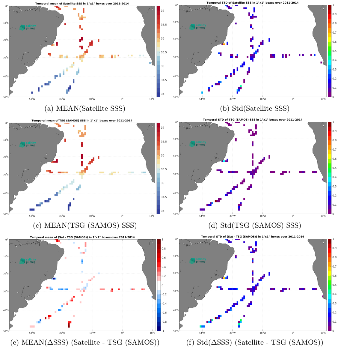
Figure 7: Temporal mean (left) and Std (right) of SSS from Aquarius SSS L2 OR v5 (NASA-GSFC) (top), TSG (SAMOS) (middle), and of \Delta SSS (Satellite - TSG (SAMOS)). Only match-up pairs are used to generate these maps.
