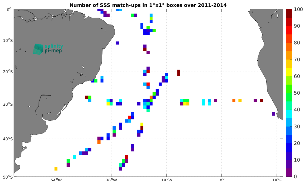
Figure 5: Number of SSS match-ups between TSG (SAMOS) SSS and the Aquarius SSS L2 OR v5 (NASA-GSFC) SSS product for the South Atlantic Ocean Pi-MEP region over 1^\circ \times 1^\circ boxes and for the full satellite product period.
