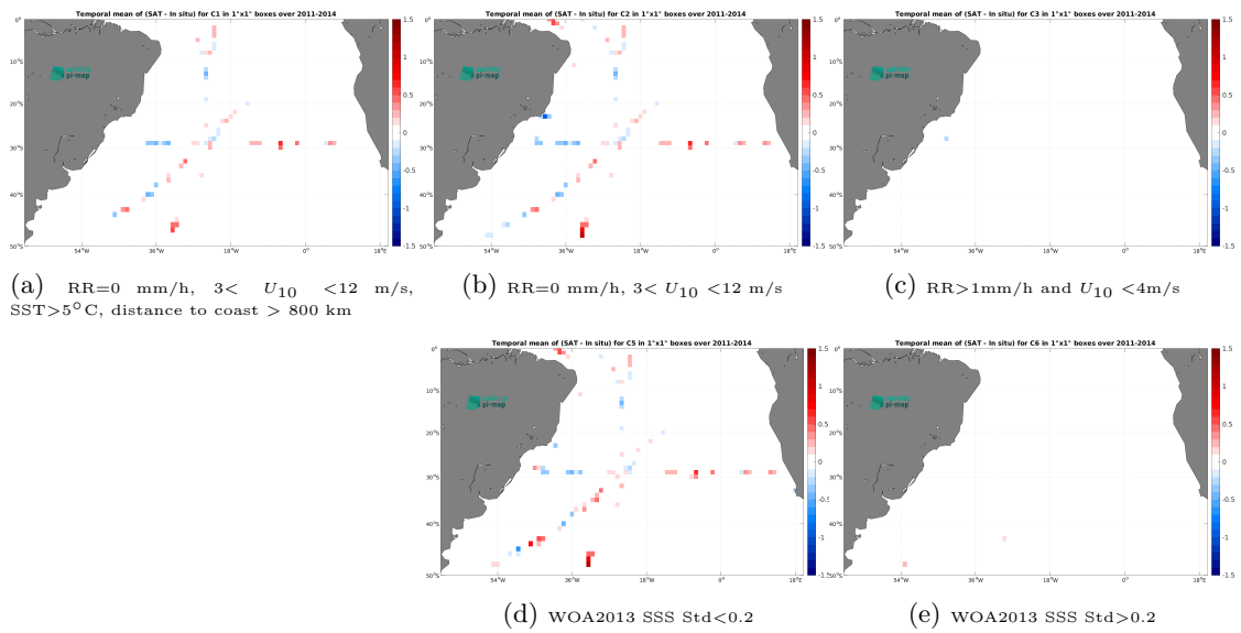
Figure 14: Temporal mean gridded over spatial boxes of size 1^\circ \times 1^\circ of \Delta SSS (Aquarius SSS L2 OR v5 (NASA-GSFC) - TSG (SAMOS)) for 5 different subdatasets corresponding to:RR=0 mm/h, 3 < U_{10} < 12 m/s, SST > 5°C, distance to coast > 800 km (a), RR=0 mm/h, 3 < U_{10} < 12 m/s (b), RR > 1mm/h and U_{10} < 4 m/s (c), WOA2013 SSS Std < 0.2 (d), WOA2013 SSS Std > 0.2 (e).
