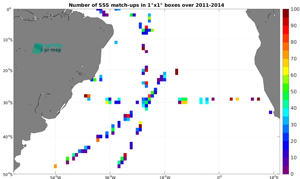
Figure 4: Number of SSS match-ups between TSG (SAMOS) SSS and the Aquarius SSS L2 OR v5 (NASA-GSFC) SSS product for the South Atlantic Ocean Pi-MEP region over 1^\circ \times 1^\circ boxes and for the full satellite product period.
