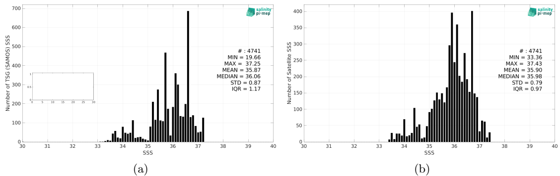
Figure 2: Histograms of SSS from TSG (SAMOS) (a) and Aquarius SSS L2 OR v5 (NASA-GSFC) (b) considering all match-up pairs per bins of 0.1 over the South Atlantic Ocean Pi-MEP region and for the full satellite product period.
