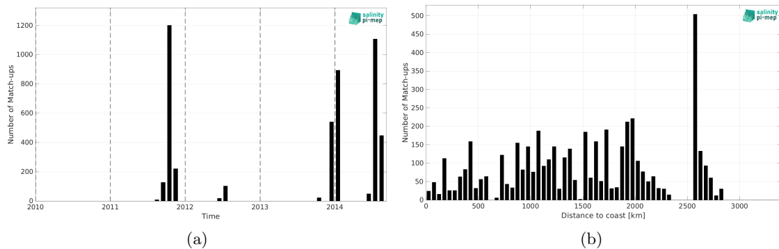
Figure 1: Number of match-ups between TSG (SAMOS) and Aquarius SSS L2 OR v5 (NASA-GSFC) SSS as a function of time (a) and as function of the distance to coast (b) over the South Atlantic Ocean Pi-MEP region and for the full satellite product period.
