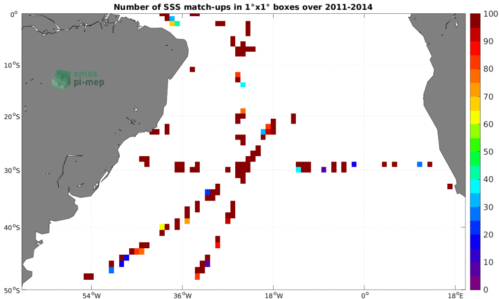
Figure 4: Number of SSS match-ups between TSG (SAMOS) SSS and the Aquarius SSS L2 OR v5 (NASA-GSFC) SSS product for the South Atlantic Ocean Pi-MEP region over 1°x1° boxes and for the full satellite product period.
