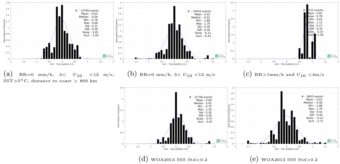
Figure 13: Normalized histogram of \Delta SSS (Aquarius-L2-OR-V5 - TSG-SAMOS) for 5 different subdatasets corresponding to: RR=0 mm/h, 3 < U_{10} < 12 m/s, SST>5°C, distance to coast > 800 km (a), RR=0 mm/h, 3 < U_{10} < 12 m/s (b), RR>1mm/h and U_{10} < 4 m/s (c), WOA2013 SSS Std<0.2 (d), WOA2013 SSS Std>0.2 (e).
