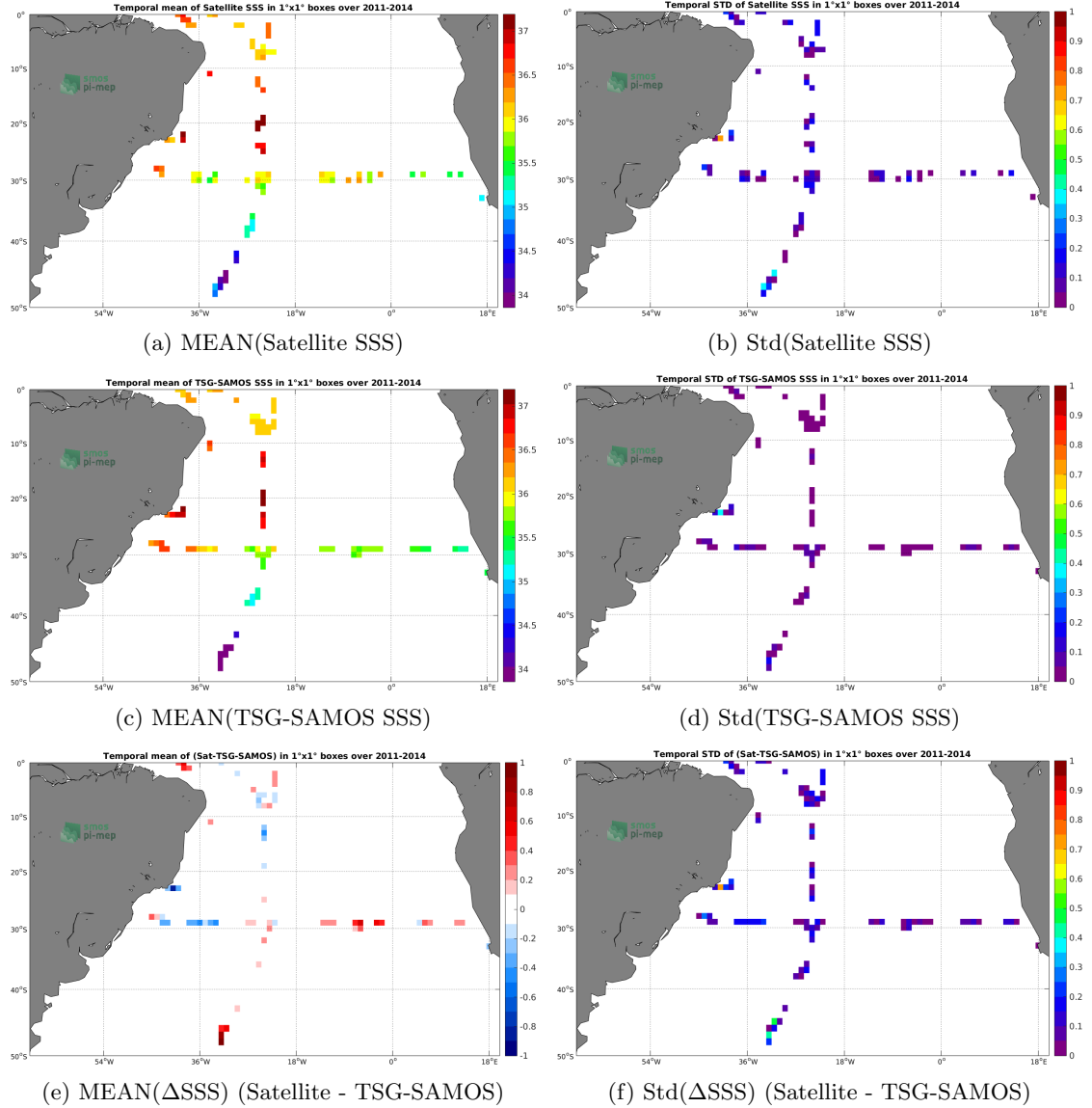
Figure 6: Temporal mean (left) and Std (right) of SSS from Aquarius-L2-OR-V5 (top), TSG-SAMOS (middle), and of \Delta SSS (Satellite - TSG-SAMOS). Only match-up pairs are used to generate these maps.
