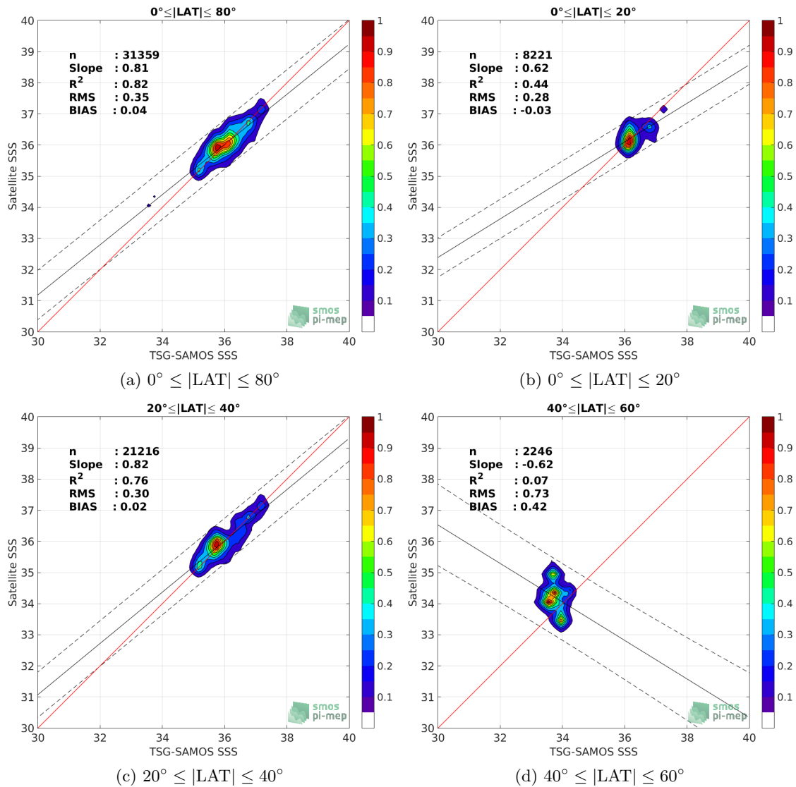
Figure 9: Contour maps of the concentration of Aquarius-L2-OR-V5 SSS (y-axis) versus TSG-SAMOS SSS (x-axis) at match-up pairs for different latitude bands. For each plot, the red line shows x=y . The black thin and dashed lines indicate a linear fit through the data cloud and the \pm 95\% confidence levels, respectively. The number match-up pairs n , the slope and R^2 coefficient of the linear fit, the root mean square (RMS) and the mean bias between satellite and in situ data are indicated for each latitude band in each plots.
