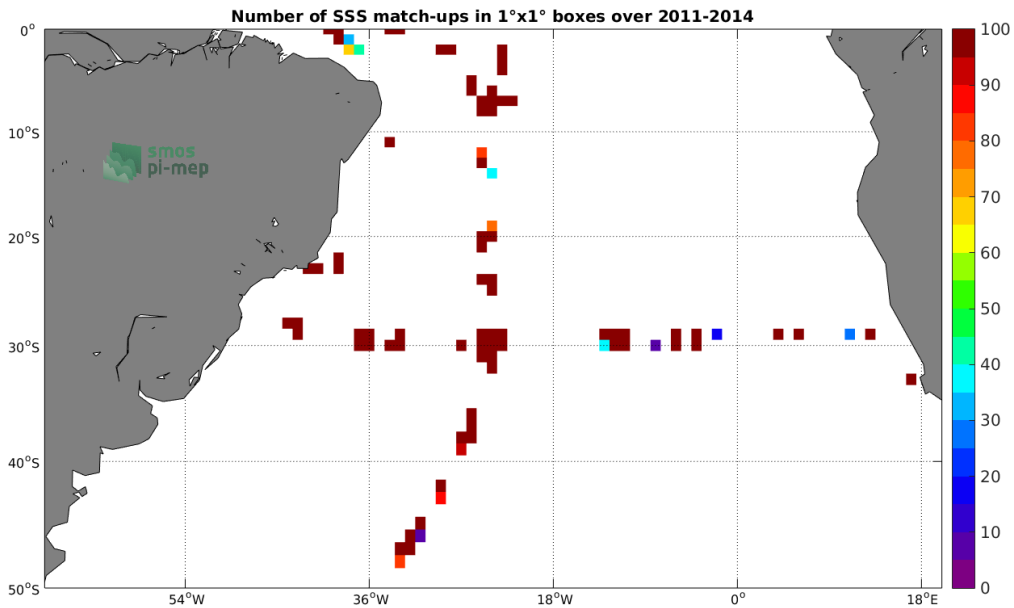
Figure 4: Number of SSS match-ups between TSG-SAMOS SSS and the Aquarius-L2-OR-V5 SSS product for the South Atlantic Ocean Pi-MEP region over 1^{\circ} \times 1^{\circ} boxes and for the full satellite product period.
