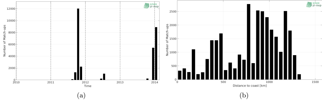
Figure 1: Number of match-ups between TSG-SAMOS and Aquarius-L2-OR-V5 SSS as a function of time (a) and as function of the distance to coast (b) over the South Atlantic Ocean Pi-MEP region and for the full satellite product period.
