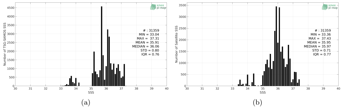
Figure 2: Histograms of SSS from TSG-SAMOS (a) and Aquarius-L2-OR-V5 (b) considering all match-up pairs per bins of 0.1 over the South Atlantic Ocean Pi-MEP region and for the full satellite product period.
