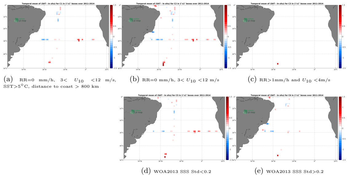
Figure 12: Temporal mean gridded over spatial boxes of size 1^\circ \times 1^\circ of \Delta SSS (Aquarius-L2-OR-V5 - TSG-SAMOS) for 5 different subdatasets corresponding to:RR=0 mm/h, 3 < U_{10} < 12 m/s, SST >5^\circ C, distance to coast > 800 km (a), RR=0 mm/h, 3 < U_{10} < 12 m/s (b), RR >1 mm/h and U_{10} < 4 m/s (c), WOA2013 SSS Std <0.2 (d), WOA2013 SSS Std >0.2 (e).
